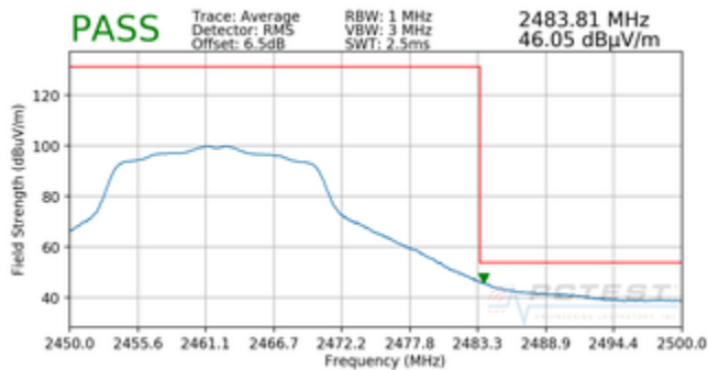
Plot 7-71. Radiated Restricted Upper Band Edge Measurement SISO ANT1 (Average)
