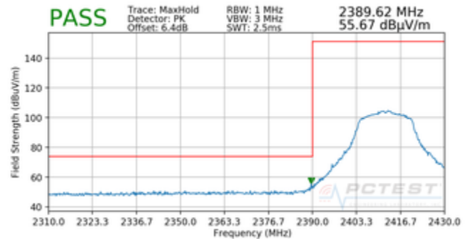
Plot 7-74. Radiated Restricted Lower Band Edge Measurement SISO ANT2 (Peak)
