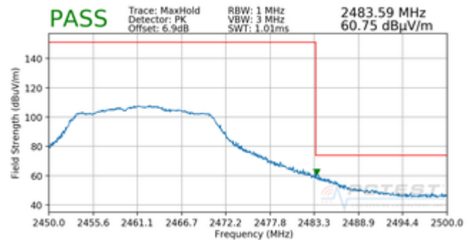
Plot 7-80. Radiated Restricted Upper Band Edge Measurement MIMO (Peak)
