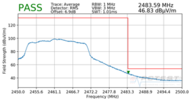
Plot 7-79. Radiated Restricted Upper Band Edge Measurement MIMO (Average)
