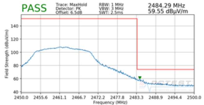
Plot 7-72. Radiated Restricted Upper Band Edge Measurement SISO ANT1 (Peak)
