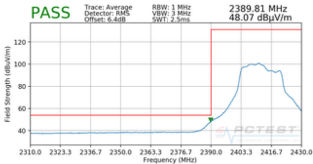
Plot 7-77. Radiated Restricted Lower Band Edge Measurement MIMO (Average)
