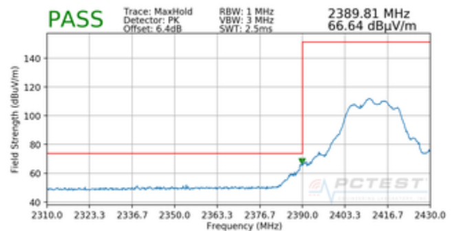
Plot 7-82. Radiated Restricted Lower Band Edge Measurement CDD (Peak)
