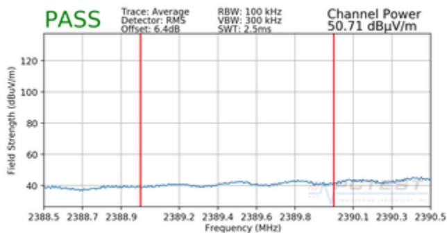
Plot 7-81. Radiated Restricted Lower Band Edge Measurement CDD (Average)
