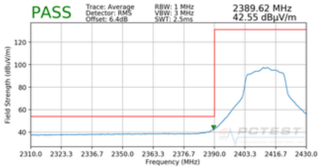
Plot 7-73. Radiated Restricted Lower Band Edge Measurement SISO ANT2 (Average)
