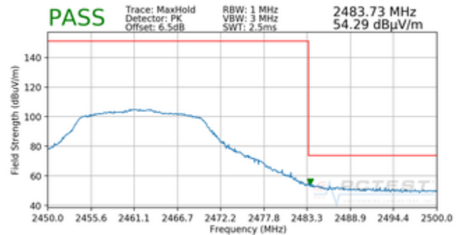
Plot 7-76. Radiated Restricted Upper Band Edge Measurement SISO ANT2 (Peak)
