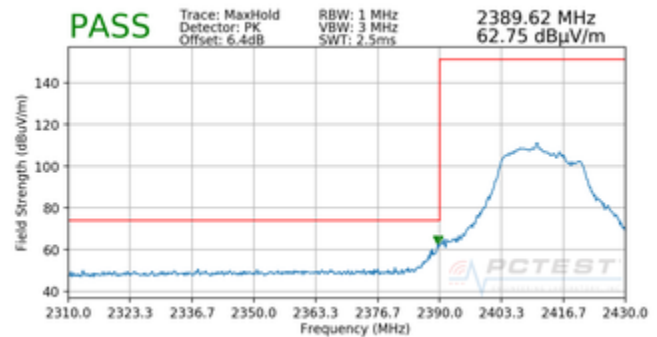
Plot 7-78. Radiated Restricted Lower Band Edge Measurement MIMO (Peak)
