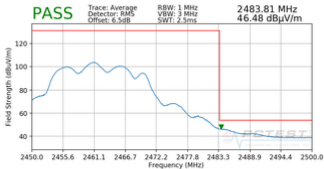
Plot 7-83. Radiated Restricted Upper Band Edge Measurement CDD (Average)
