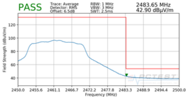
Plot 7-75. Radiated Restricted Upper Band Edge Measurement SISO ANT2 (Average)
