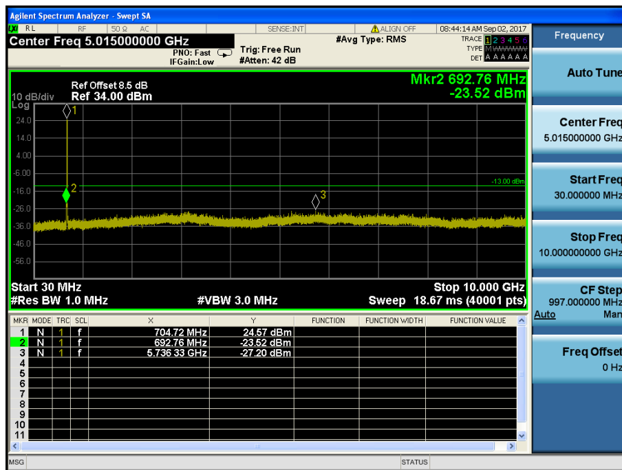
LTE Band 17 / 5MHz / QPSK - RB Size/Offset (25/0) – Low Channel
