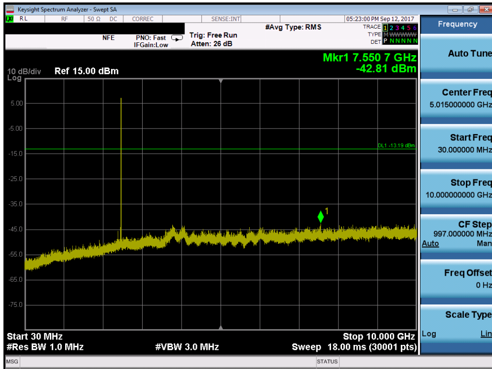
Plot 7-40. Conducted Spurious Plot (Bluetooth, N/AMbps – Ch. 78)
