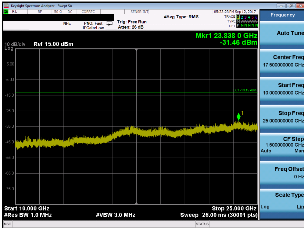
Plot 7-41. Conducted Spurious Plot (Bluetooth, N/AMbps – Ch. 78)
