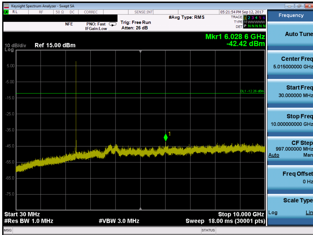
Plot 7-38. Conducted Spurious Plot (Bluetooth, N/AMbps – Ch. 39)
