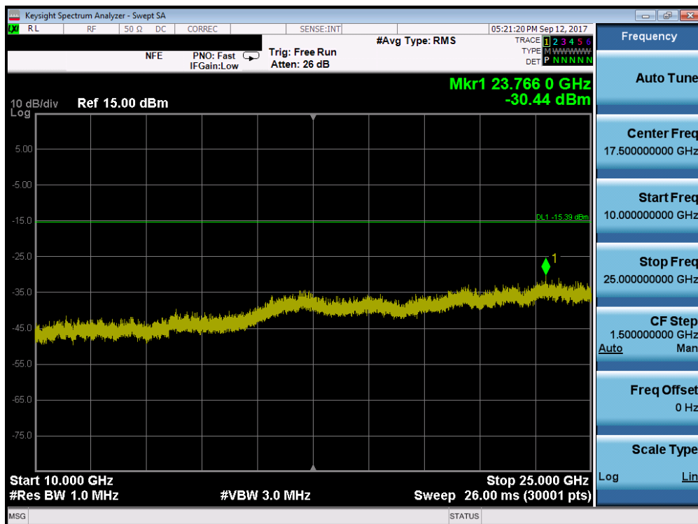
Plot 7-37. Conducted Spurious Plot (Bluetooth, N/AMbps – Ch. 0)
