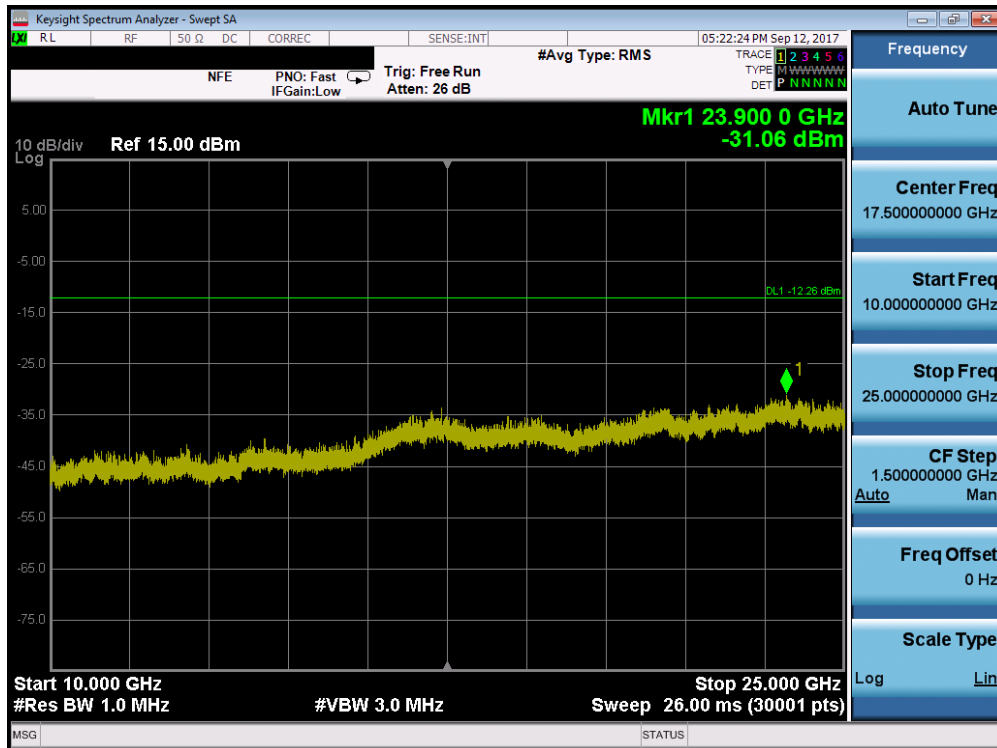
Plot 7-39. Conducted Spurious Plot (Bluetooth, N/AMbps – Ch. 39)
