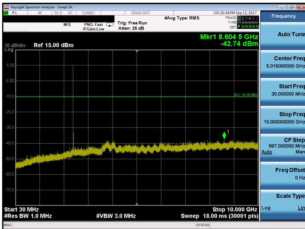
Plot 7-36. Conducted Spurious Plot (Bluetooth, N/AMbps – Ch. 0)
