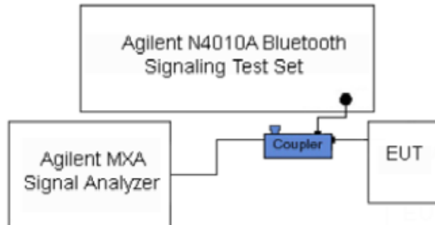
Figure 9-7 Power Measurement Setup
