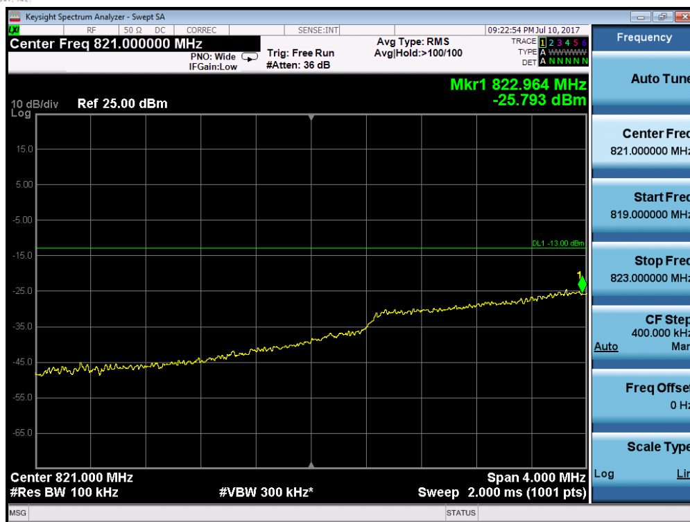
Plot 7-130. Lower Extended Band Edge Plot (Band 5/26 - 3.0MHz QPSK - RB Size 15)
