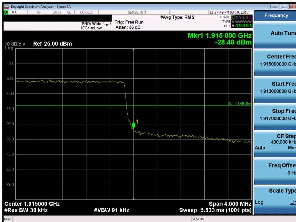
Plot 7-175. Upper Band Edge Plot (Band 25 – 3.0MHz QPSK – RB Size 15)
