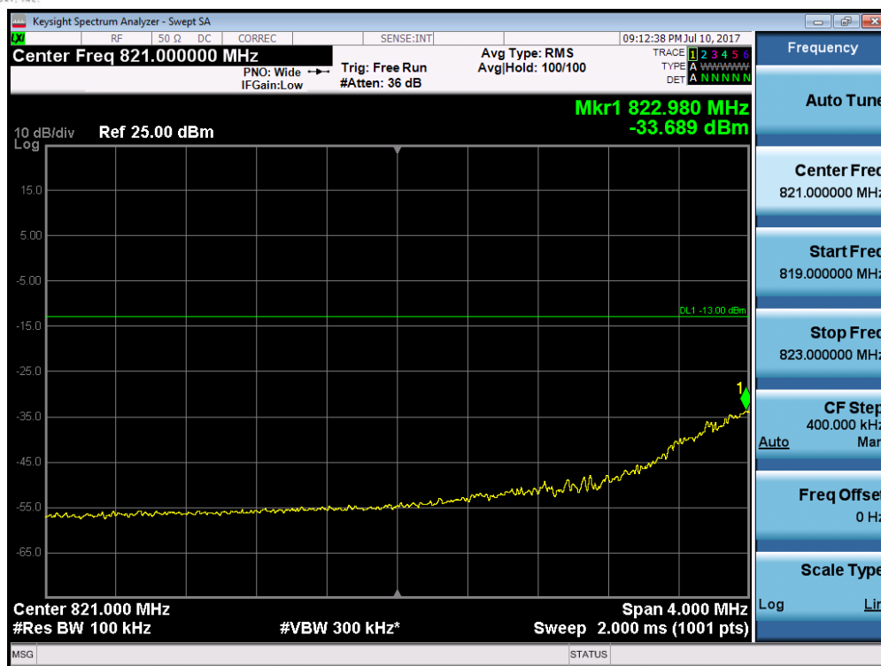
Plot 7-126. Lower Extended Band Edge Plot (Band 5/26 – 1.4MHz QPSK – RB Size 6)
