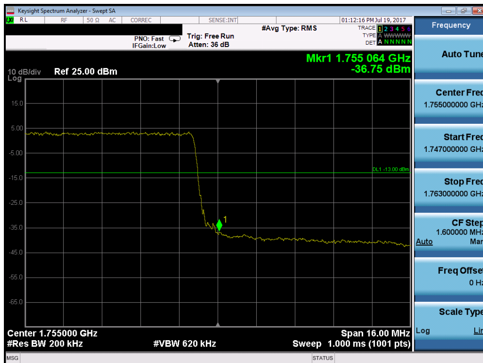
Plot 7-167. Upper Band Edge Plot (Band 4 – 20.0MHz QPSK – RB Size 100)
