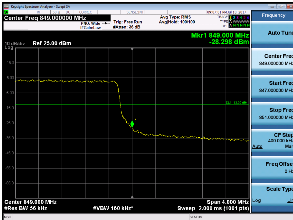
Plot 7-135. Upper Band Edge Plot (Band 5/26 – 5.0MHz QPSK – RB Size 25)
