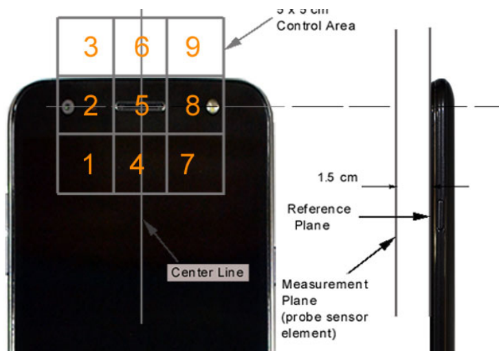
Figure 17-3 5x5 Scan grid above WD
