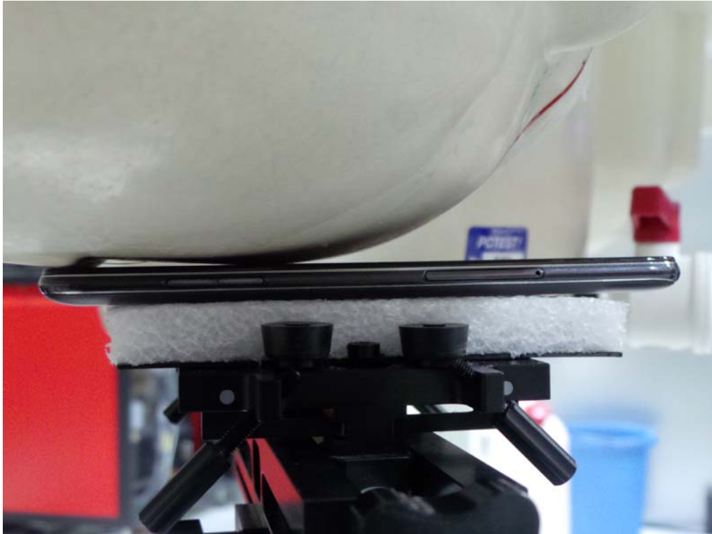
SAR Test Setup Photo 1: Right Cheek
