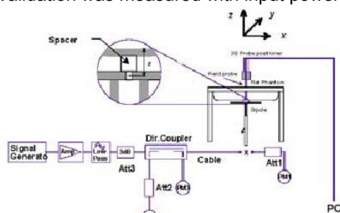
Figure 9.1 Dipole Validation Test Setup
