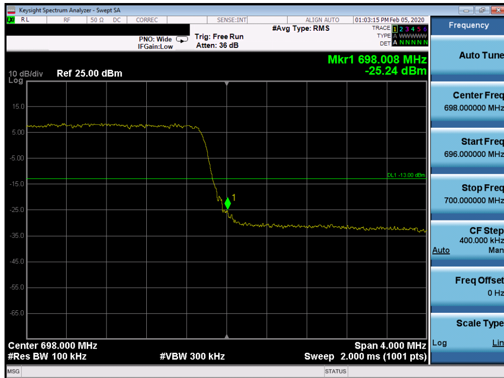
Plot 7-152. Upper Band Edge Plot (Band 71 - 5.0MHz QPSK - Full RB Configuration)
