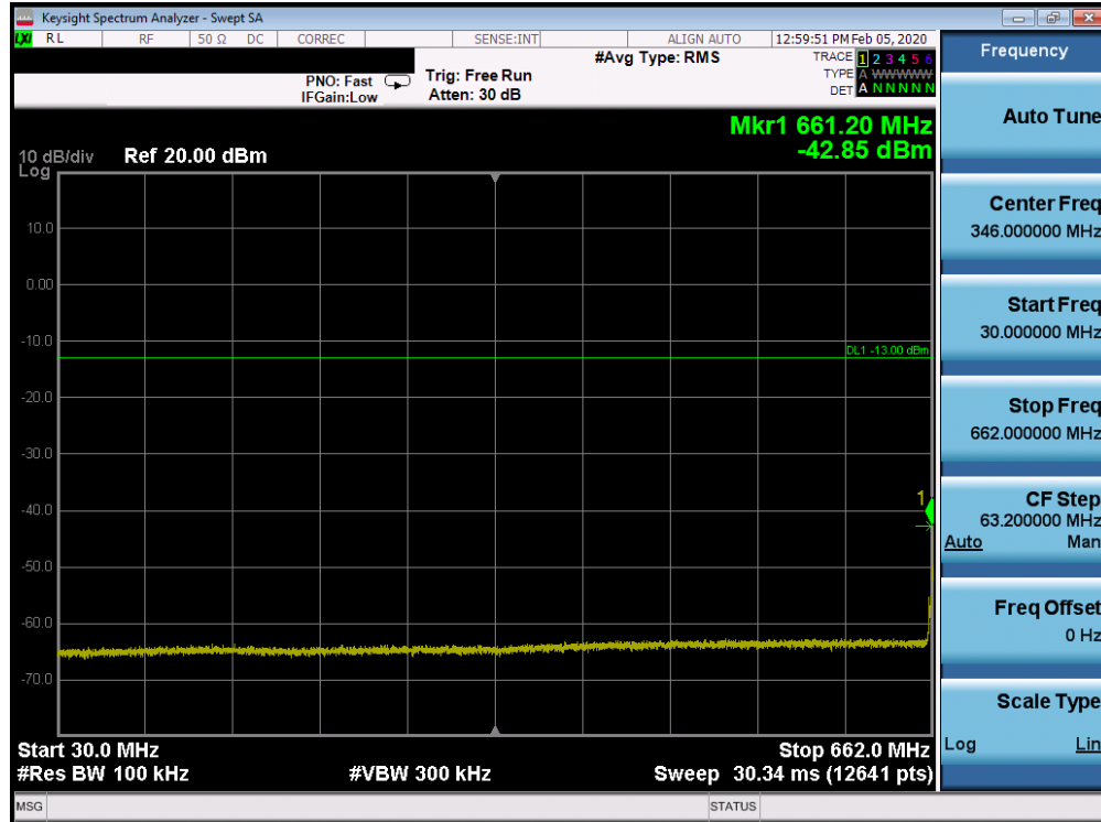
Plot 7-94. Conducted Spurious Plot (Band 71 - 5.0MHz QPSK - RB Size 1, RB Offset 0 - Low Channel)
