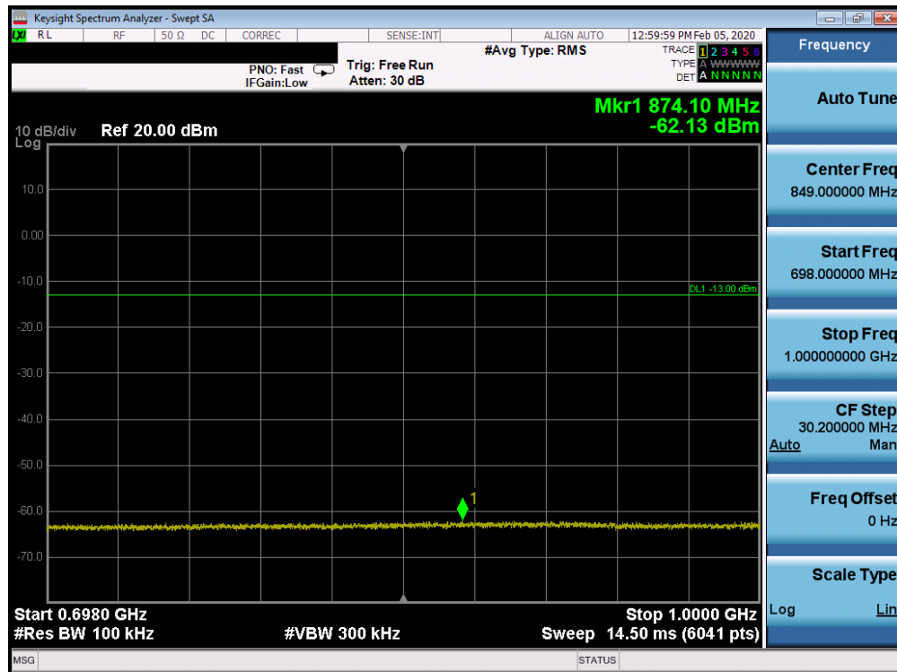
Plot 7-95. Conducted Spurious Plot (Band 71 - 5.0MHz QPSK - RB Size 1, RB Offset 0 - Low Channel)
