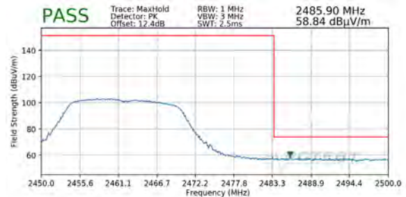
Plot 7-110. Radiated Restricted Upper Band Edge Measurement SISO ANT2 (Peak)
