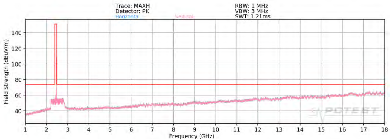
Plot 7-81. Radiated Spurious Plot above 1GHz SISO ANT1 (802.11b – Ch. 11)
