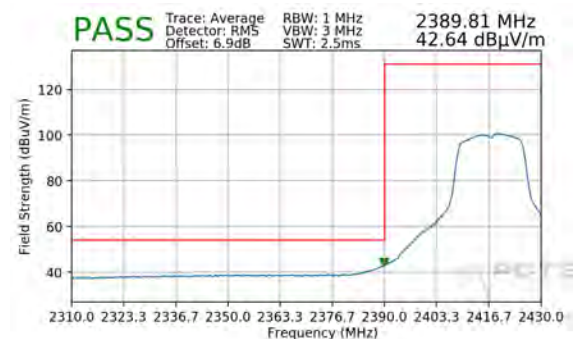
Plot 7-113. Radiated Restricted Lower Band Edge Measurement MIMO (Average)
