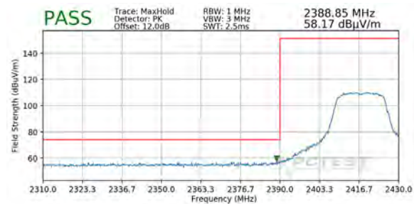
Plot 7-90. Radiated Restricted Lower Band Edge Measurement SISO ANT1 (Peak)
