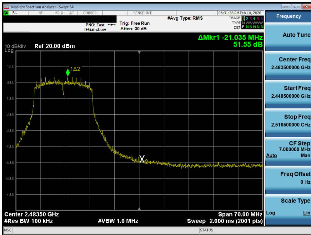
Plot 7-59. Band Edge Plot SISO ANT2 (802.11g – Ch. 11)
