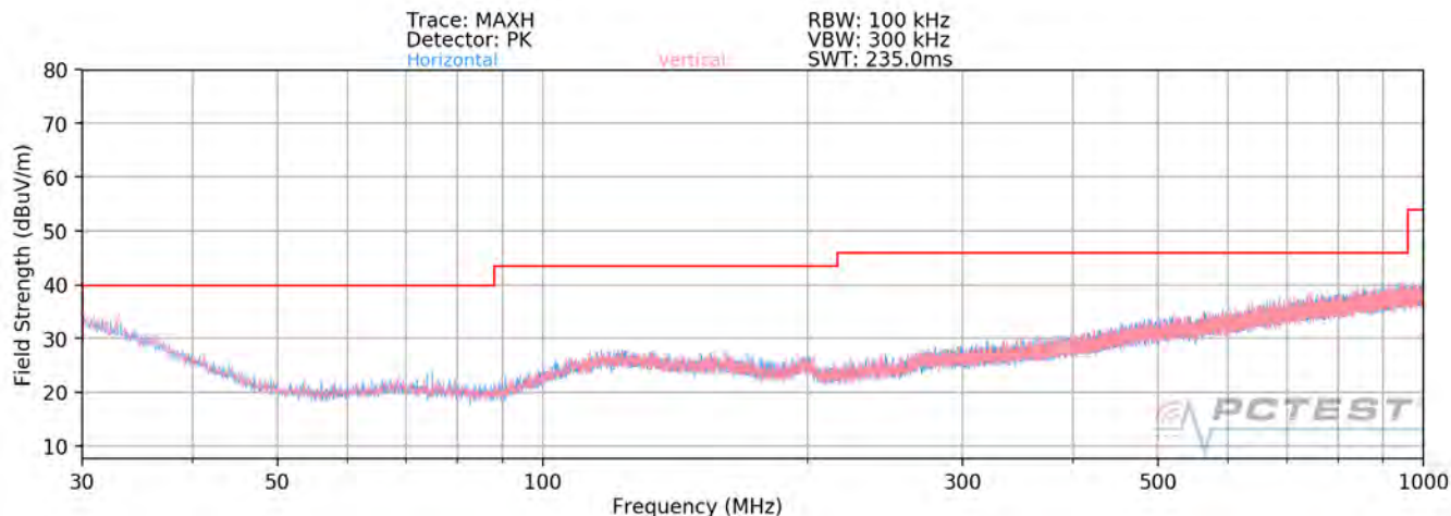
Plot 7-123. Radiated Spurious Plot below 1GHz SISO ANT1
