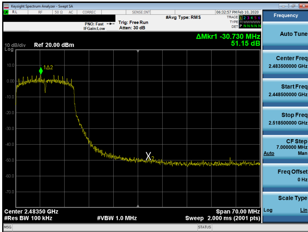
Plot 7-58. Band Edge Plot SISO ANT2 (802.11g – Ch. 10)
