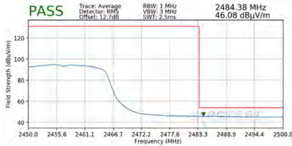
Plot 7-107. Radiated Restricted Upper Band Edge Measurement SISO ANT2 (Average)
