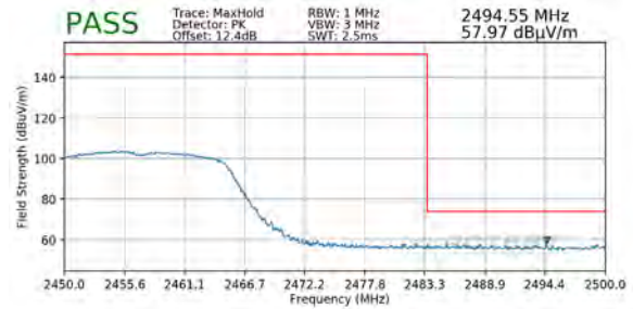
Plot 7-108. Radiated Restricted Upper Band Edge Measurement SISO ANT2 (Peak)
