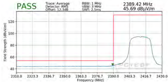
Plot 7-99. Radiated Restricted Lower Band Edge Measurement SISO ANT2 (Average)
