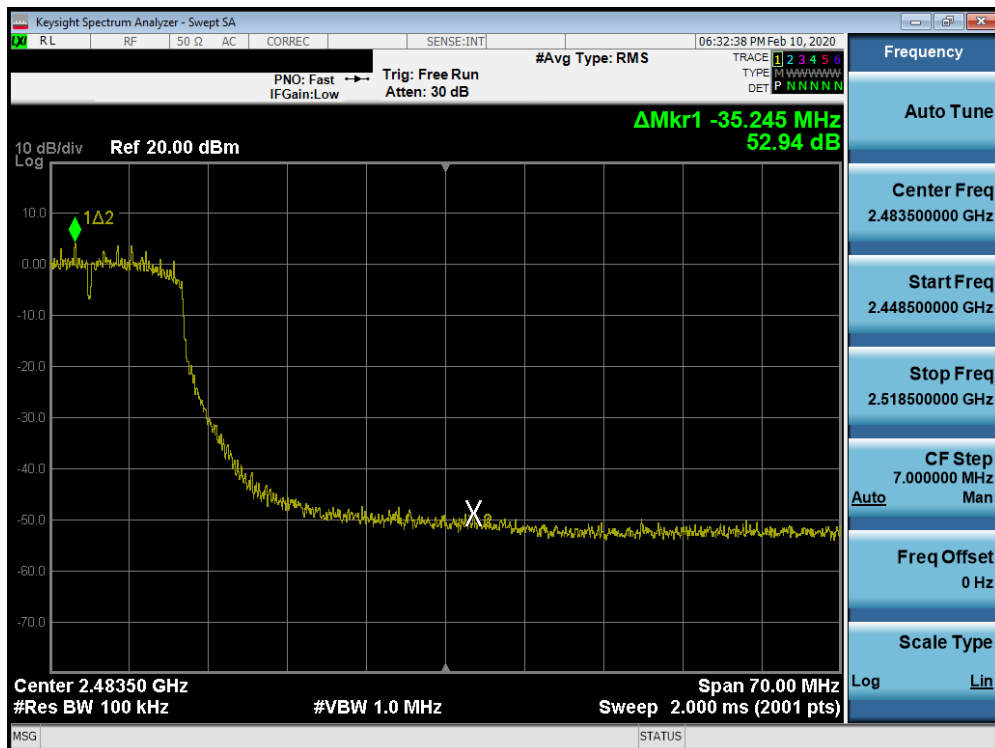
Plot 7-57. Band Edge Plot SISO ANT2 (802.11g - Ch. 9)
