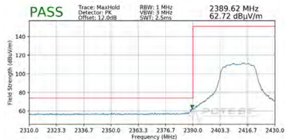
Plot 7-112. Radiated Restricted Lower Band Edge Measurement MIMO (Peak)
