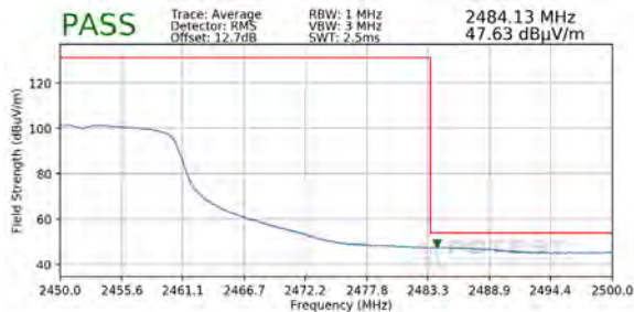
Plot 7-93. Radiated Restricted Upper Band Edge Measurement SISO ANT1 (Average)
