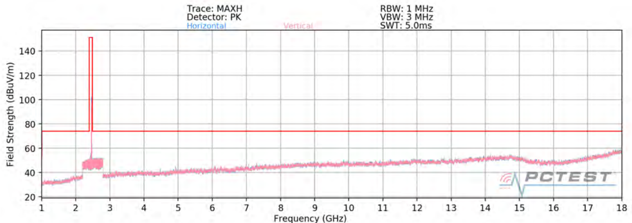
Plot 7-85. Radiated Spurious Plot above 1GHz SISO ANT2 (802.11b – Ch. 11)
