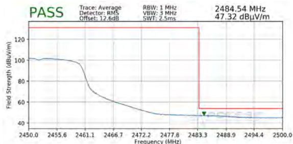
Plot 7-117. Radiated Restricted Upper Band Edge Measurement MIMO (Average)
