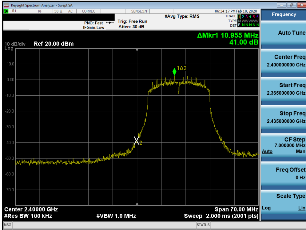
Plot 7-60. Band Edge Plot SISO ANT2 (802.11n (2.4GHz) – Ch. 1)
