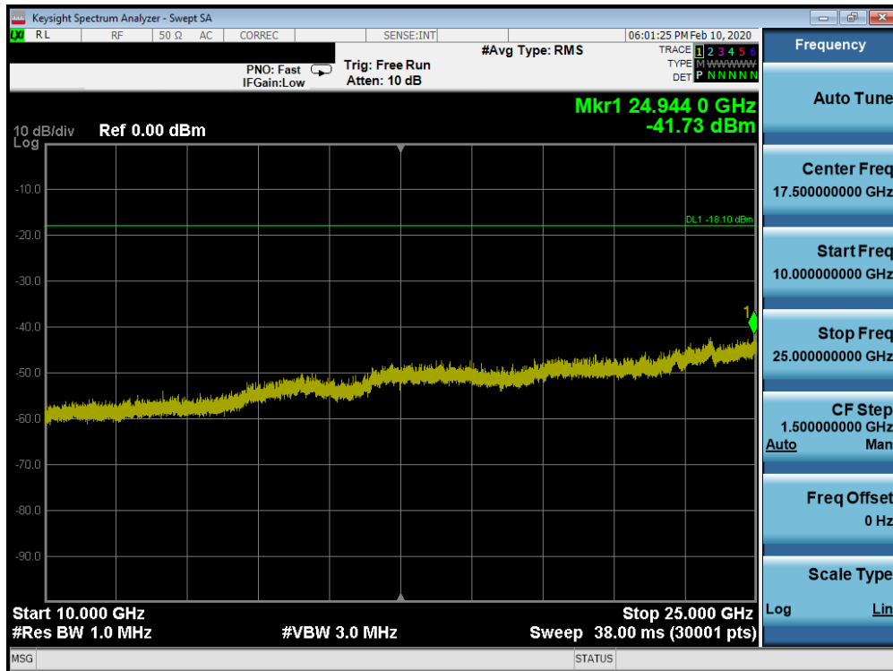
Plot 7-72. Conducted Spurious Plot SISO ANT1 (802.11b – Ch. 11)
