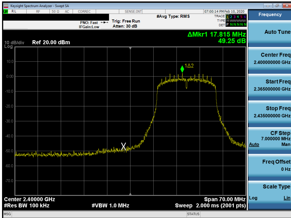
Plot 7-61. Band Edge Plot SISO ANT2 (802.11n (2.4GHz) – Ch. 2)
