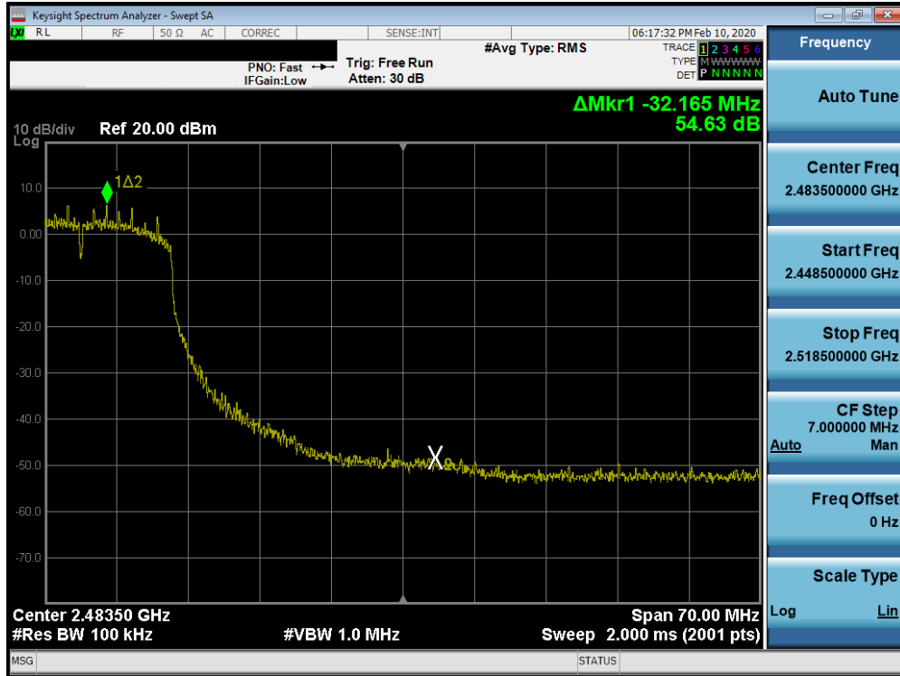
Plot 7-49. Band Edge Plot SISO ANT1 (802.11n (2.4GHz) – Ch. 9)
