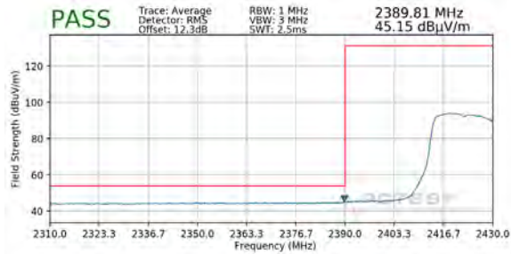
Plot 7-103. Radiated Restricted Lower Band Edge Measurement SISO ANT2 (Average)
