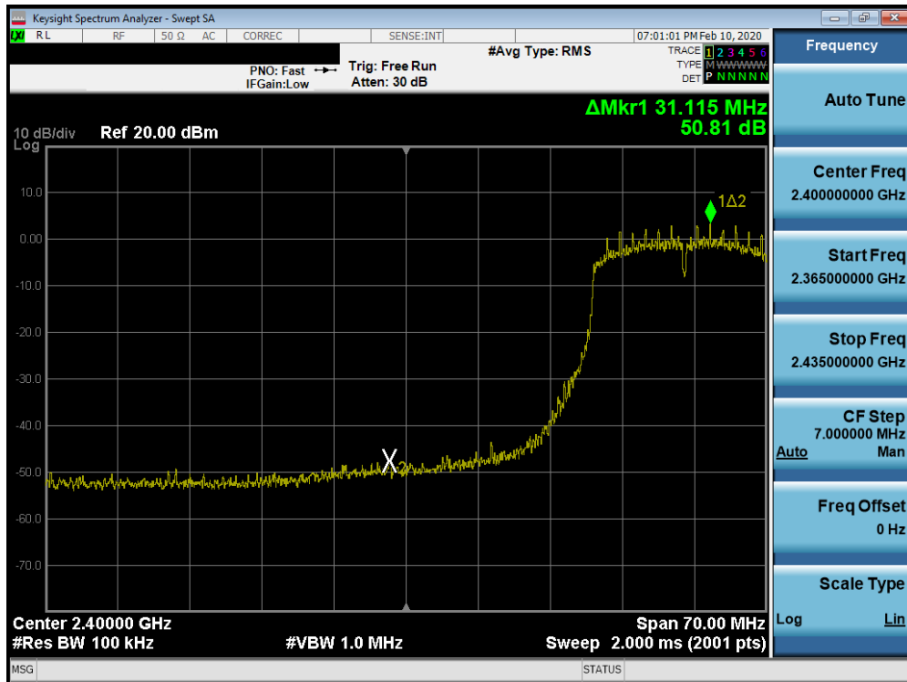
Plot 7-63. Band Edge Plot SISO ANT2 (802.11n (2.4GHz) – Ch. 4)
