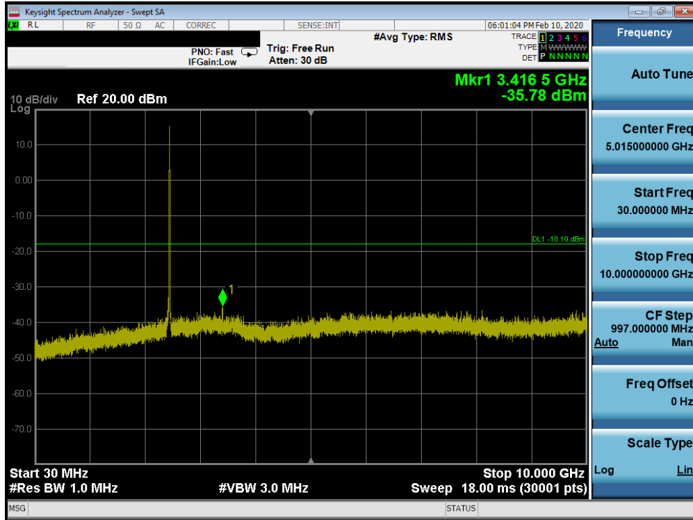
Plot 7-71. Conducted Spurious Plot SISO ANT1 (802.11b – Ch. 11)
