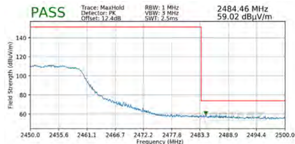
Plot 7-118. Radiated Restricted Upper Band Edge Measurement MIMO (Peak)
