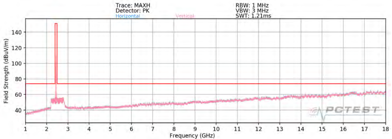
Plot 7-80. Radiated Spurious Plot above 1GHz SISO ANT1 (802.11b – Ch. 6)
