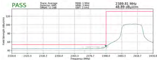
Plot 7-87. Radiated Restricted Lower Band Edge Measurement SISO ANT1 (Average)
