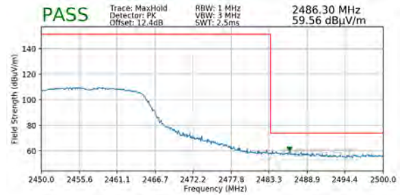
Plot 7-96. Radiated Restricted Upper Band Edge Measurement SISO ANT1 (Peak)
