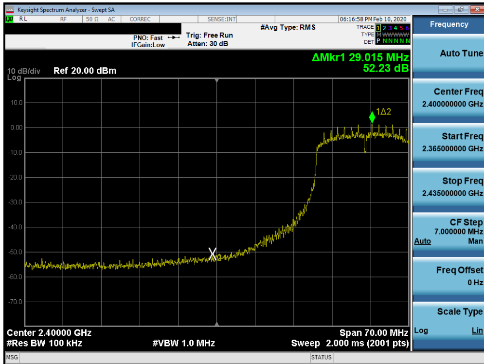
Plot 7-48. Band Edge Plot SISO ANT1 (802.11n (2.4GHz) – Ch. 4)
