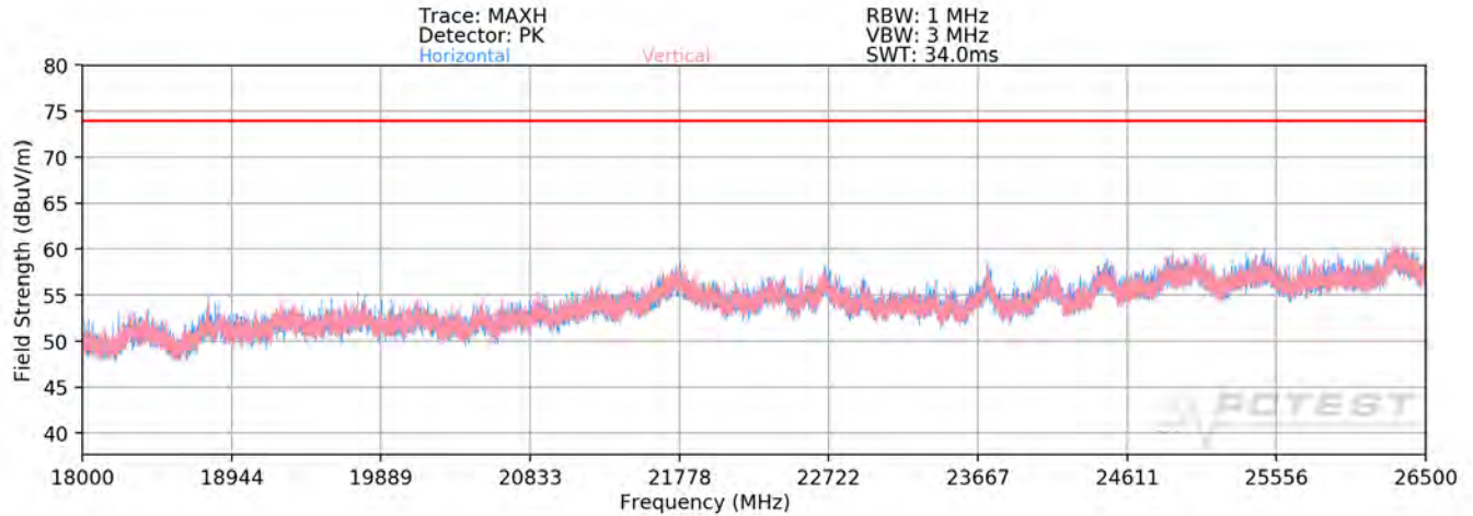
Plot 7-82. Radiated Spurious Plot above 18GHz SISO ANT1
