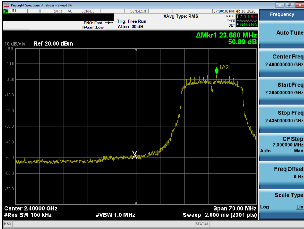
Plot 7-62. Band Edge Plot SISO ANT2 (802.11n (2.4GHz) – Ch. 3)
