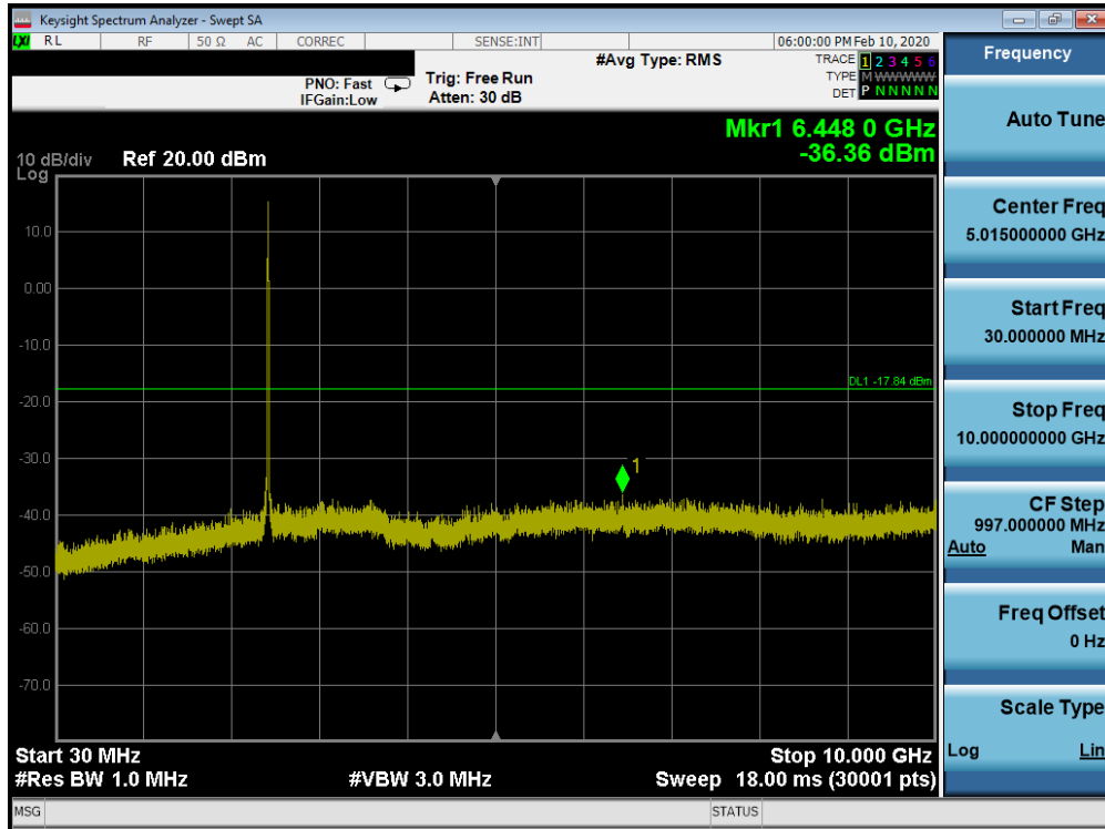
Plot 7-69. Conducted Spurious Plot SISO ANT1 (802.11b – Ch. 6)
