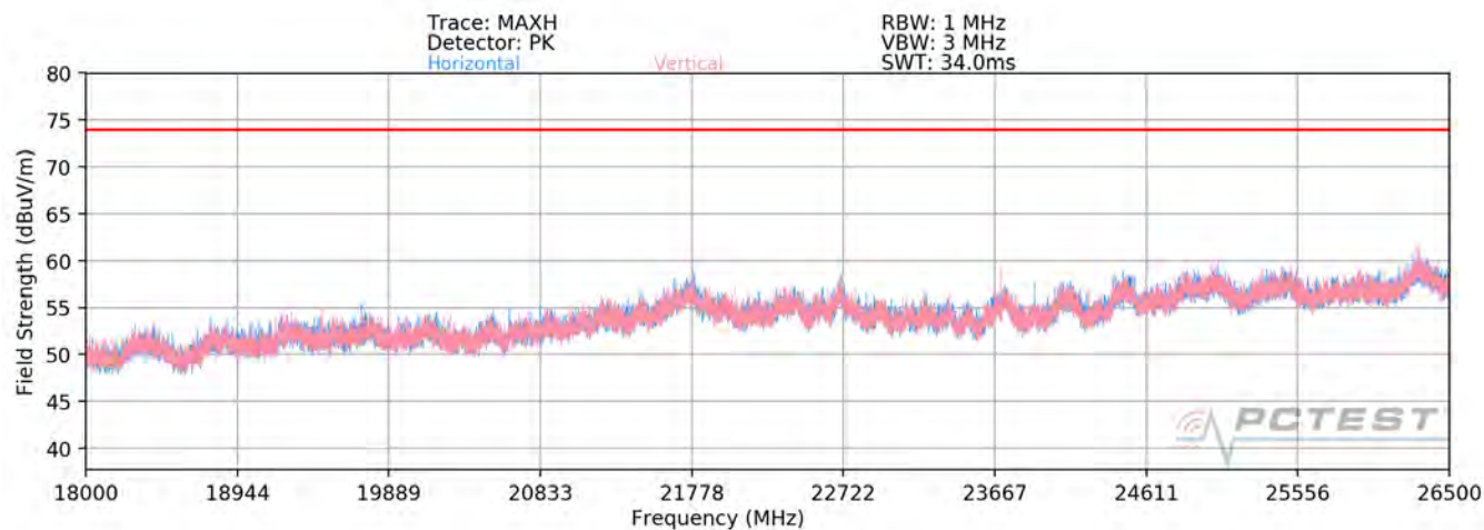
Plot 7-86. Radiated Spurious Plot above 18GHz SISO ANT2
