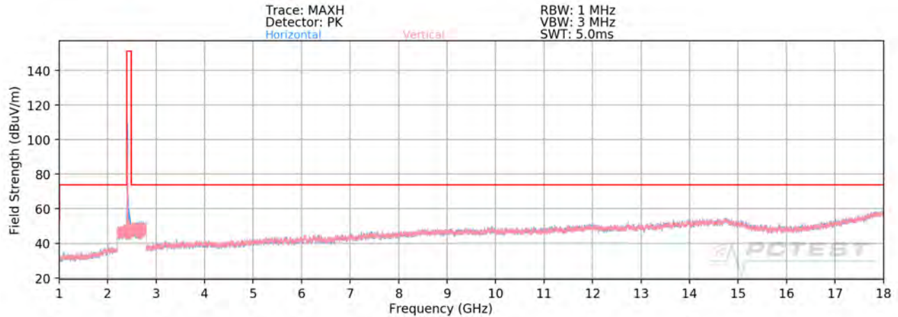
Plot 7-83. Radiated Spurious Plot above 1GHz SISO ANT2 (802.11b – Ch. 1)
