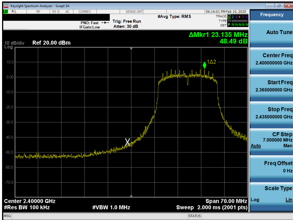
Plot 7-46. Band Edge Plot SISO ANT1 (802.11n (2.4GHz) – Ch. 2)
