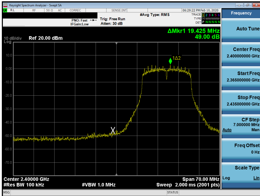
Plot 7-55. Band Edge Plot SISO ANT2 (802.11g- Ch. 2)
