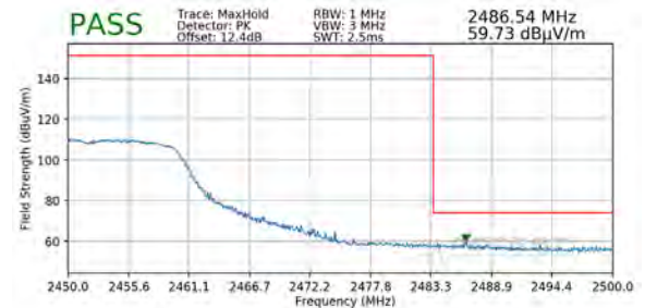
Plot 7-94. Radiated Restricted Upper Band Edge Measurement SISO ANT1 (Peak)
