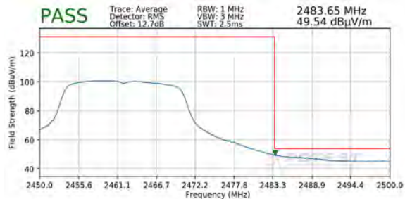
Plot 7-97. Radiated Restricted Upper Band Edge Measurement SISO ANT1 (Average)
