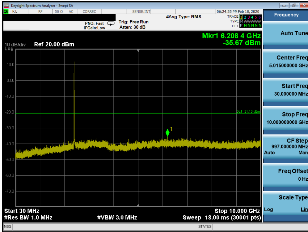
Plot 7-73. Conducted Spurious Plot SISO ANT2 (802.11b – Ch. 1)
