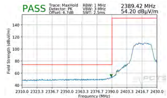
Plot 7-114. Radiated Restricted Lower Band Edge Measurement MIMO (Peak)
