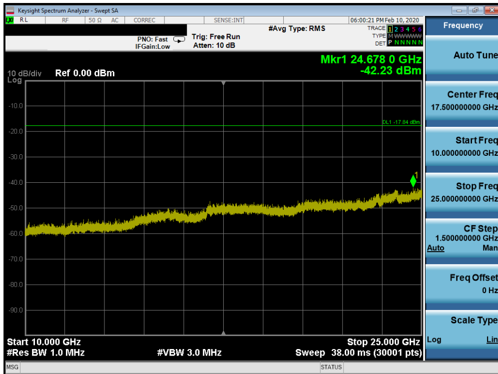
Plot 7-70. Conducted Spurious Plot SISO ANT1 (802.11b – Ch. 6)
