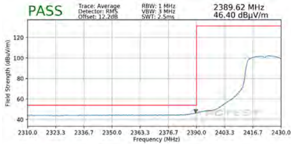
Plot 7-91. Radiated Restricted Lower Band Edge Measurement SISO ANT1 (Average)
