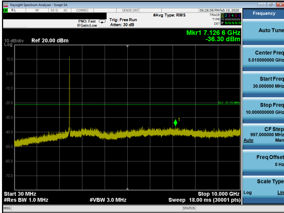
Plot 7-77. Conducted Spurious Plot SISO ANT2 (802.11b – Ch. 11)
