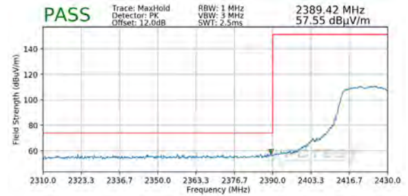
Plot 7-92. Radiated Restricted Lower Band Edge Measurement SISO ANT1 (Peak)
