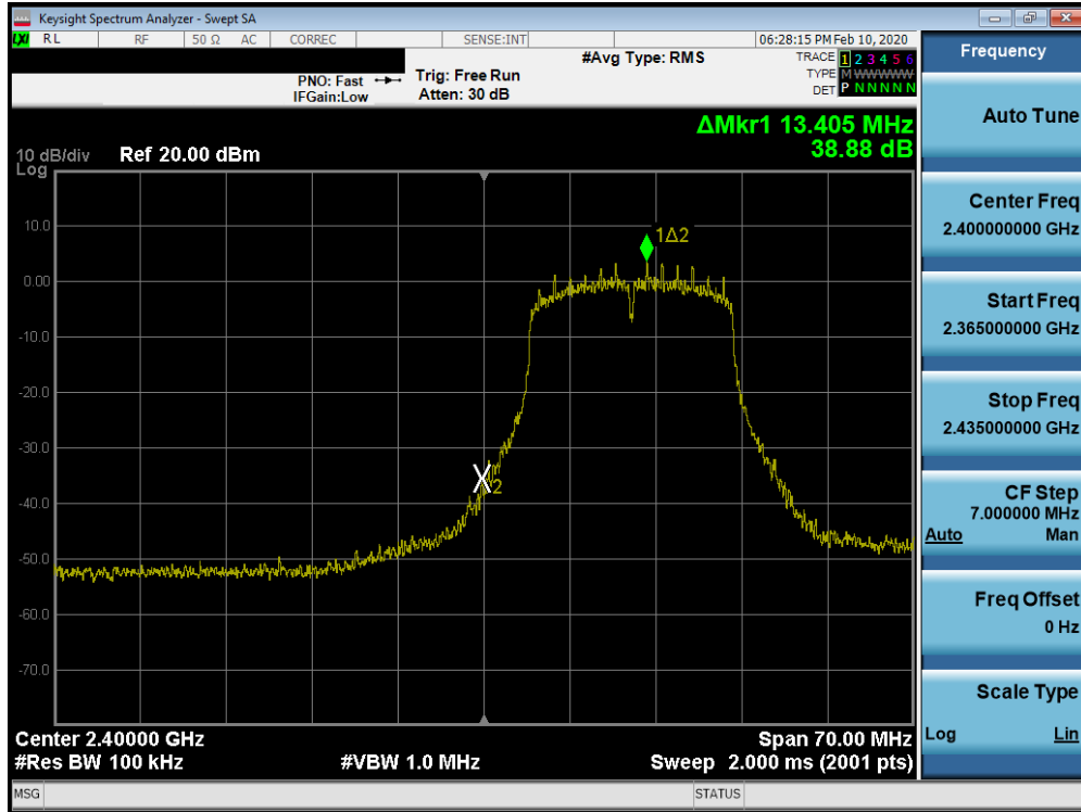
Plot 7-54. Band Edge Plot SISO ANT2 (802.11g- Ch. 1)
