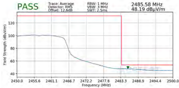
Plot 7-95. Radiated Restricted Upper Band Edge Measurement SISO ANT1 (Average)
