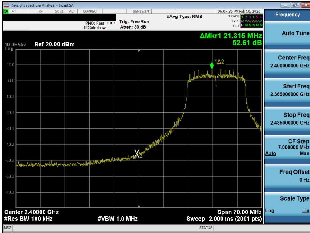
Plot 7-41. Band Edge Plot SISO ANT1 (802.11g– Ch. 3)
