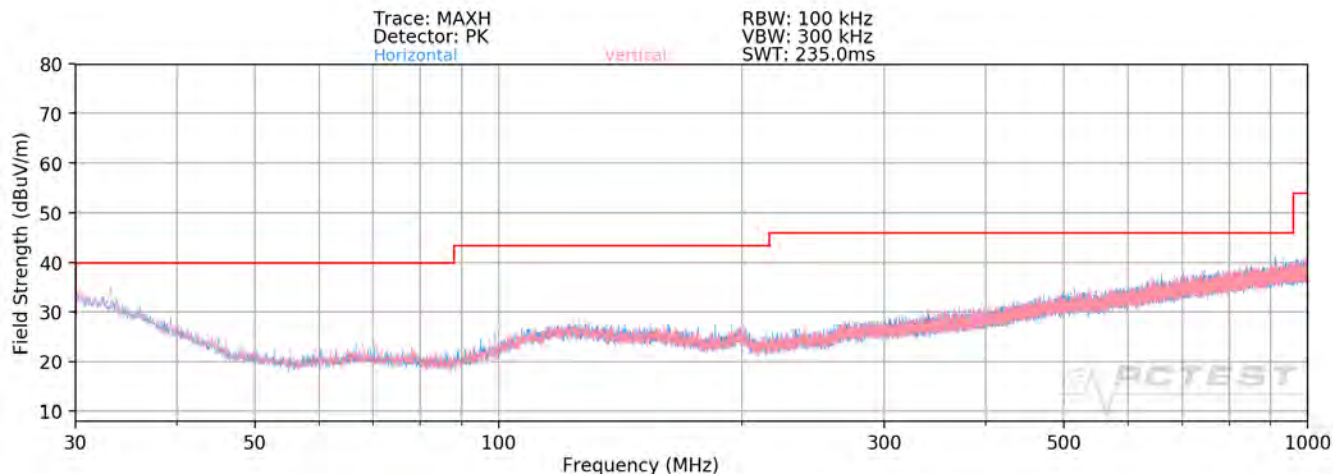
Plot 7-124. Radiated Spurious Plot below 1GHz SISO ANT2
