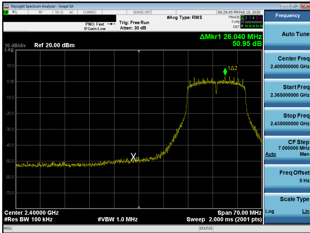
Plot 7-56. Band Edge Plot SISO ANT2 (802.11g- Ch. 3)
