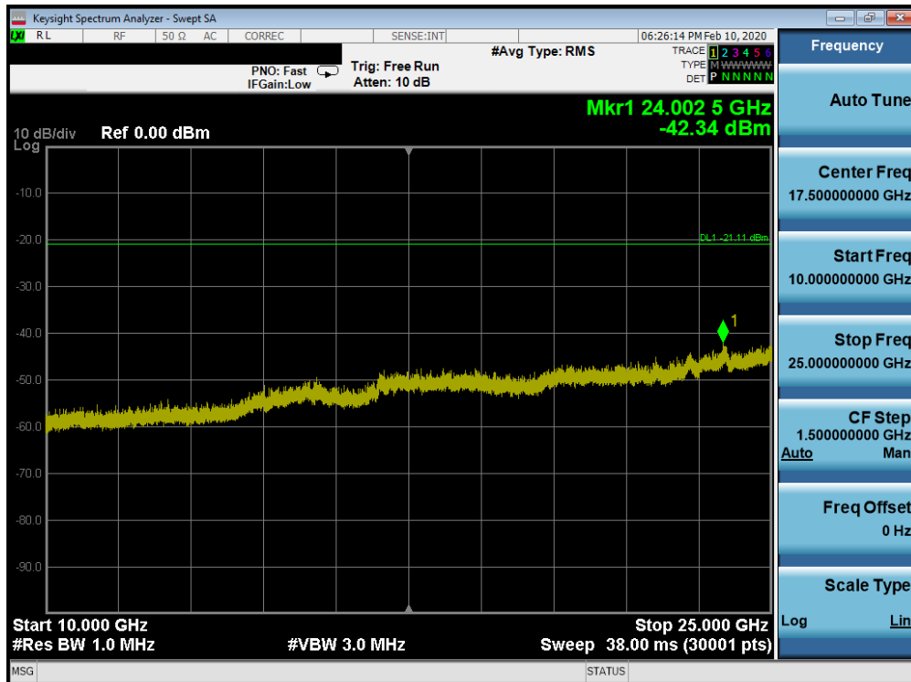
Plot 7-76. Conducted Spurious Plot SISO ANT2 (802.11b – Ch. 6)
