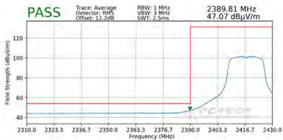
Plot 7-89. Radiated Restricted Lower Band Edge Measurement SISO ANT1 (Average)
