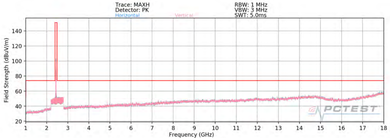
Plot 7-84. Radiated Spurious Plot above 1GHz SISO ANT2 (802.11b – Ch. 6)
