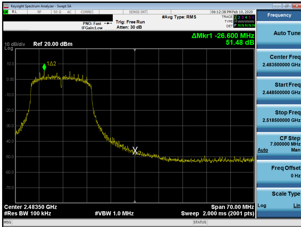
Plot 7-51. Band Edge Plot SISO ANT1 (802.11n (2.4GHz) – Ch. 11)
