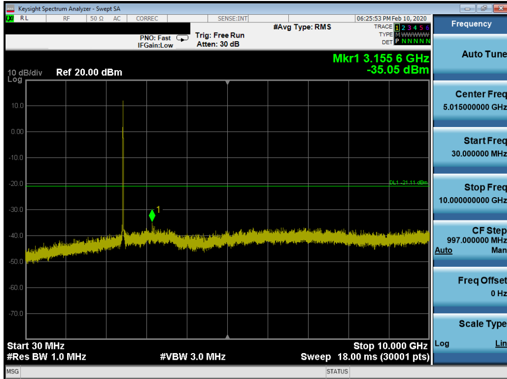
Plot 7-75. Conducted Spurious Plot SISO ANT2 (802.11b – Ch. 6)
