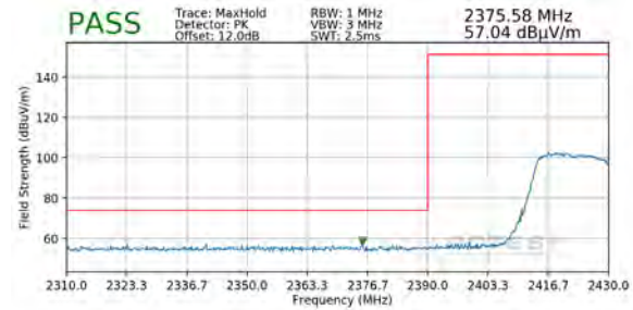
Plot 7-104. Radiated Restricted Lower Band Edge Measurement SISO ANT2 (Peak)
