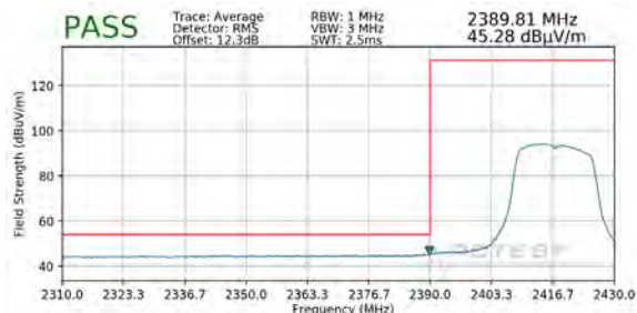
Plot 7-101. Radiated Restricted Lower Band Edge Measurement SISO ANT2 (Average)
