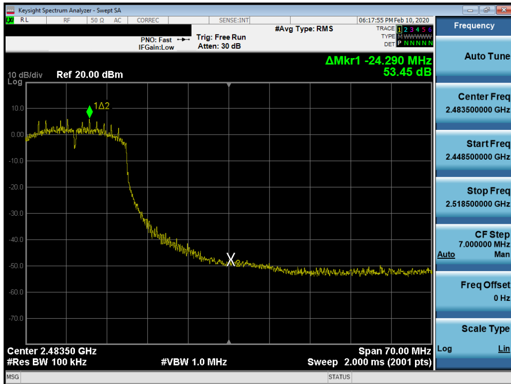
Plot 7-50. Band Edge Plot SISO ANT1 (802.11n (2.4GHz) – Ch. 10)
