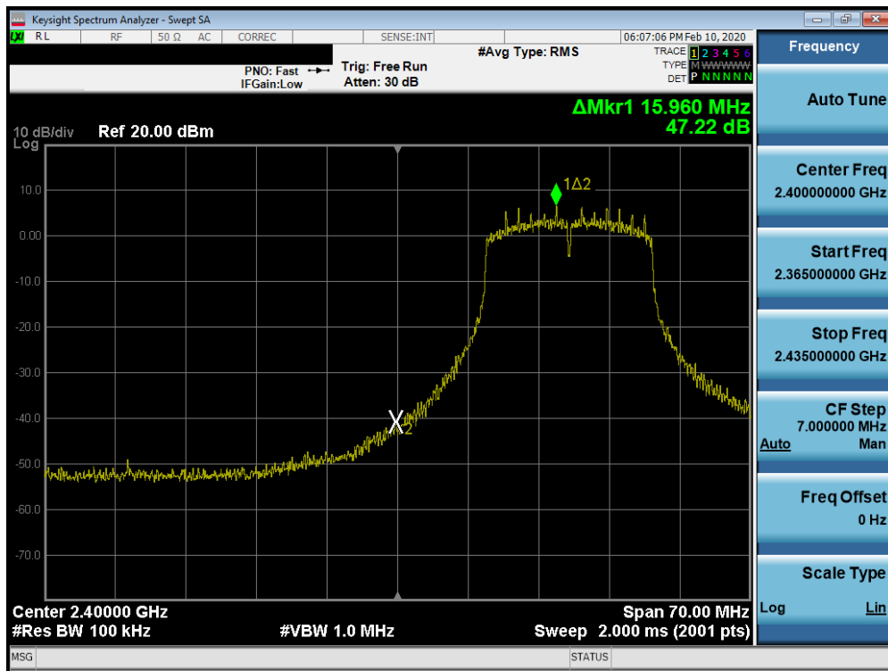
Plot 7-40. Band Edge Plot SISO ANT1 (802.11g- Ch. 2)
