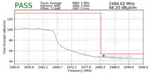
Plot 7-119. Radiated Restricted Upper Band Edge Measurement MIMO (Average)
