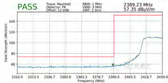
Plot 7-116. Radiated Restricted Lower Band Edge Measurement MIMO (Peak)
