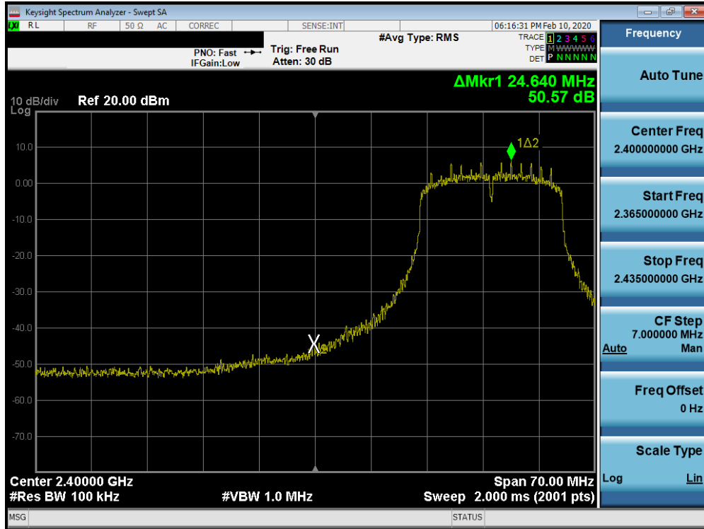
Plot 7-47. Band Edge Plot SISO ANT1 (802.11n (2.4GHz) – Ch. 3)
