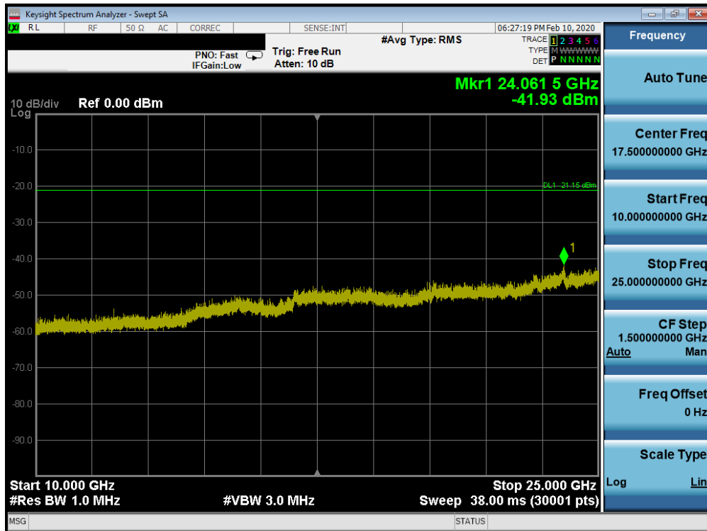
Plot 7-78. Conducted Spurious Plot SISO ANT2 (802.11b – Ch. 11)
