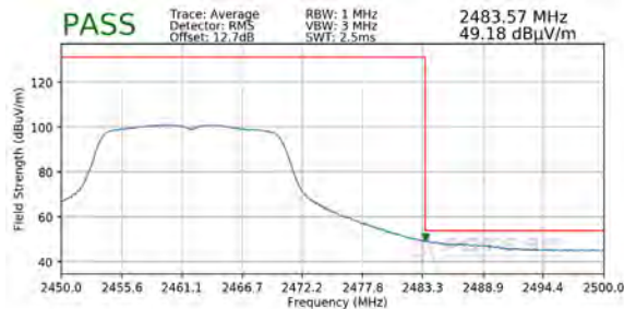
Plot 7-121. Radiated Restricted Upper Band Edge Measurement MIMO (Average)
