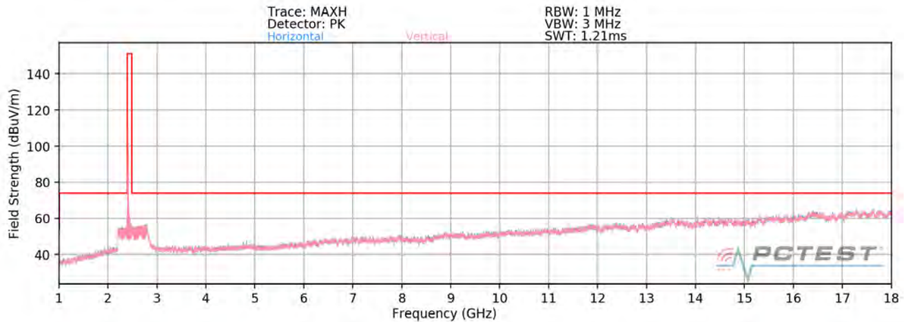
Plot 7-79. Radiated Spurious Plot above 1GHz SISO ANT1 (802.11b – Ch. 1)
