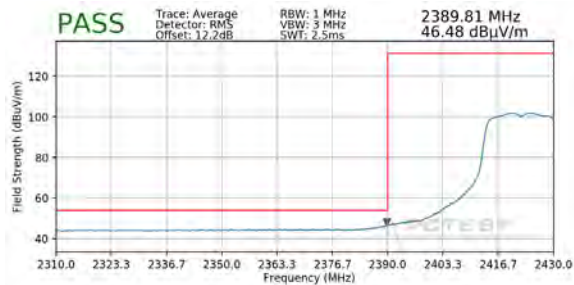
Plot 7-115. Radiated Restricted Lower Band Edge Measurement MIMO (Average)
