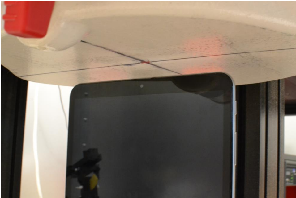
SAR Test Setup Photo 3 – Top Edge at 17 mm
