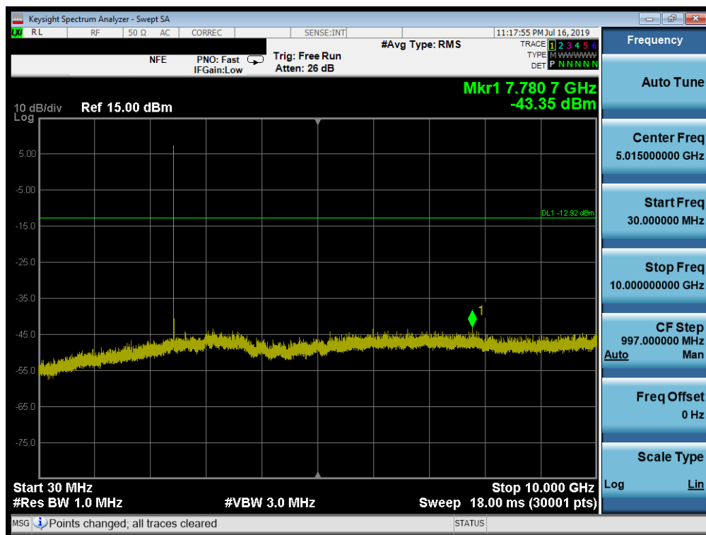
Plot 7-38. Conducted Spurious Plot (Bluetooth – Ch. 39)
