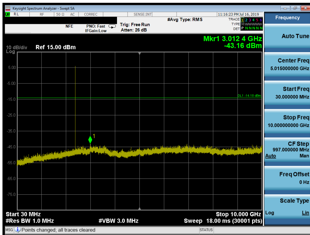
Plot 7-36. Conducted Spurious Plot (Bluetooth – Ch. 0)
