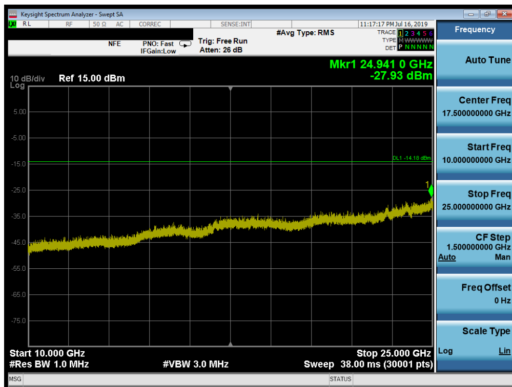
Plot 7-37. Conducted Spurious Plot (Bluetooth – Ch. 0)
