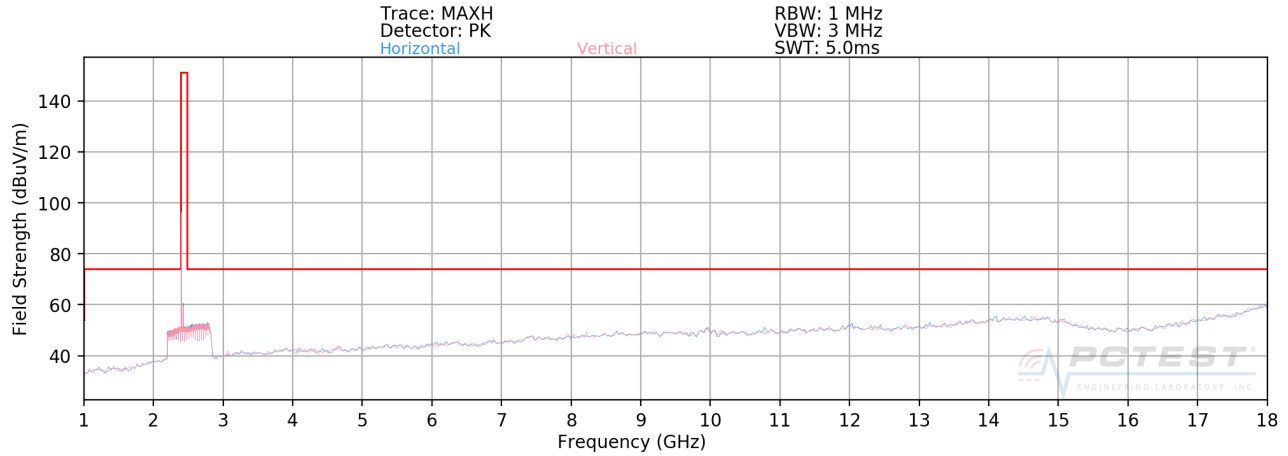
Plot 7-42. Radiated Spurious Plot above 1GHz (Bluetooth- Ch. 0)
