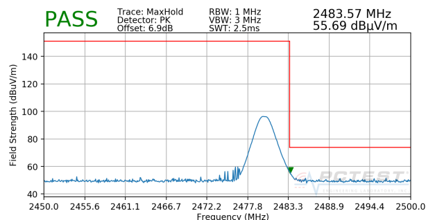
Plot 7-47. Radiated Restricted Higher Band Edge Measurement (Peak)
