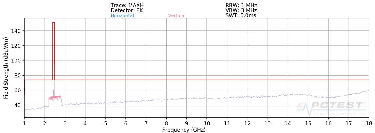
Plot 7-44. Radiated Spurious Plot above 1GHz (Bluetooth - Ch. 78)
