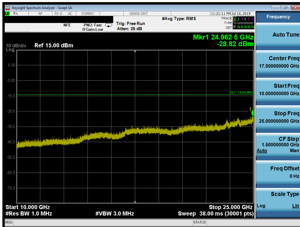
Plot 7-41. Conducted Spurious Plot (Bluetooth – Ch. 78)
