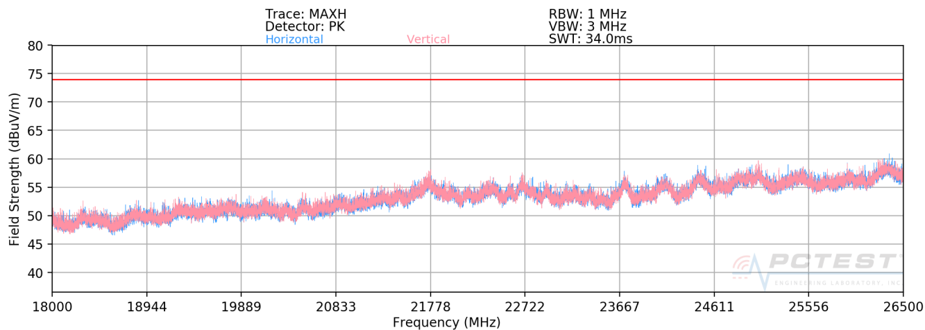
Plot 7-45. Radiated Spurious Plot above 18GHz GFSK Bluetooth
