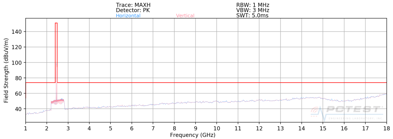
Plot 7-43. Radiated Spurious Plot above 1GHz (Bluetooth - Ch. 39)
