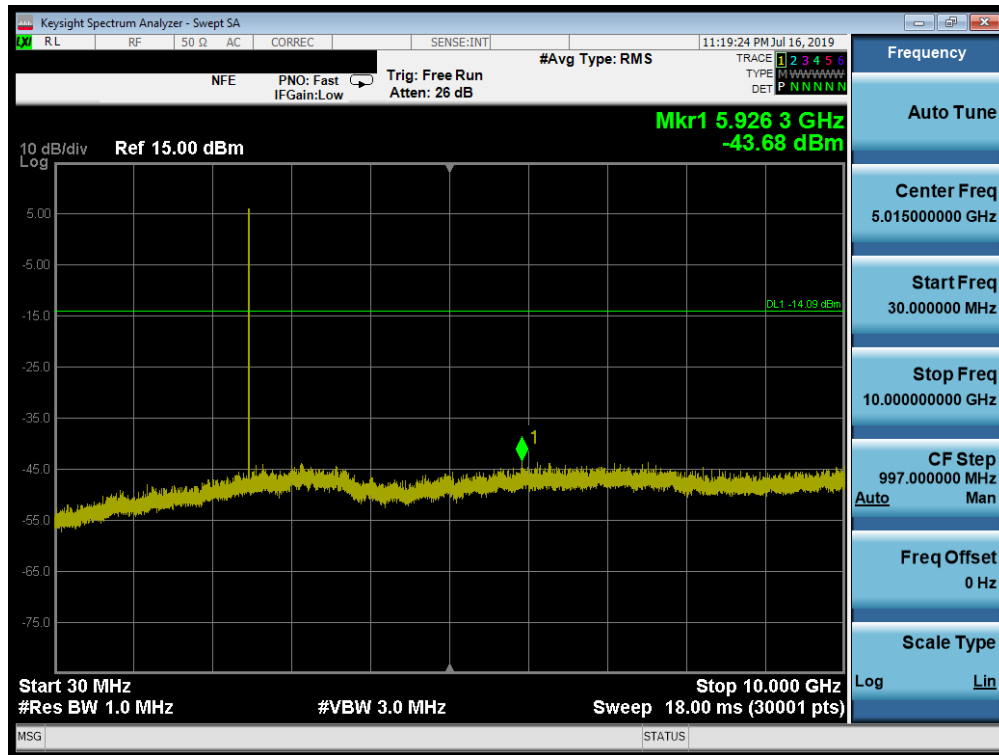
Plot 7-40. Conducted Spurious Plot (Bluetooth – Ch. 78)
