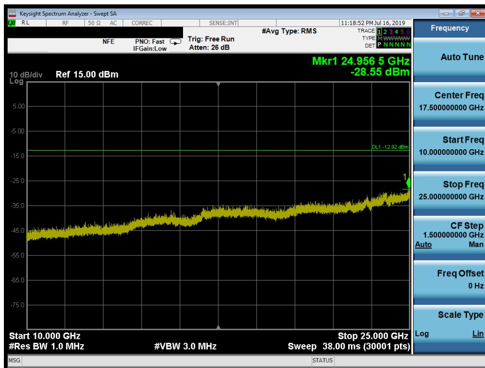
Plot 7-39. Conducted Spurious Plot (Bluetooth – Ch. 39)
