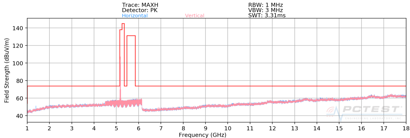
Plot 7-157. Radiated Spurious Plot above 1GHz SISO ANT1 (802.11a – U1 Ch. 40)
