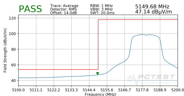
Plot 7-175. Radiated Lower Band Edge Plot SISO ANT1 (Average – UNII Band 1)
