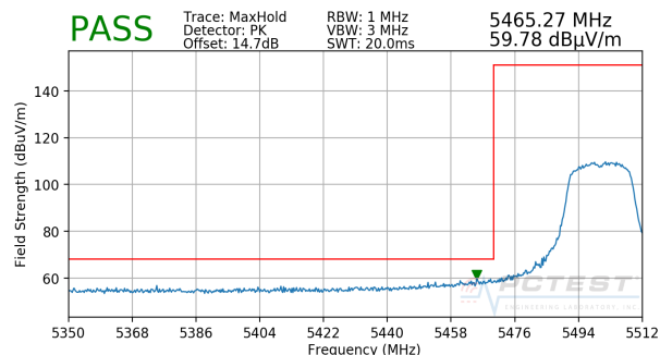
Plot 7-180. Radiated Lower Band Edge Plot SISO ANT1 (Peak – UNII Band 2C)
