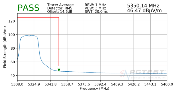
Plot 7-177. Radiated Upper Band Edge Plot SISO ANT1 (Average – UNII Band 2A)
