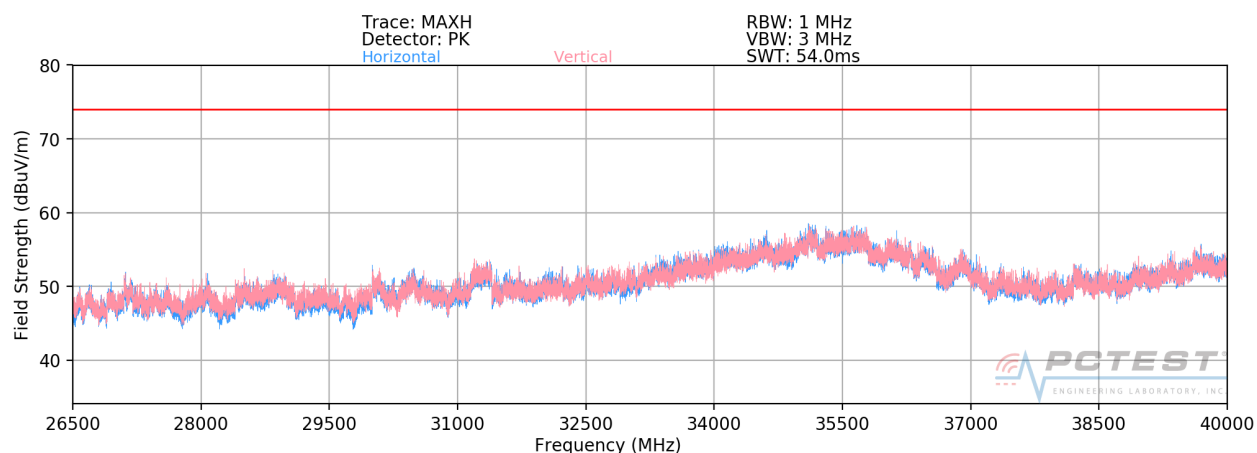
Plot 7-168. Radiated Spurious Plot 26.5GHz - 40GHz SISO ANT2 (802.11a)
