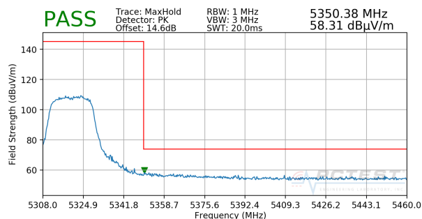
Plot 7-178. Radiated Upper Band Edge Plot SISO ANT1 (Peak – UNII Band 2A)
