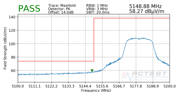
Plot 7-176. Radiated Lower Band Edge Plot SISO ANT1 (Peak – UNII Band 1)
