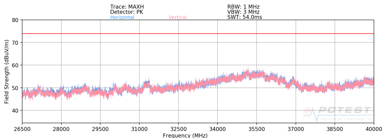
Plot 7-162. Radiated Spurious Plot 26.5GHz - 40GHz SISO ANT1 (802.11a)
