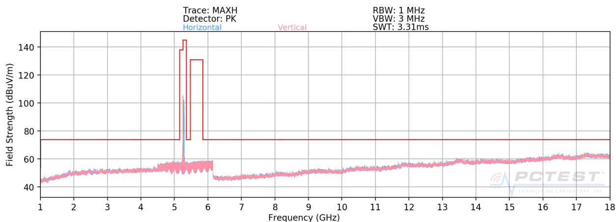
Plot 7-158. Radiated Spurious Plot above 1GHz SISO ANT1 (802.11a – U2A Ch. 56)
