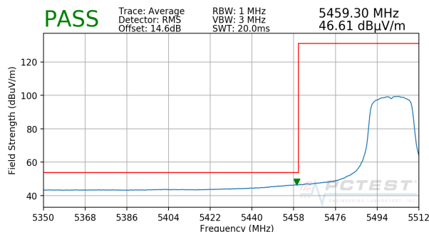
Plot 7-179. Radiated Lower Band Edge Plot SISO ANT1 (Average – UNII Band 2C)
