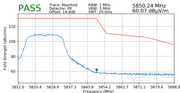
Plot 7-181. Radiated Upper Band Edge Plot SISO ANT1 (Peak – UNII Band 3)
