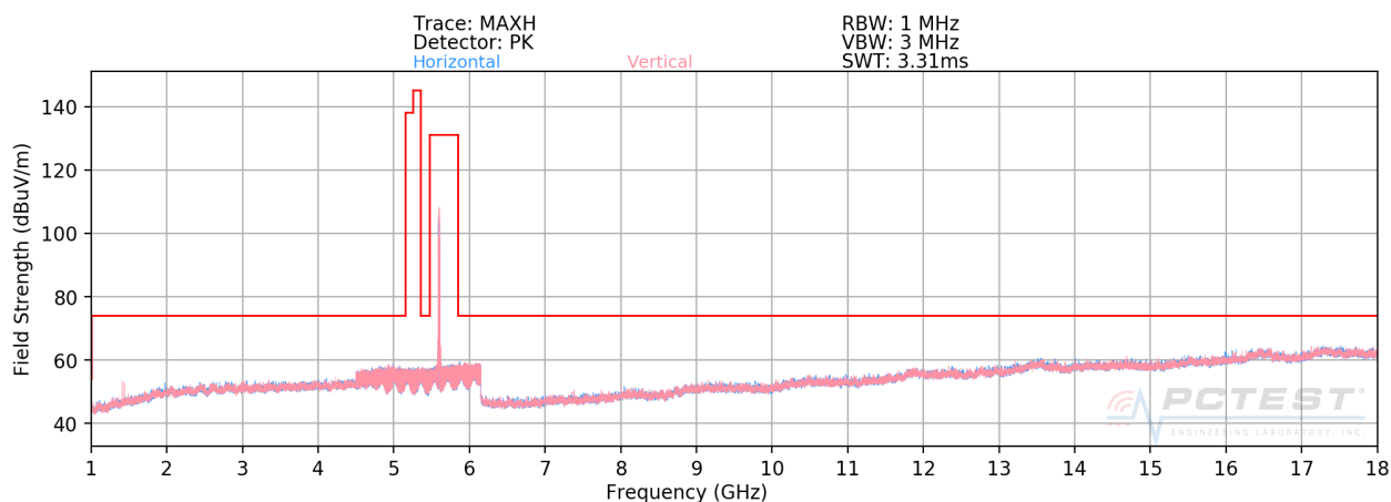
Plot 7-159. Radiated Spurious Plot above 1GHz SISO ANT1 (802.11a – U2C Ch. 120)
