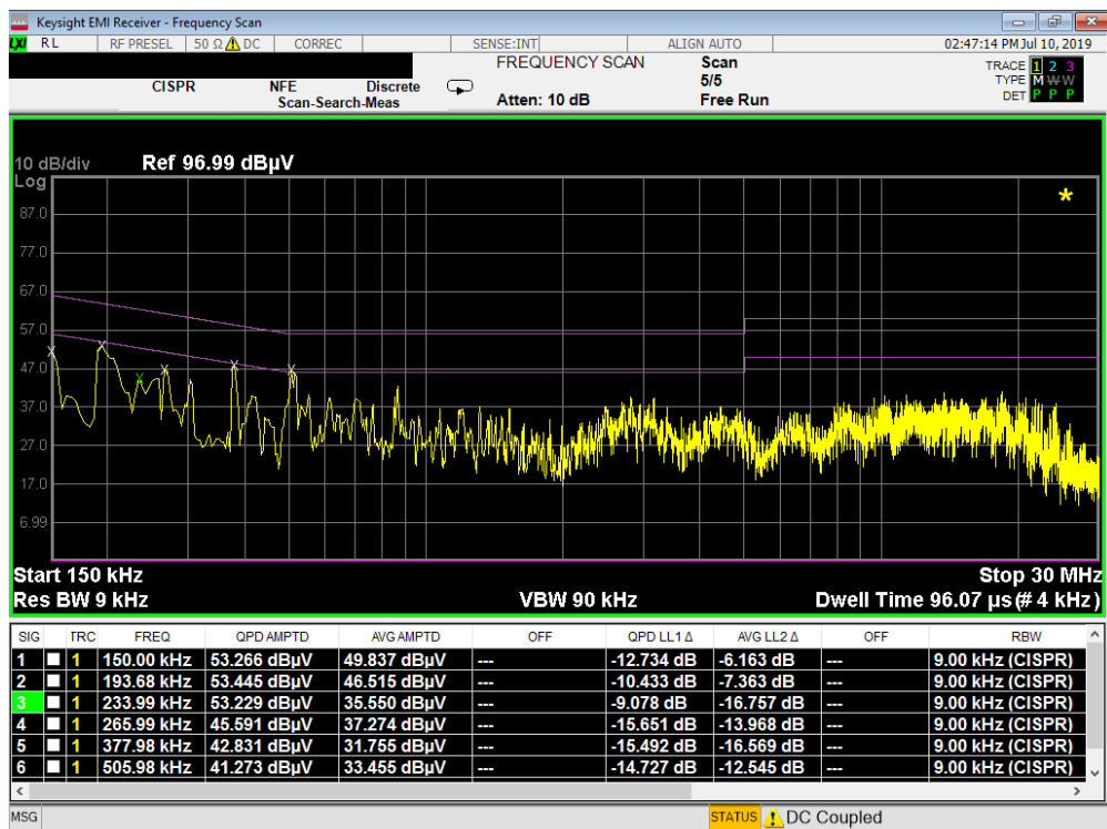
Plot 7-87. Line Conducted Plot with 802.11b (L1)
