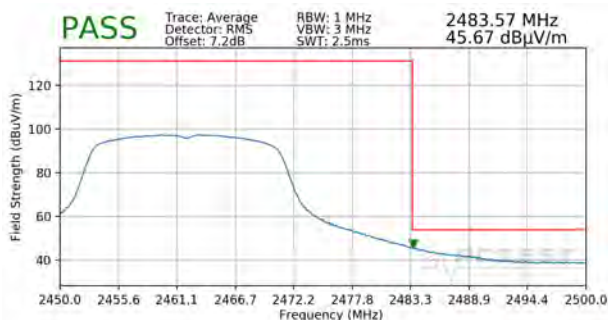
Plot 7-79. Radiated Restricted Upper Band Edge Measurement SISO ANT2 (Average)
