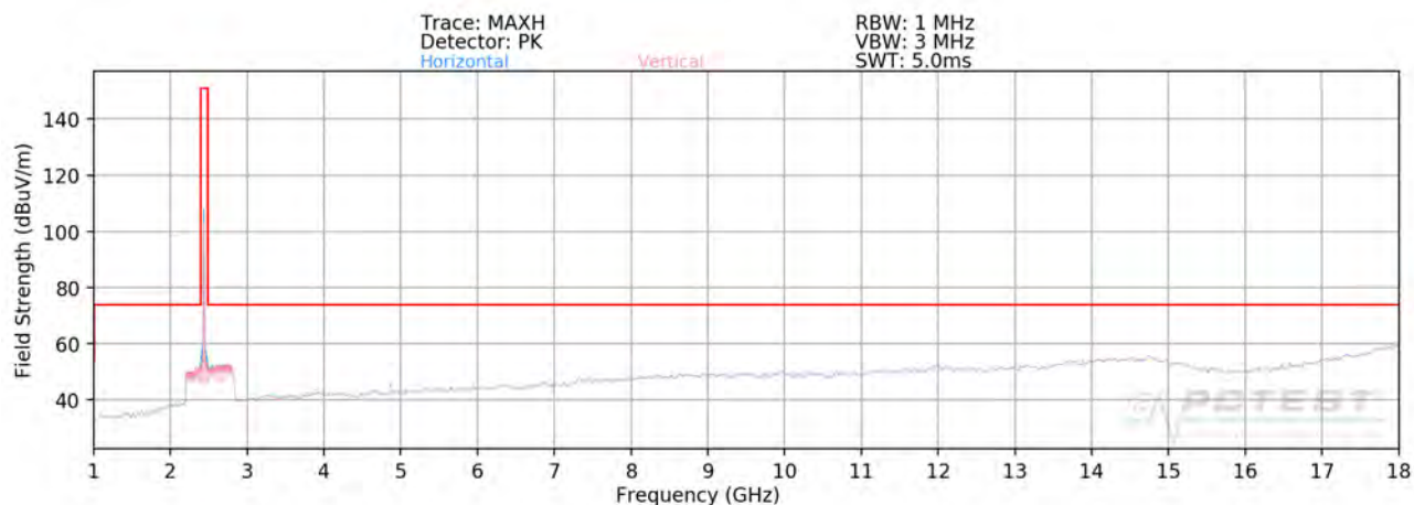
Plot 7-70. Radiated Spurious Plot above 1GHz MIMO/CDD (802.11g – Ch. 6)
