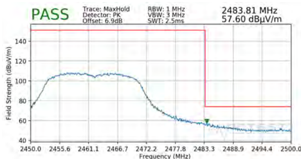
Plot 7-84. Radiated Restricted Upper Band Edge Measurement MIMO (Peak)
