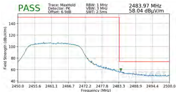
Plot 7-80. Radiated Restricted Upper Band Edge Measurement SISO ANT2 (Peak)
