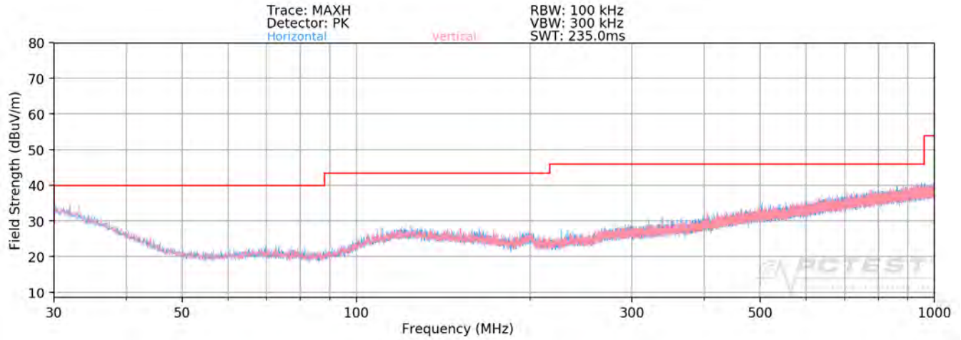
Plot 7-85. Radiated Spurious Plot below 1GHz SISO ANT1
