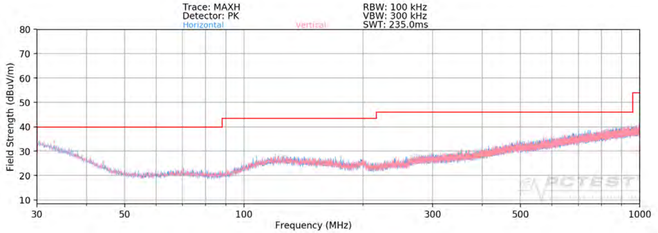
Plot 7-86. Radiated Spurious Plot below 1GHz SISO ANT2
