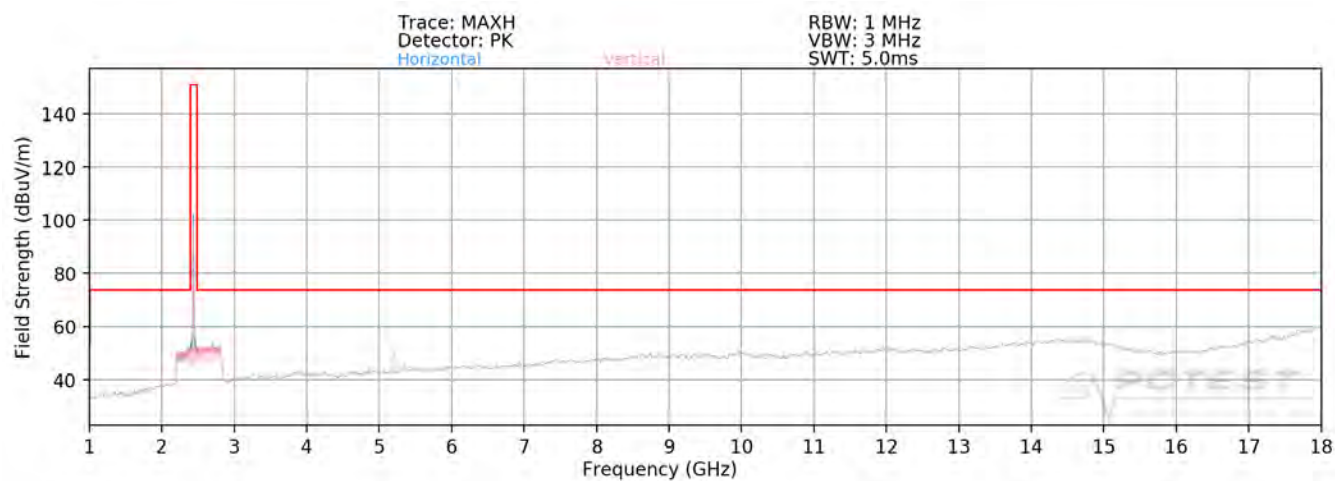
Plot 7-66. Radiated Spurious Plot above 1GHz SISO ANT2 (802.11b – Ch. 6)
