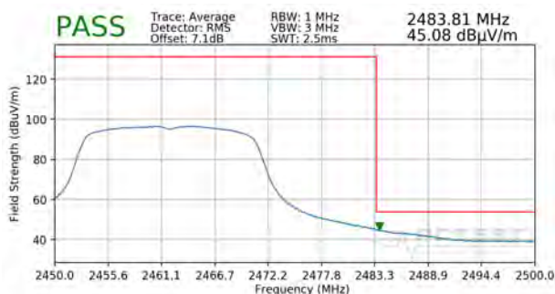
Plot 7-83. Radiated Restricted Upper Band Edge Measurement MIMO (Average)
