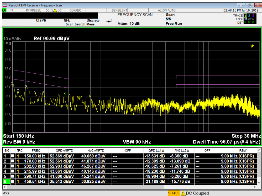
Plot 7-88. Line Conducted Plot with 802.11b (N)
