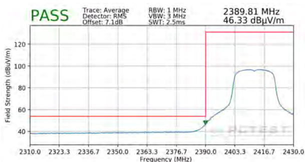
Plot 7-73. Radiated Restricted Lower Band Edge Measurement SISO ANT1 (Average)
