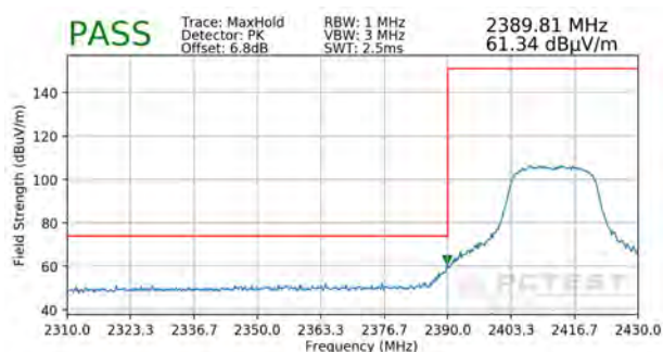
Plot 7-74. Radiated Restricted Lower Band Edge Measurement SISO ANT1 (Peak)
