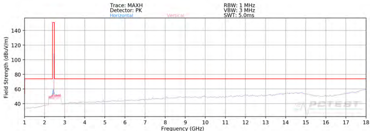
Plot 7-71. Radiated Spurious Plot above 1GHz MIMO/CDD (802.11g – Ch. 11)
