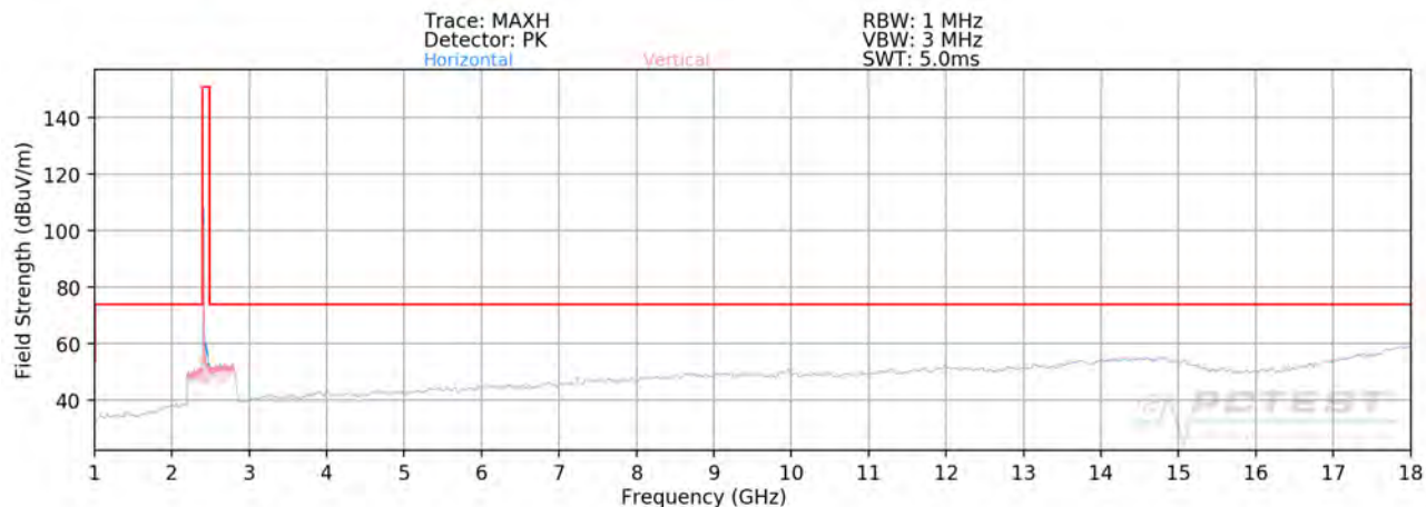
Plot 7-69. Radiated Spurious Plot above 1GHz MIMO/CDD (802.11g – Ch. 1)
