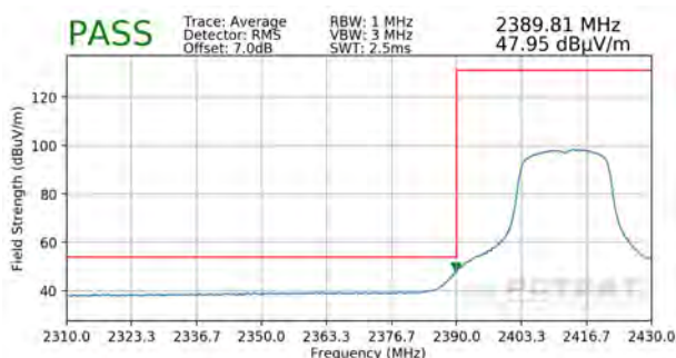
Plot 7-81. Radiated Restricted Lower Band Edge Measurement MIMO (Average)
