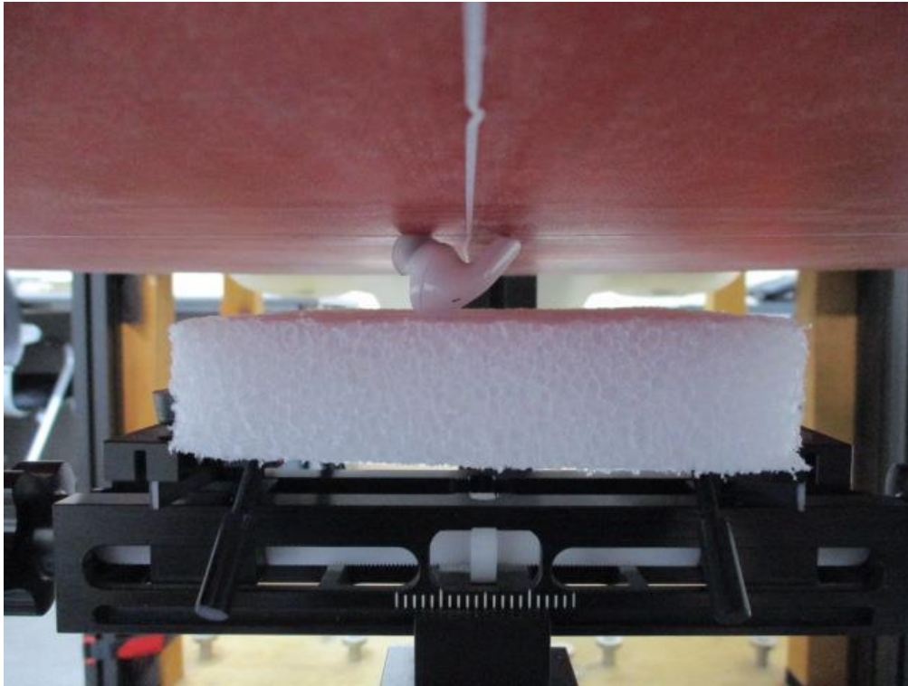
Right Ear & Front Side from Flat Phantom (Separation Distance: 0 cm) – Right Ear
