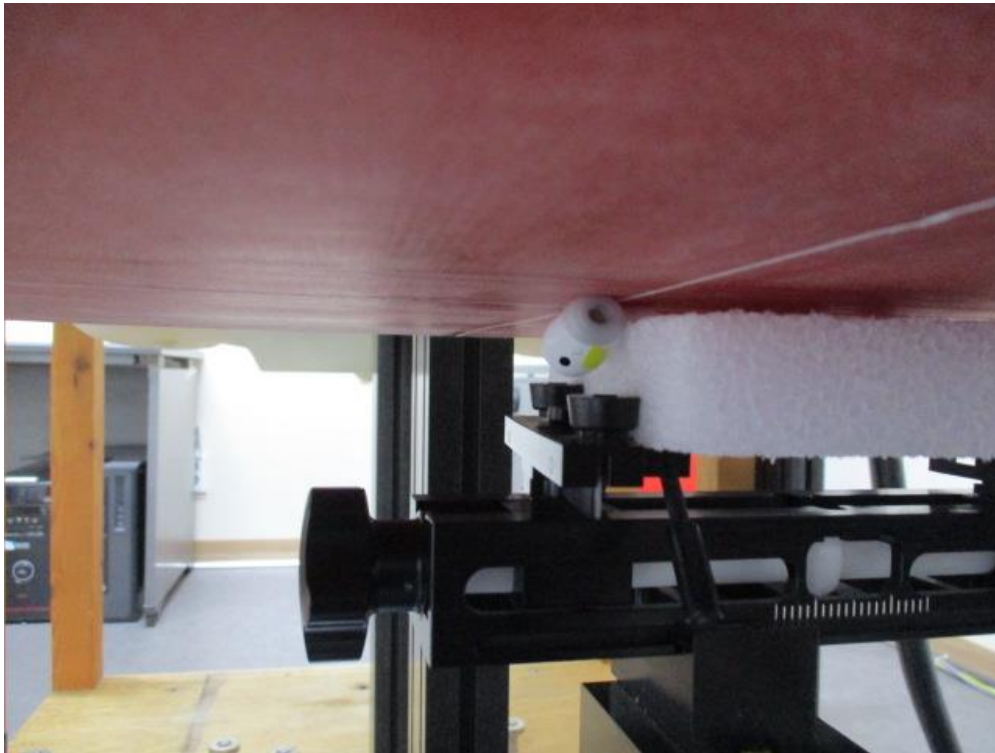
Right Side from Flat Phantom (Separation Distance: 0 cm) – Left Ear
