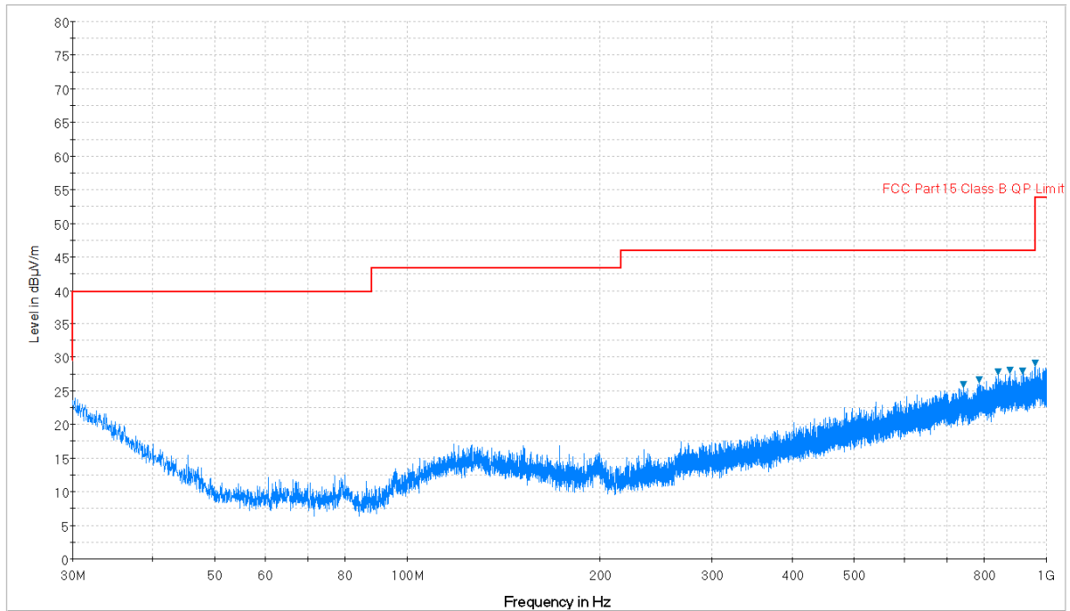
Plot 7-93. Radiated Spurious Plot below 1GHz (802.11a – U3 Ch. 157, Ant. Pol. H)
