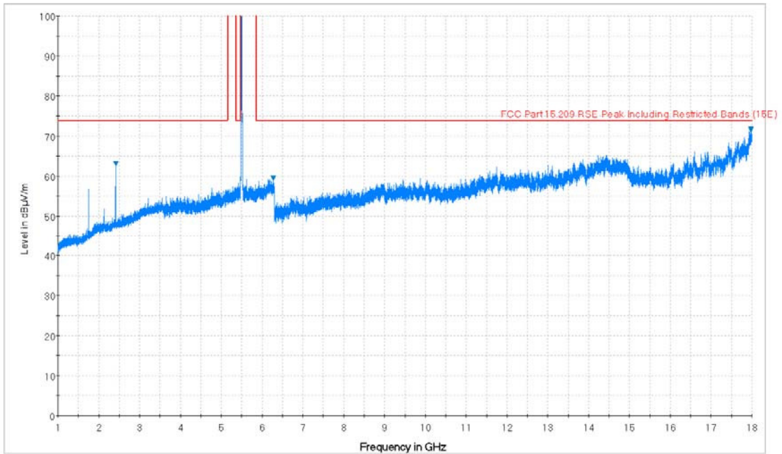
Plot 7-72. Radiated Spurious Plot above 1GHz (802.11a – U2C Ch. 116, Ant. Pol. V)
