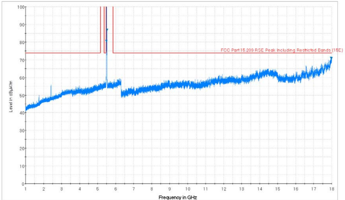
Plot 7-71. Radiated Spurious Plot above 1GHz (802.11a – U2C Ch. 116, Ant. Pol. H)
