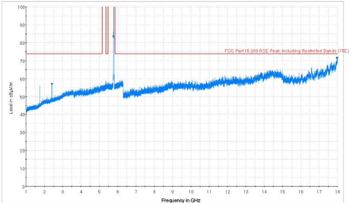
Plot 7-73. Radiated Spurious Plot above 1GHz (802.11a – U3 Ch. 157, Ant. Pol. H)
