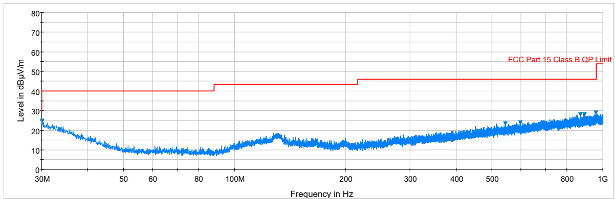
Plot 7-47. Radiated Spurious Plot below 1GHz (Pol. H)
