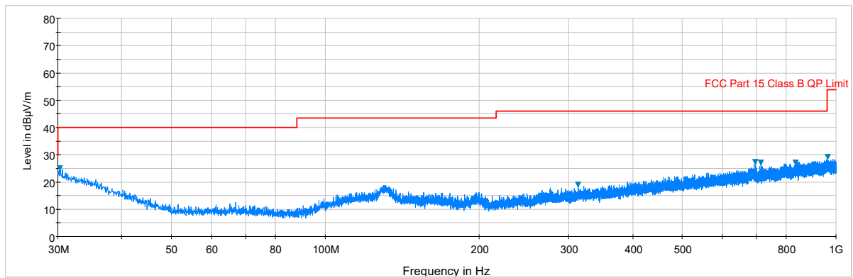
Plot 7-48. Radiated Spurious Plot below 1GHz (Pol. V)
