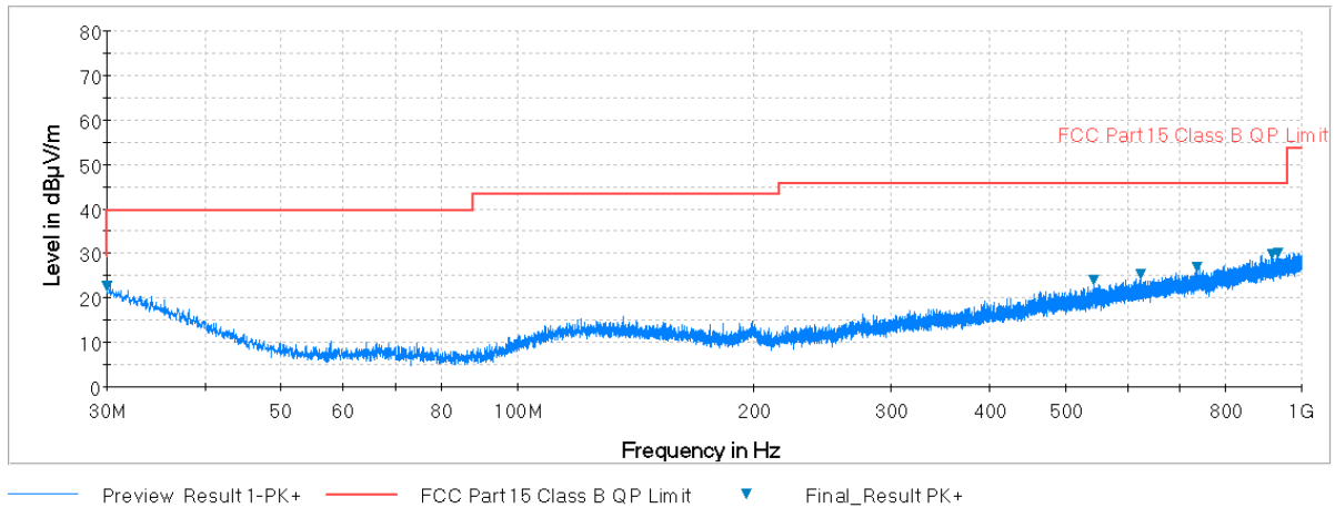
Plot 7-17. Radiated Spurious Plot below 1GHz (Pol. H)
