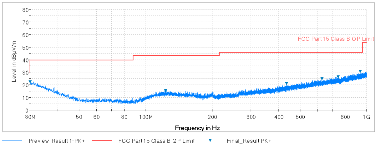
Plot 7-18. Radiated Spurious Plot below 1GHz (Pol. V)
