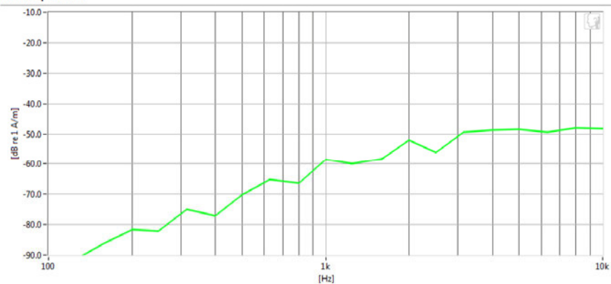
Noise Spectrum
