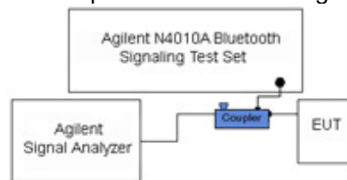
Figure 7-1. Test Instrument & Measurement Setup
