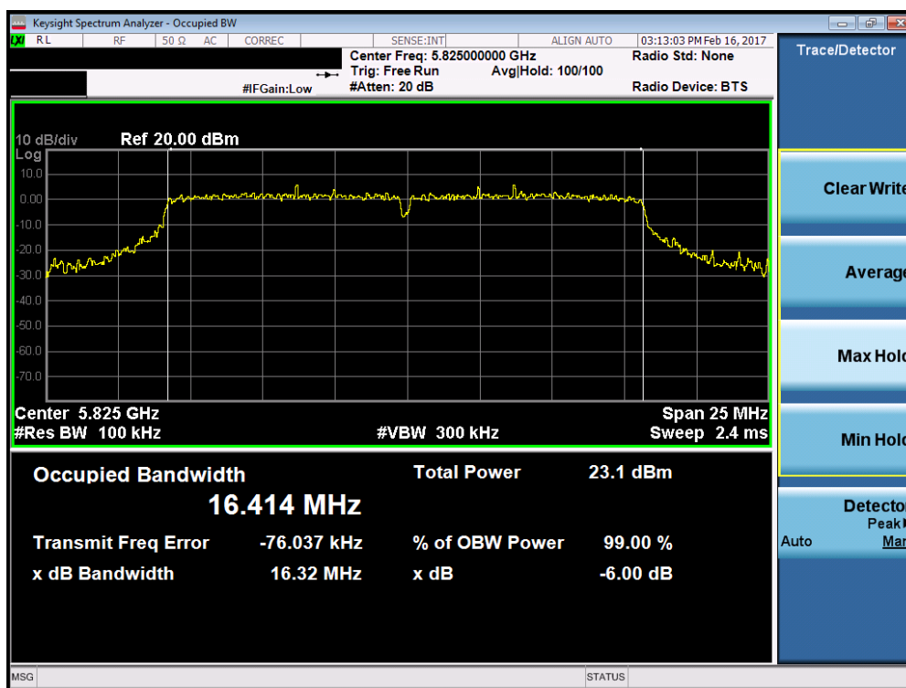
Plot 7-31. 6dB Bandwidth Plot (802.11a (UNII Band 3) – Ch. 165)
