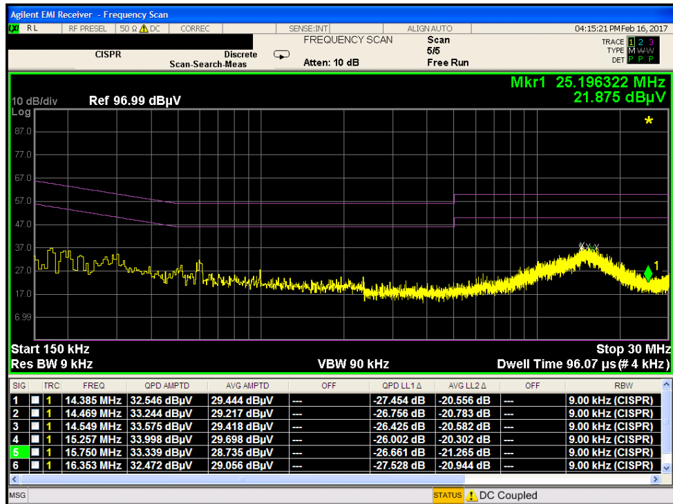
Plot 7-46. Line Conducted Plot with 802.11b (N)
