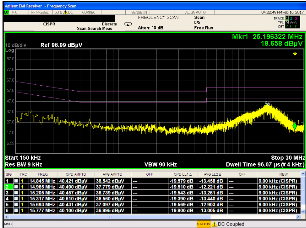
Plot 7-45. Line Conducted Plot with 802.11b (L1)
