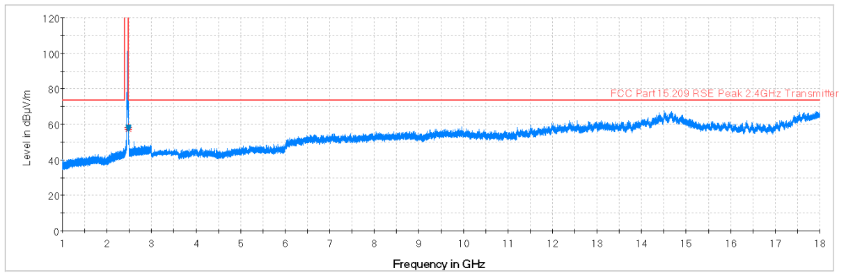
Plot 7-35. Radiated Spurious Plot above 1GHz (802.11b – Ch. 11, Ant. Pol. H)
