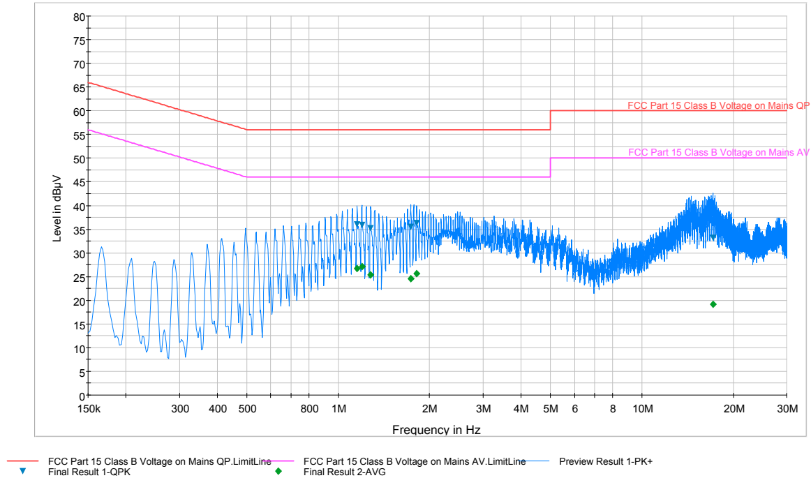
Plot 6-63. Line Conducted Plot with 802.11b (L1)
