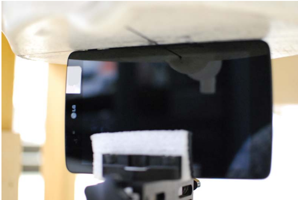
SAR Test Setup Photo 5 – Right Edge at 0.0 mm
