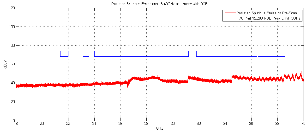
Plot 6-75. Radiated Spurious Plot above 18GHz (802.11a – Ant. Pol. H)
