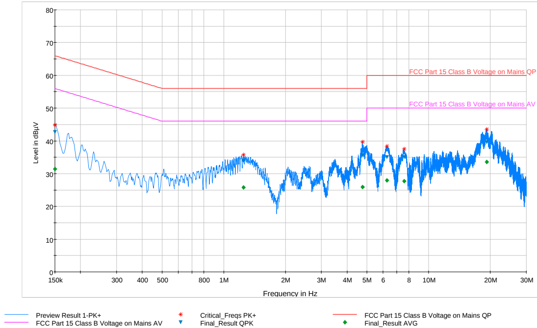
Plot 6-93. Line Conducted Plot with 802.11a UNII Band 2A (L1)
