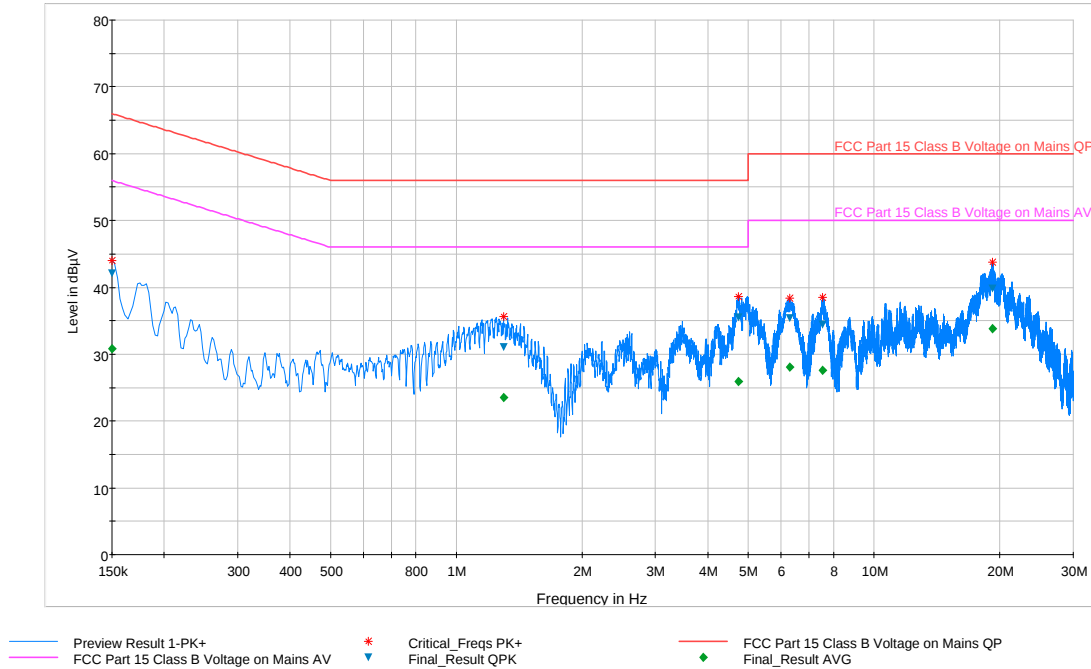
Plot 6-97. Line Conducted Plot with 802.11a UNII Band 3 (L1)
