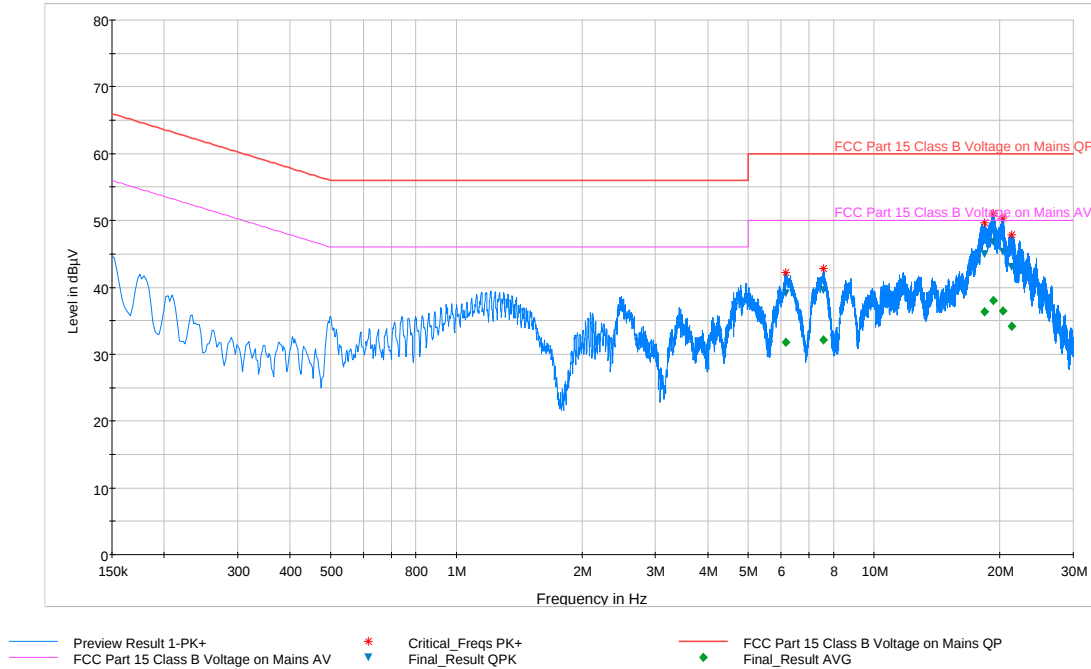
Plot 6-98. Line Conducted Plot with 802.11a UNII Band 3 (N)
