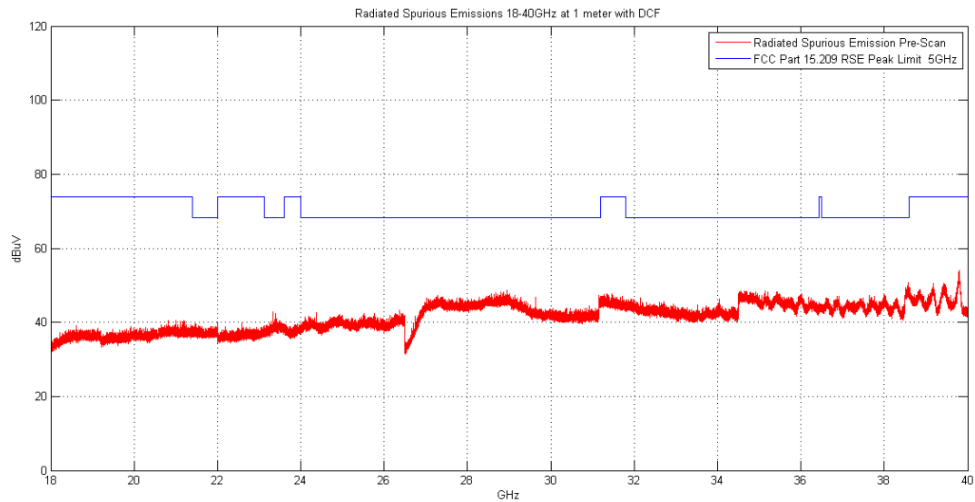
Plot 6-76. Radiated Spurious Plot above 18GHz (802.11a – Ant. Pol. V)
