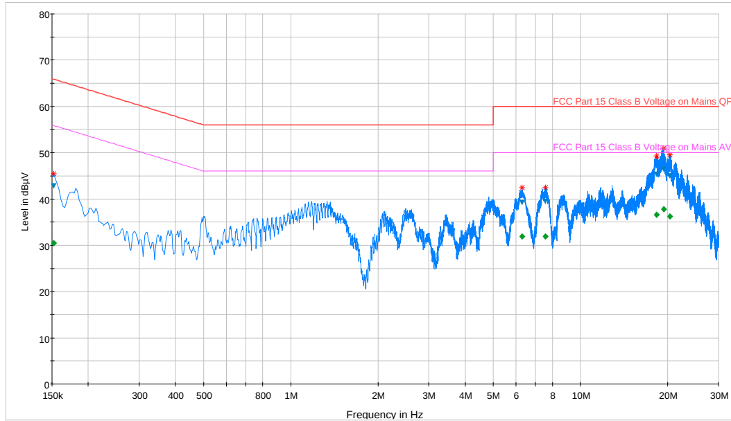
Plot 6-92. Line Conducted Plot with 802.11a UNII Band 1 (N)
