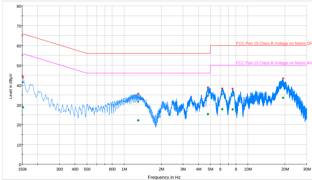
Plot 6-95. Line Conducted Plot with 802.11a UNII Band 2C (L1)
