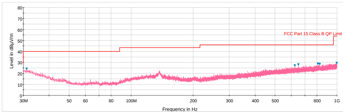
Plot 6-90. Radiated Spurious Plot below 1GHz (802.11a – U3 Ch. 157, Ant. Pol. V)
