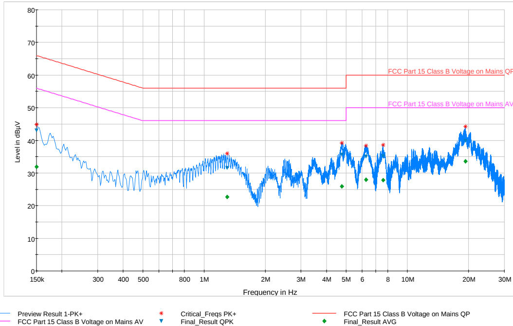
Plot 6-91. Line Conducted Plot with 802.11a UNII Band 1 (L1)
