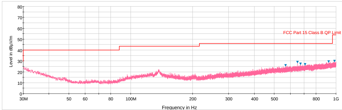
Plot 6-89. Radiated Spurious Plot below 1GHz (802.11a – U3 Ch. 157, Ant. Pol. H)
