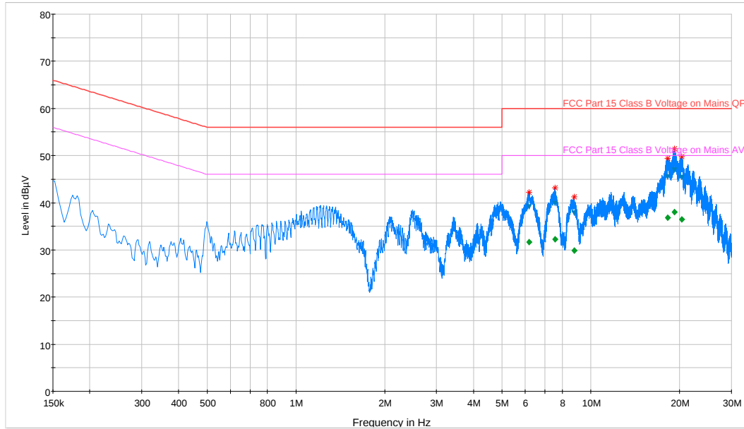
Plot 6-96. Line Conducted Plot with 802.11a UNII Band 2C (N)
