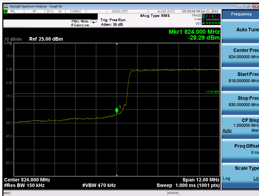
Plot 7-107. Lower Band Edge Plot (Band 26 – 15.0MHz QPSK – RB Size 75)
