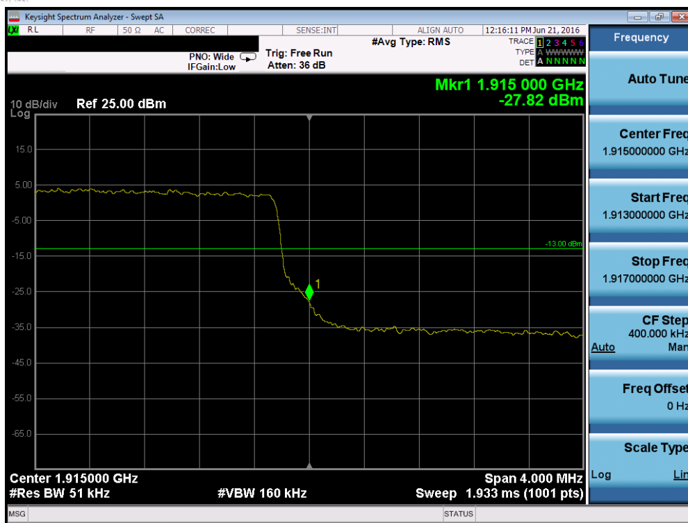
Plot 7-143. Upper Band Edge Plot (Band 2/25 - 5.0MHz QPSK - RB Size 25)
