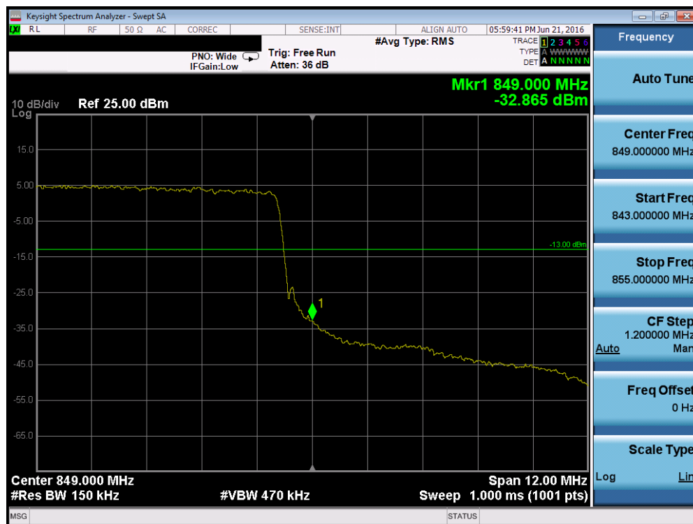
Plot 7-108. Upper Band Edge Plot (Band 26 – 15.0MHz QPSK – RB Size 75)
