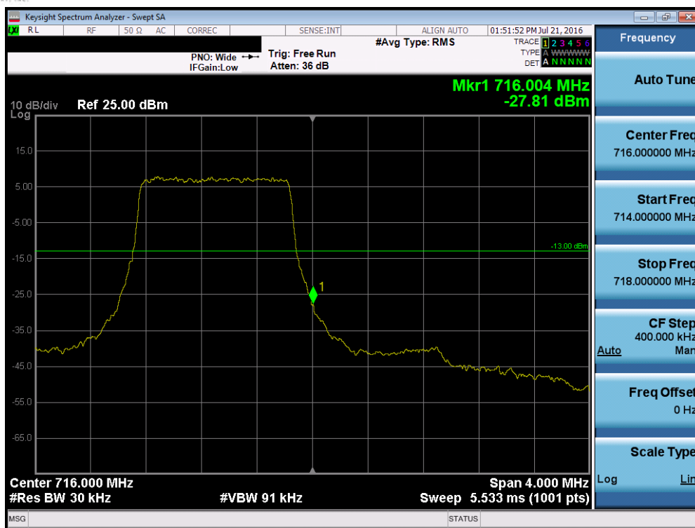
Plot 7-81. Upper Band Edge Plot (Band 12 - 1.4MHz QPSK - RB Size 6)
