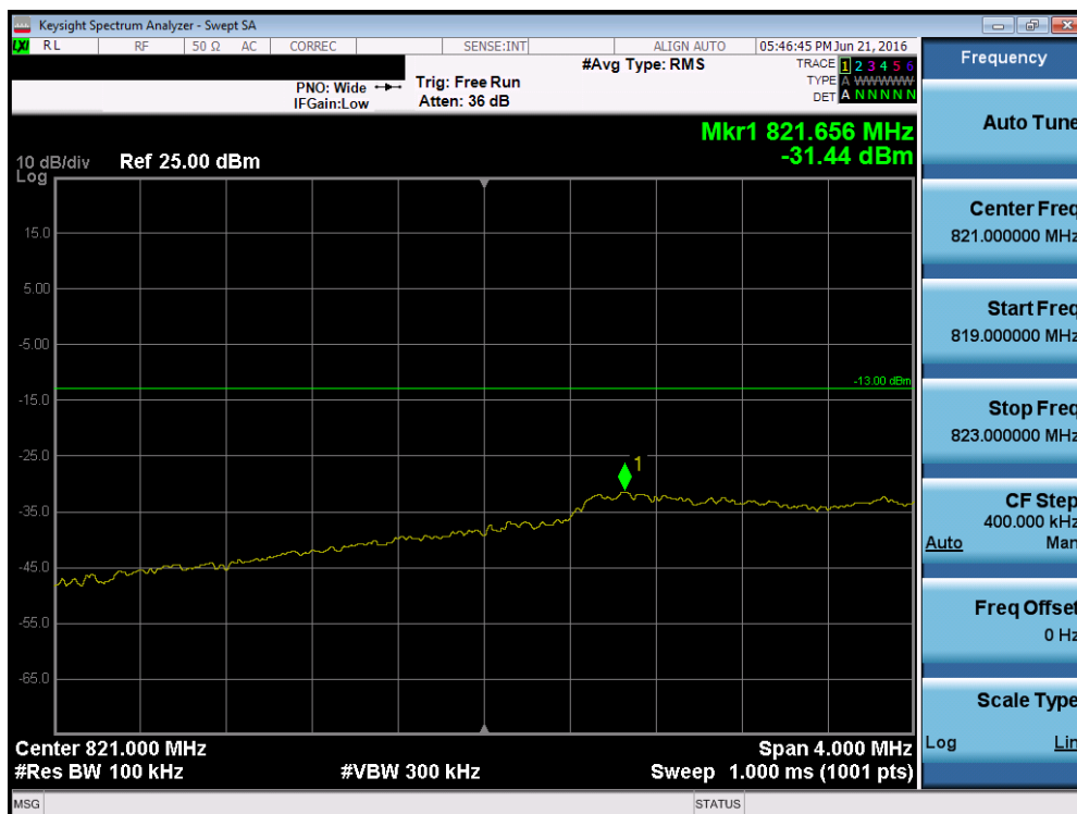
Plot 7-98. Lower Extended Band Edge Plot (Band 5/26 – 3.0MHz QPSK – RB Size 15)
