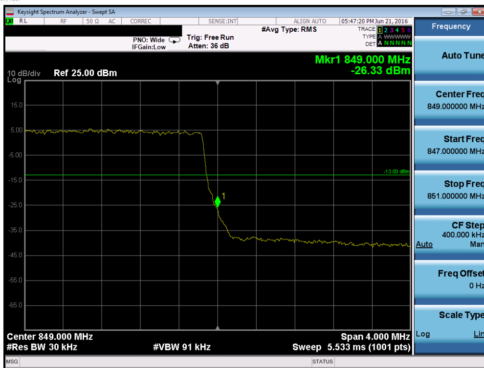
Plot 7-99. Upper Band Edge Plot (Band 5/26 – 3.0MHz QPSK – RB Size 15)
