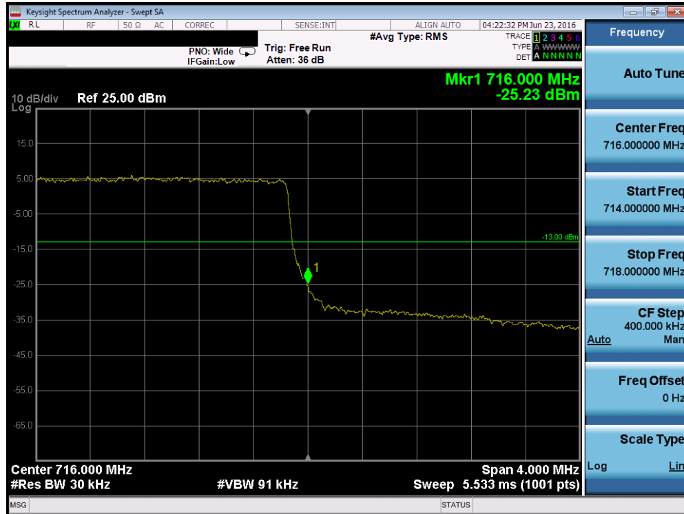
Plot 7-85. Upper Band Edge Plot (Band 12 – 3.0MHz QPSK – RB Size 15)
