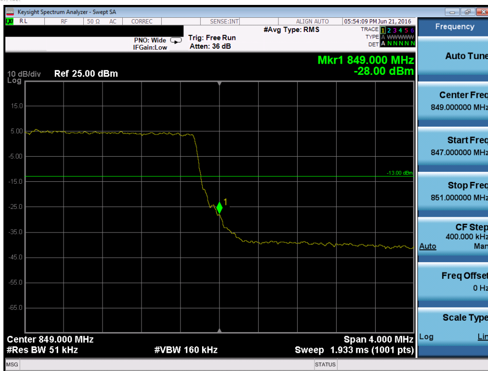
Plot 7-103. Upper Band Edge Plot (Band 5/26 – 5.0MHz QPSK – RB Size 25)
