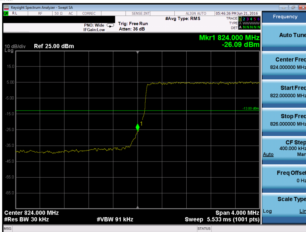
Plot 7-97. Lower Band Edge Plot (Band 5/26 – 3.0MHz QPSK – RB Size 15)
