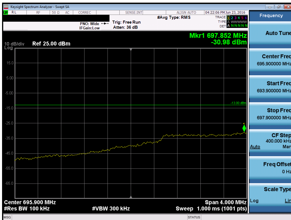
Plot 7-84. Lower Extended Band Edge Plot (Band 12 – 3.0MHz QPSK – RB Size 15)
