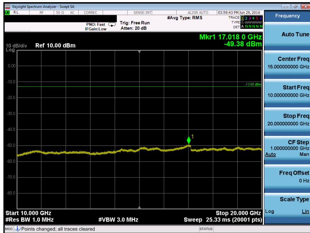
Plot 7-14. Conducted Spurious Plot (PCS WCDMA Mode – Ch. 9262)
