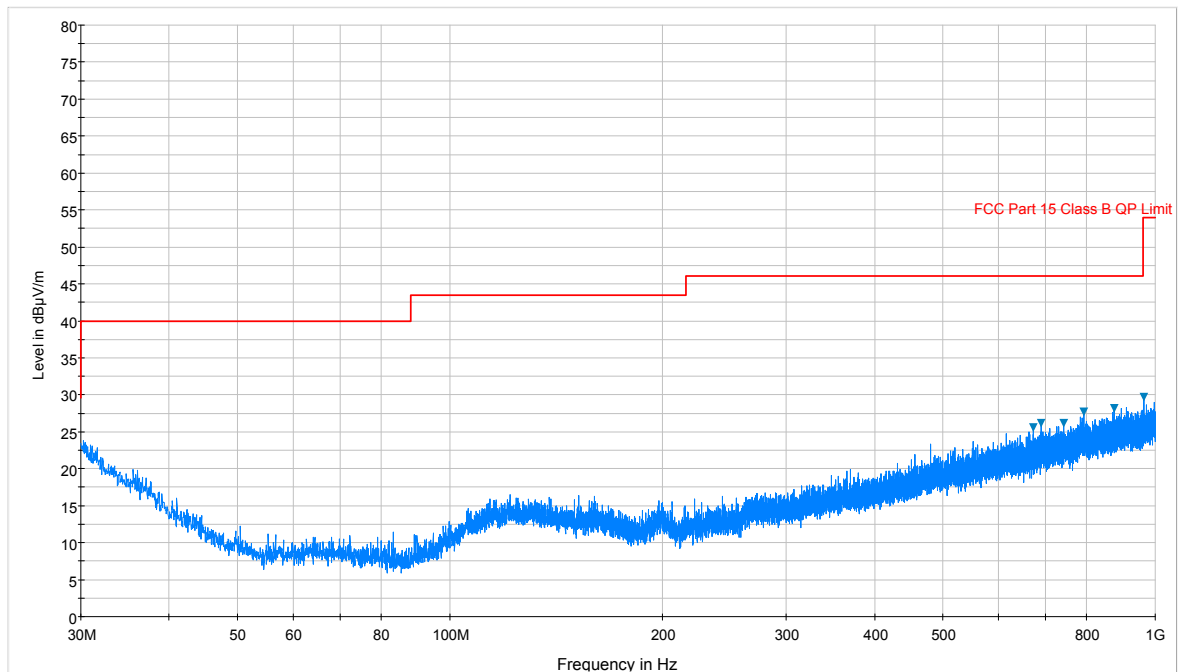
Plot 7-53. Radiated Spurious Plot below 1GHz (Pol. V)
