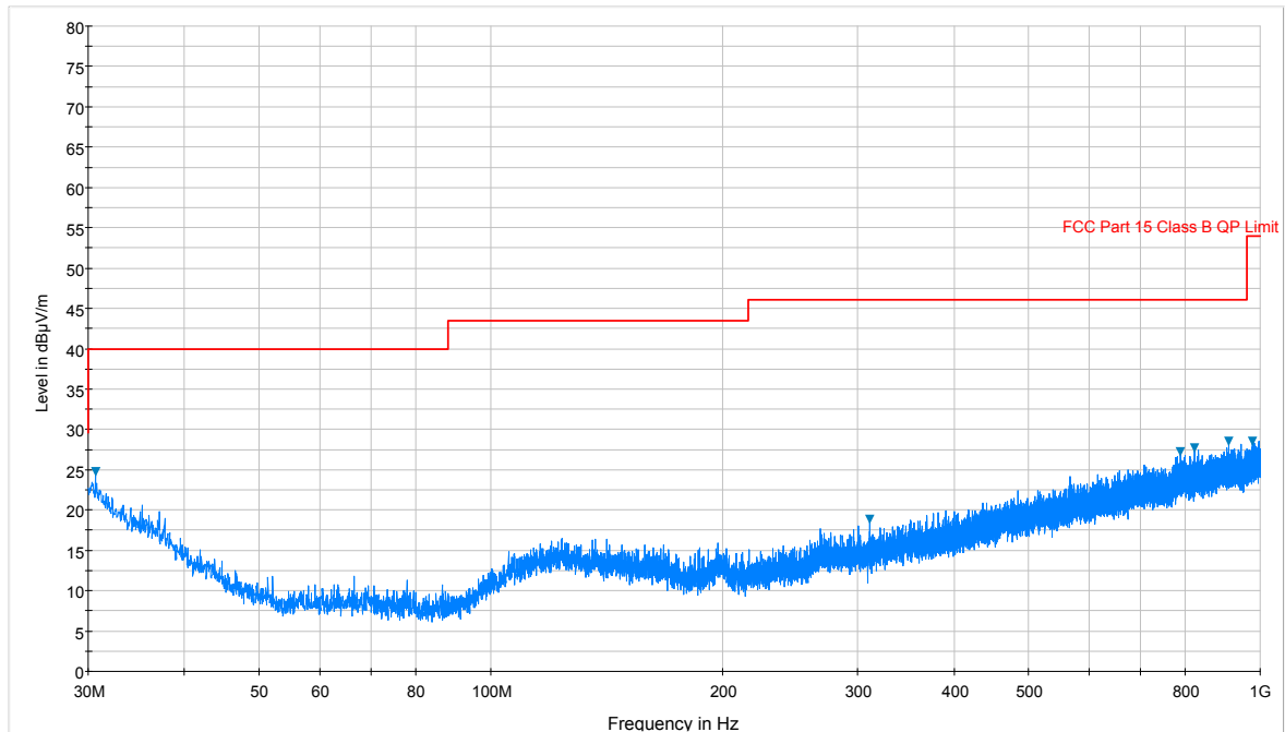
Plot 7-52. Radiated Spurious Plot below 1GHz (Pol. H)
