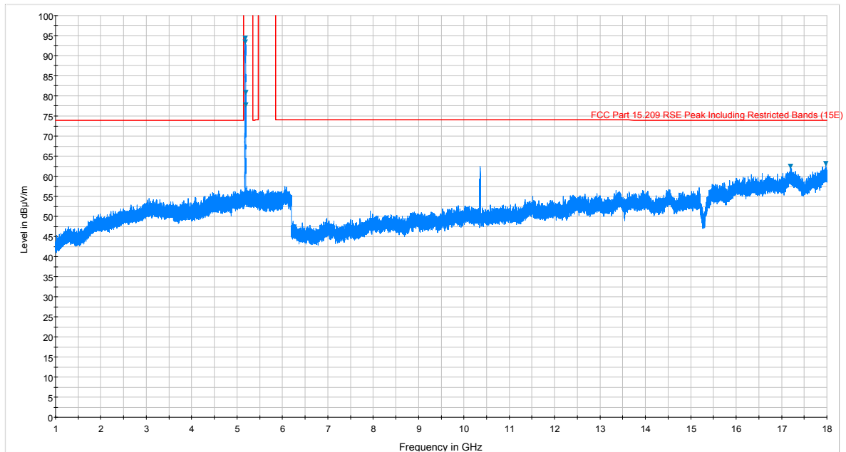
Plot 7-75. Radiated Spurious Plot above 1GHz (802.11a – U1 Ch. 40, Ant. Pol. H)
