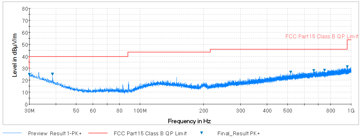
Plot 7-47. Radiated Spurious Plot below 1GHz (Pol. H)
