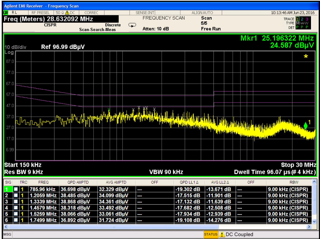
Plot 7-50. Line Conducted Plot with 802.11b (N)
