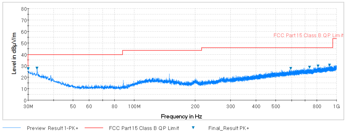
Plot 7-48. Radiated Spurious Plot below 1GHz (Pol. V)
