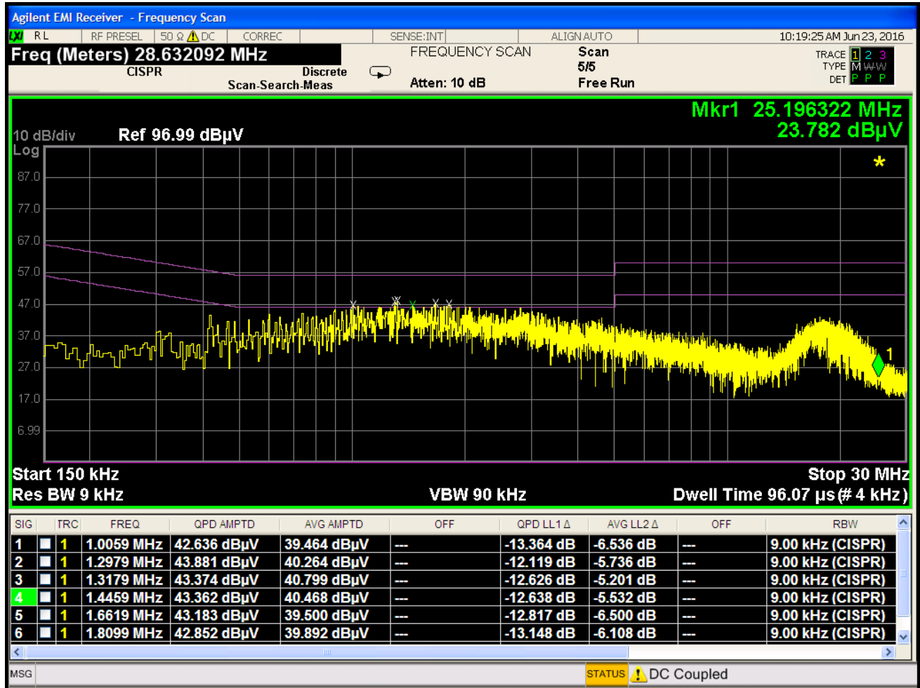
Plot 7-49. Line Conducted Plot with 802.11b (L1)
