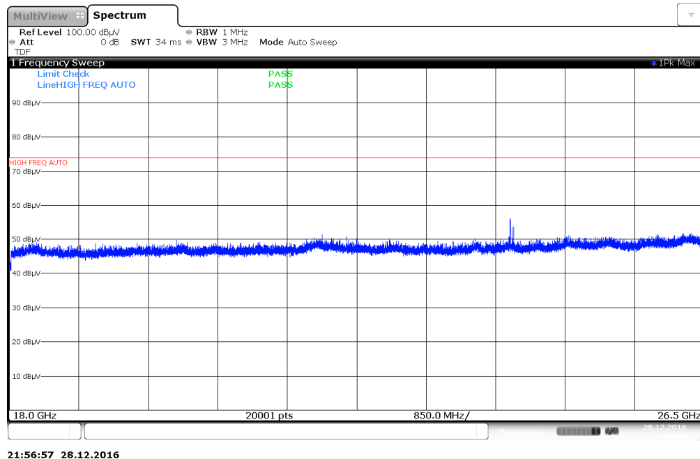
Plot 7-40. Radiated Spurious Plot above 18GHz (Pol. V)
