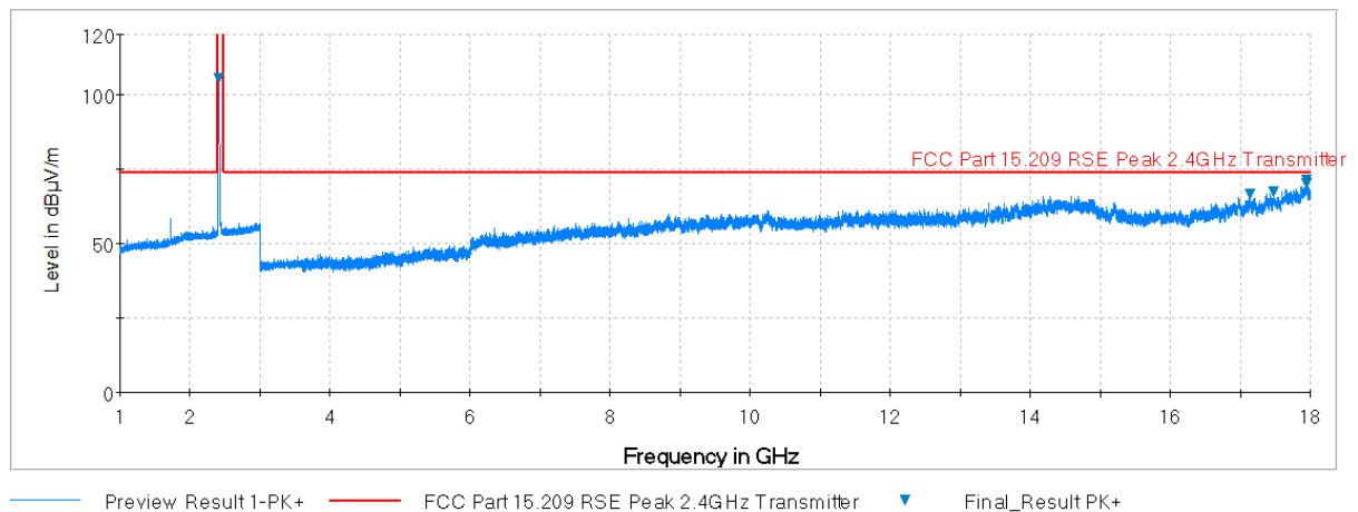
Plot 7-34. Radiated Spurious Plot above 1GHz (802.11b – Ch. 1, Ant. Pol. V)
