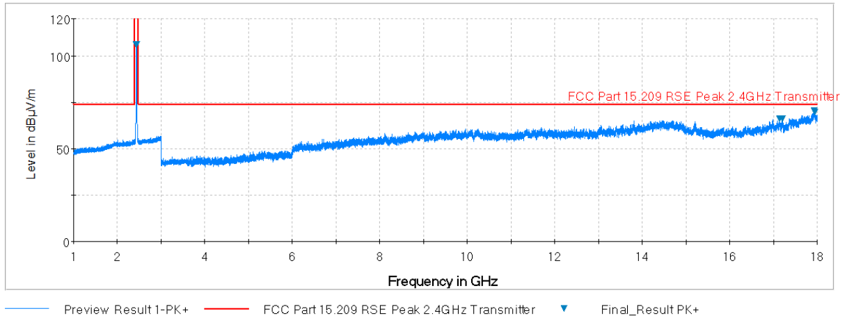
Plot 7-36. Radiated Spurious Plot above 1GHz (802.11b – Ch. 6, Ant. Pol. V)
