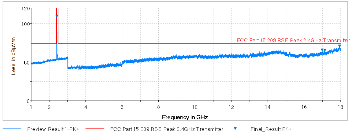
Plot 7-33. Radiated Spurious Plot above 1GHz (802.11b – Ch. 1, Ant. Pol. H)
