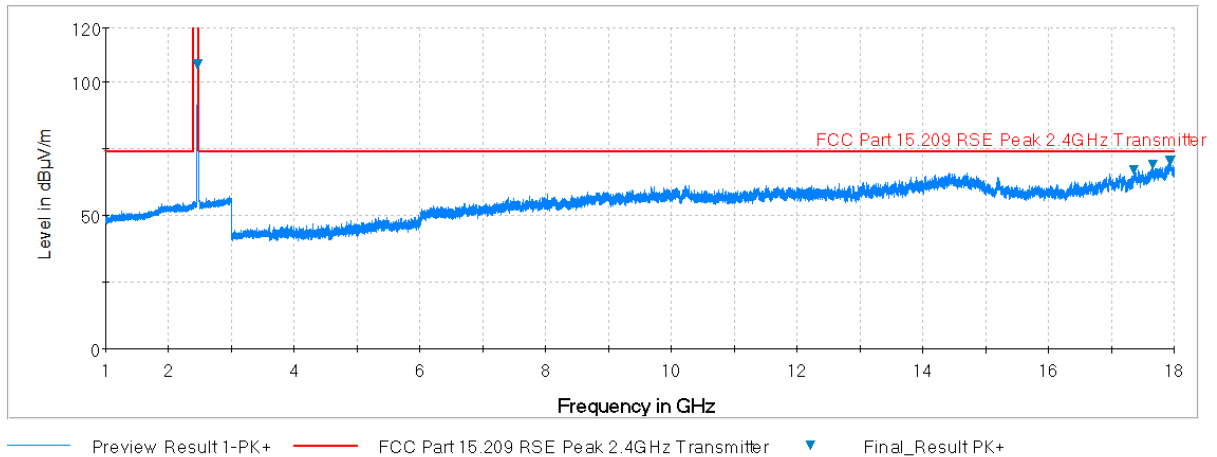
Plot 7-38. Radiated Spurious Plot above 1GHz (802.11b – Ch. 11, Ant. Pol. V)
