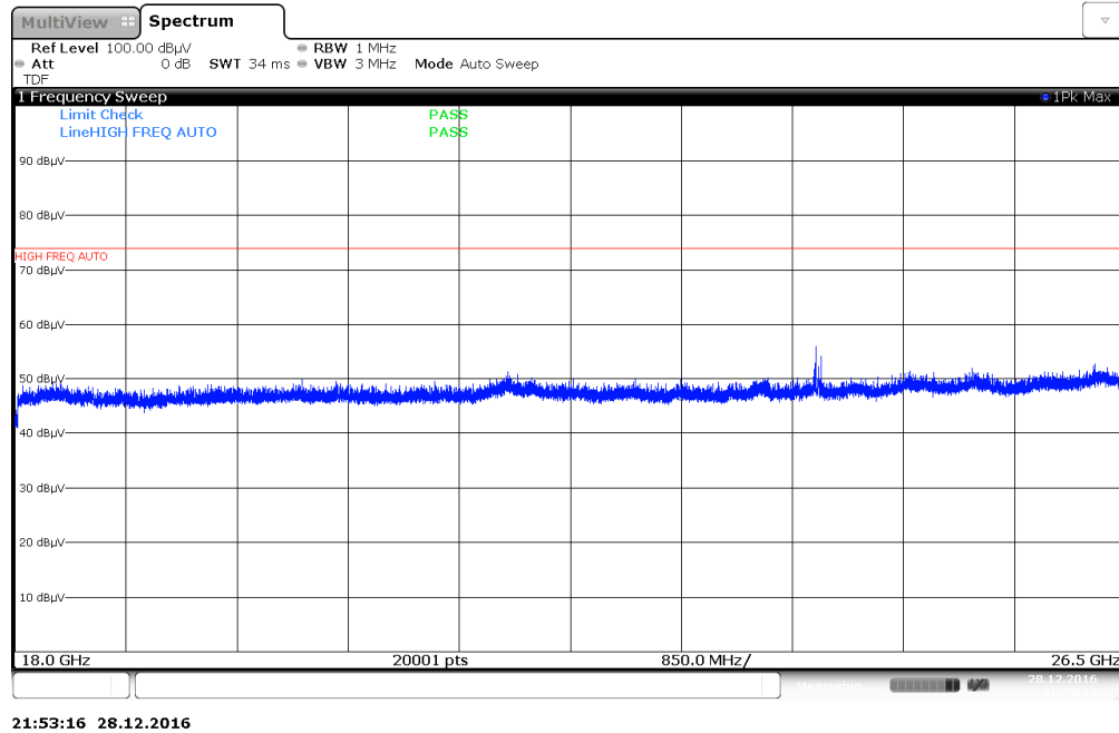
Plot 7-39. Radiated Spurious Plot above 18GHz (Pol. H)
