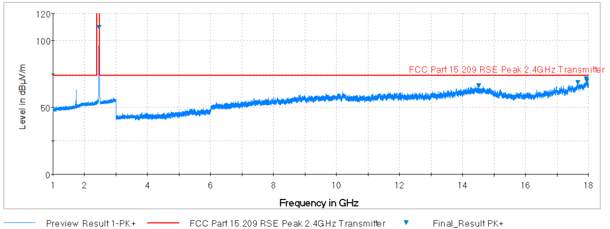
Plot 7-37. Radiated Spurious Plot above 1GHz (802.11b – Ch. 11, Ant. Pol. H)
