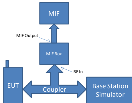
Figure 7-1 MIF Measurement Setup for licensed modes
