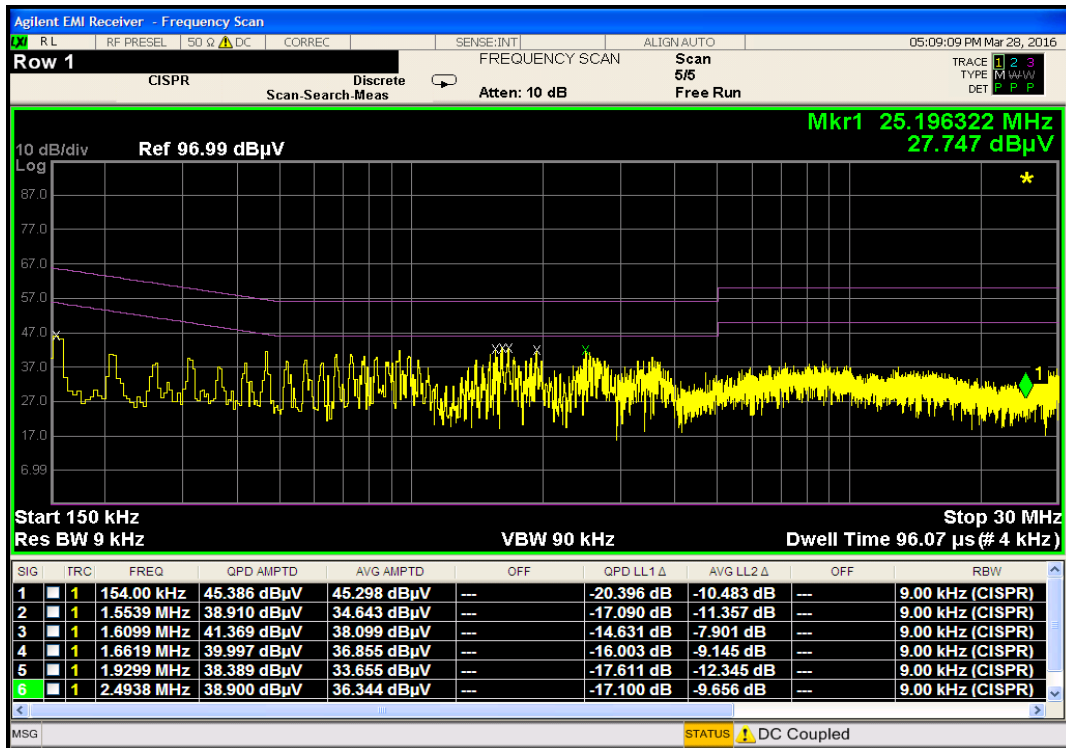
Plot 7-54. Line-Conducted Test Plot (L1)
