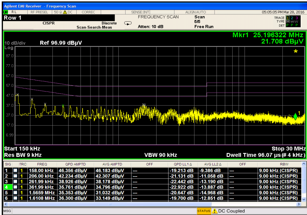
Plot 7-55. Line-Conducted Test Plot (N)
