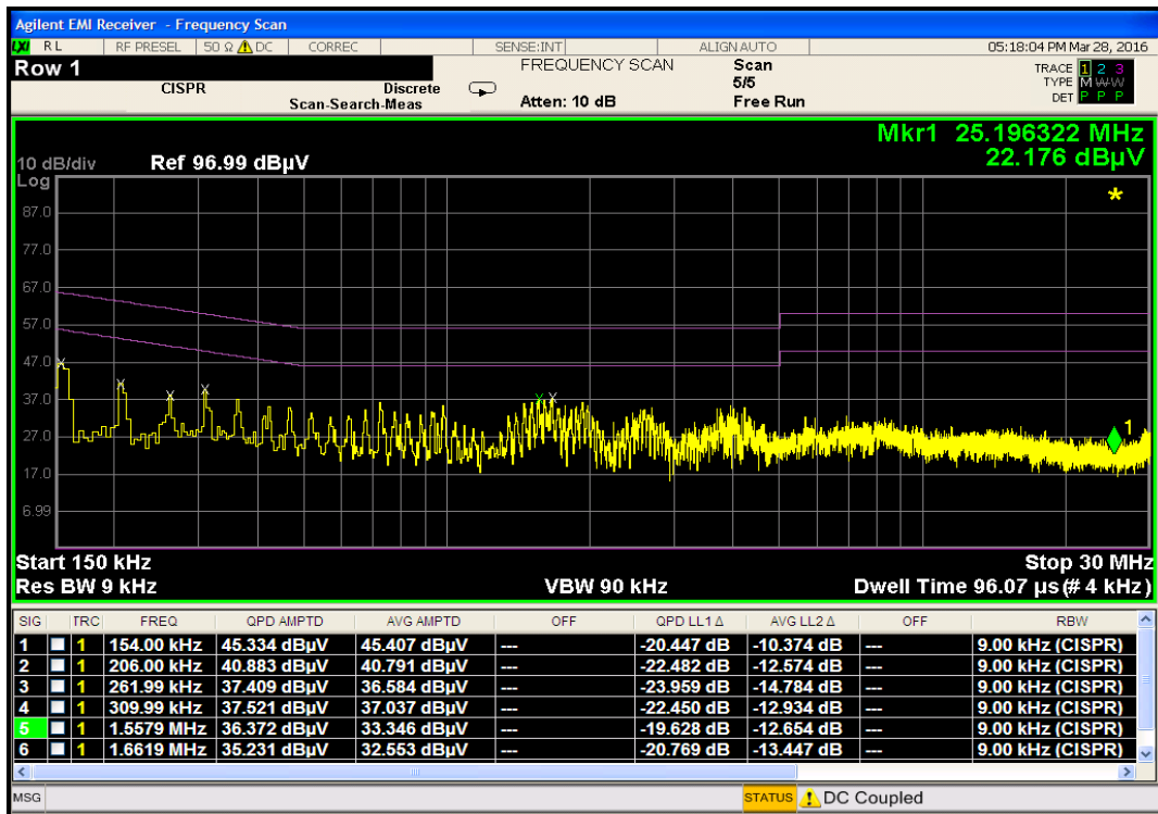
Plot 7-52. Line Conducted Plot with 802.11b (N)
