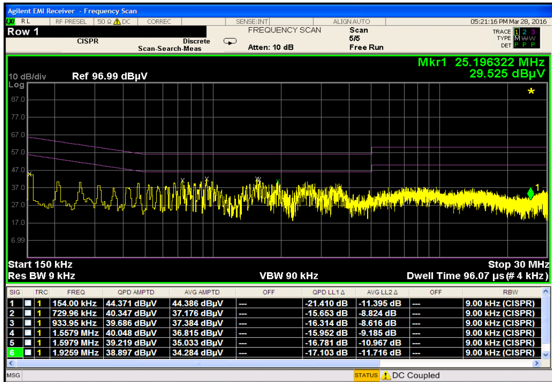
Plot 7-51. Line Conducted Plot with 802.11b (L1)
