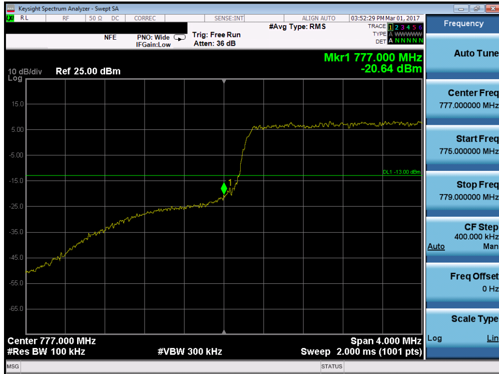
Plot 7-99. Lower Band Edge Plot (Band 13 - 5.0MHz QPSK - RB Size 25)
