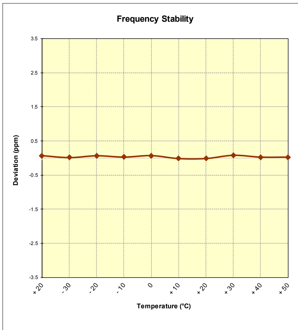
Figure 7-12. Frequency Stability Graph (Band 25)
