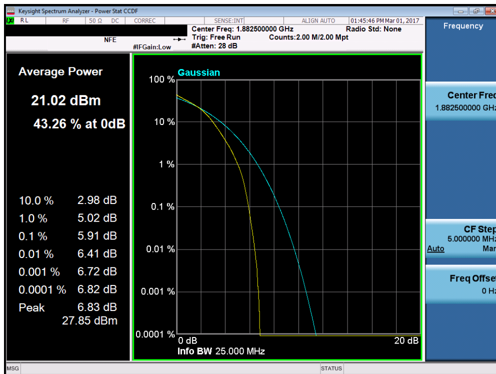
Plot 7-174. PAR Plot (Band 25 – 20.0MHz 16-QAM – RB Size 100)
