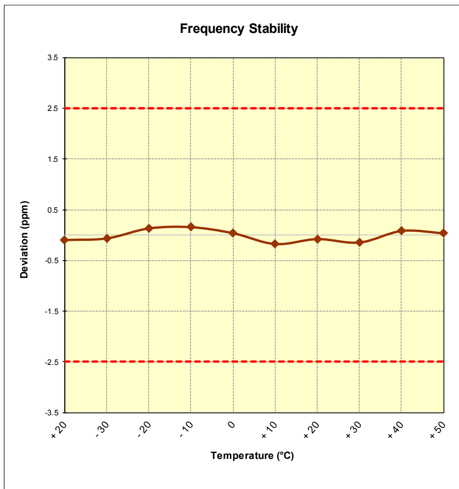
Figure 7-9. Frequency Stability Graph (Band 13)
