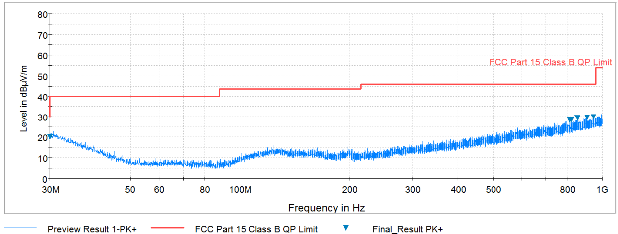
Plot 7-97. Radiated Spurious Plot below 1GHz (802.11a – U3 Ch. 157, Ant. Pol. H)
