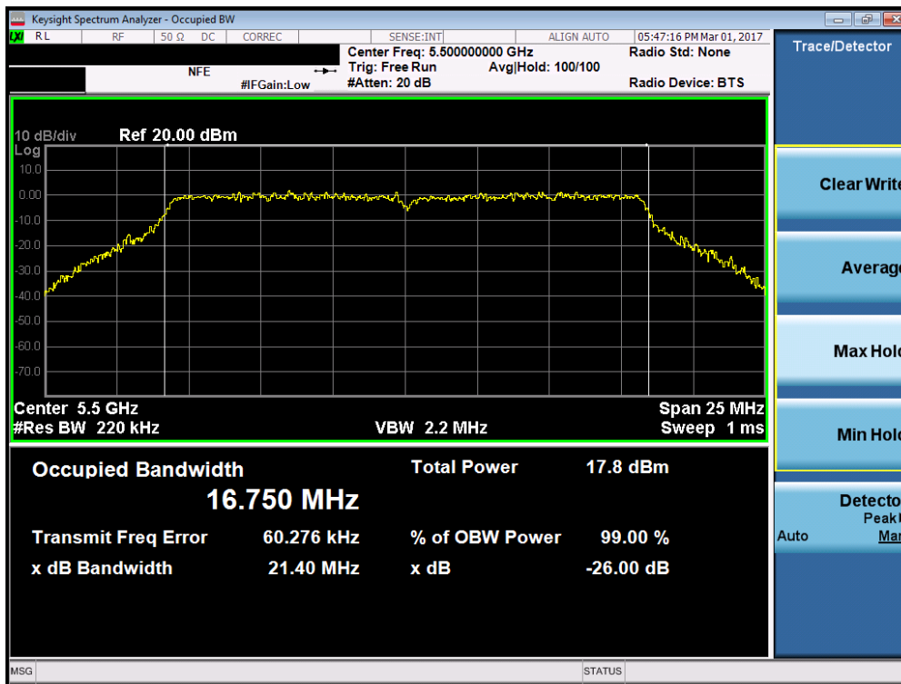
Plot 7-17. 26dB Bandwidth Plot (802.11a (UNII Band 2C) – Ch. 100)
