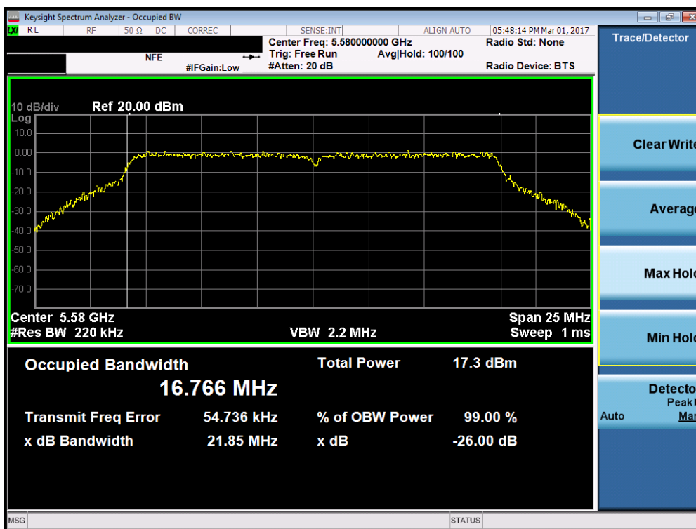
Plot 7-18. 26dB Bandwidth Plot (802.11a (UNII Band 2C) – Ch. 116)
