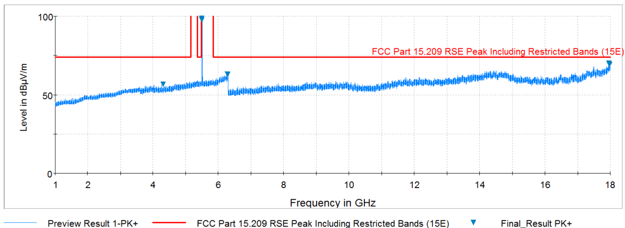
Plot 7-72. Radiated Spurious Plot above 1GHz (802.11a – U2C Ch. 116, Ant. Pol. V)
