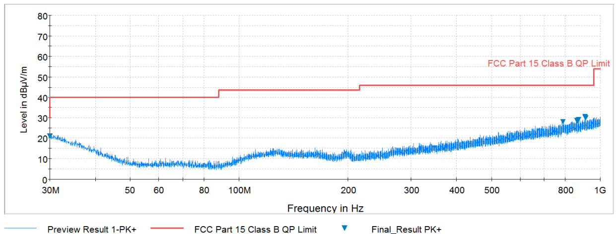
Plot 7-98. Radiated Spurious Plot below 1GHz (802.11a – U3 Ch. 157, Ant. Pol. V)
