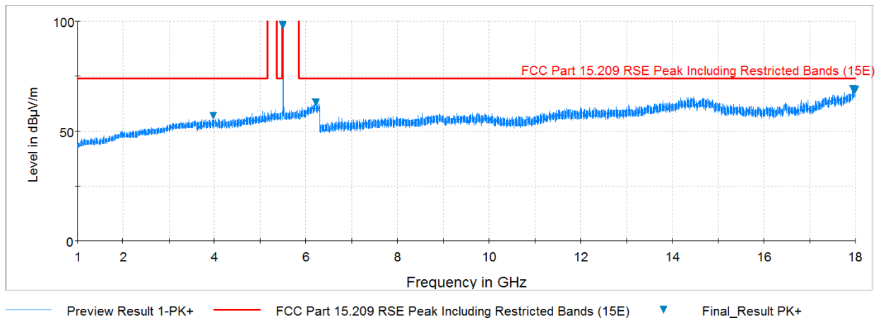
Plot 7-71. Radiated Spurious Plot above 1GHz (802.11a – U2C Ch. 116, Ant. Pol. H)
