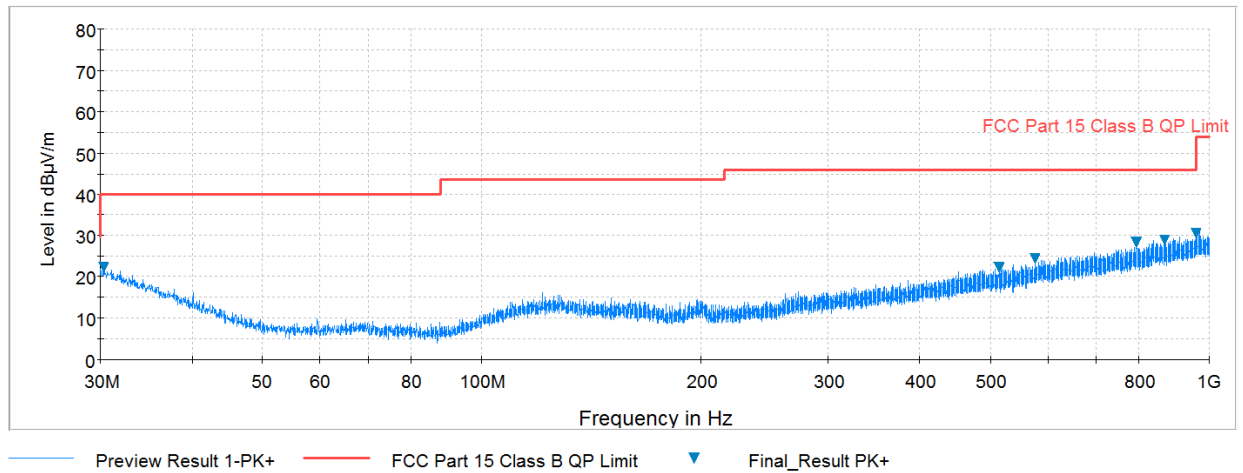
Plot 7-43. Radiated Spurious Plot below 1GHz (Pol. H)
