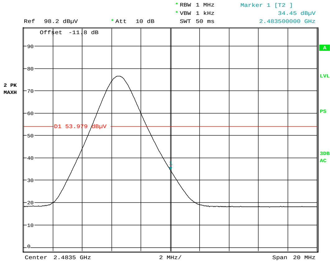
Plot 6-45. Radiated Restricted Upper Band Edge Measurement with WCC (Peak)
