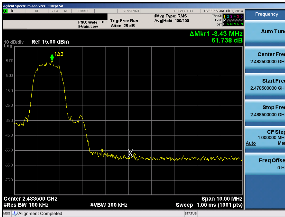
Plot 6-29. Band Edge Plot (Bluetooth with Hopping Disabled, 3 Mbps – Ch. 78)
