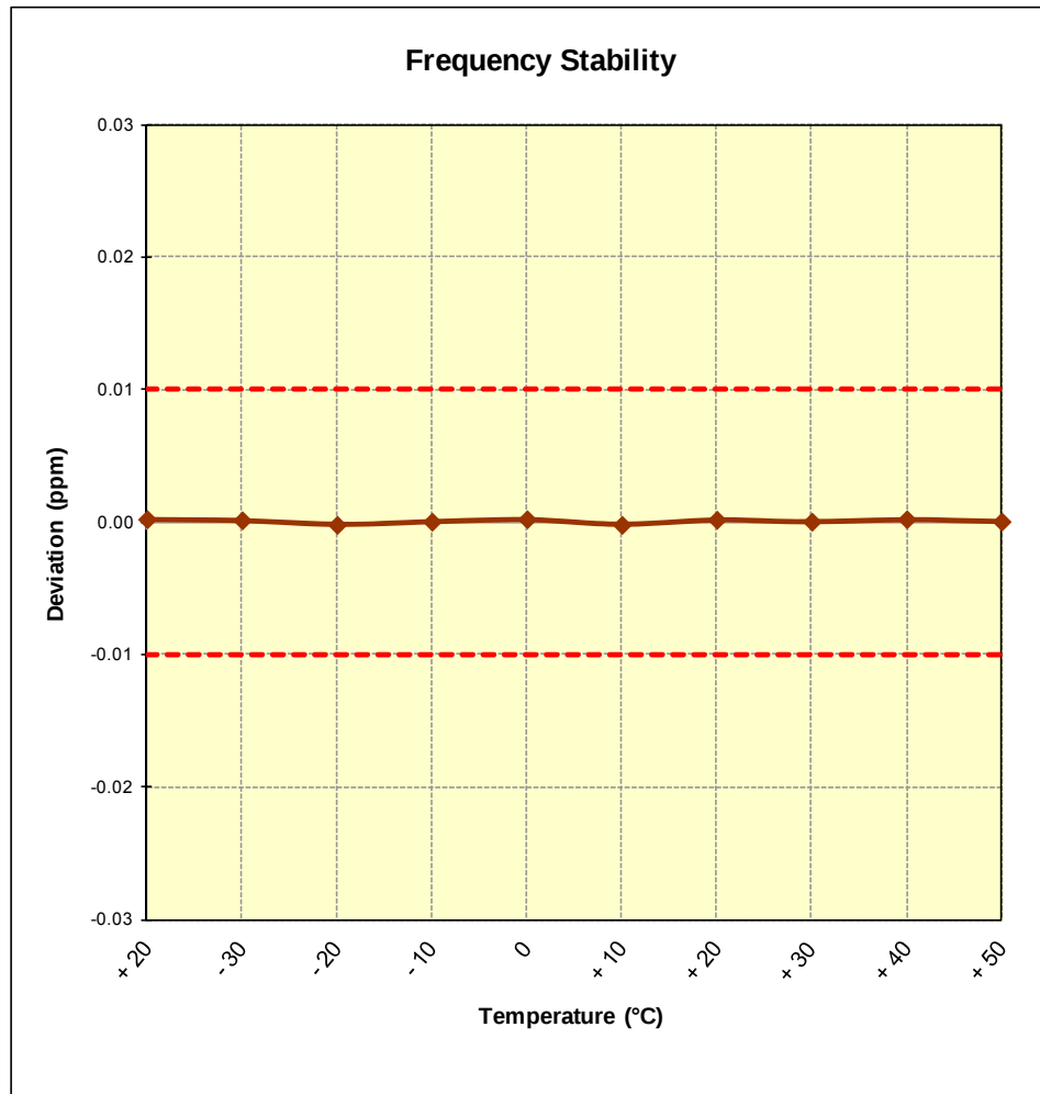
Figure 8-4. Frequency Stability Plot
