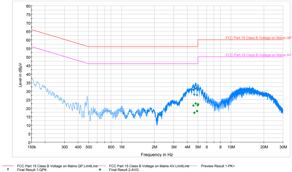
Plot 6-38. Line Conducted Plot with 802.11b (N)
