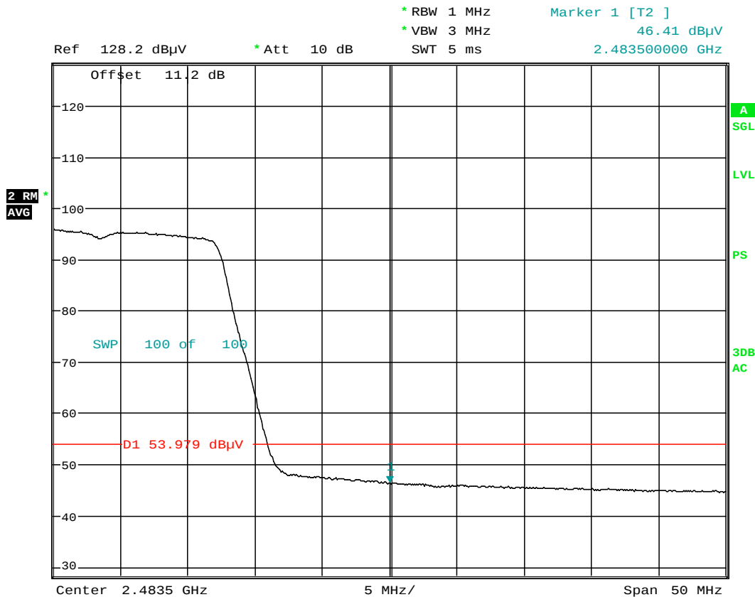
Plot 6-35. Radiated Restricted Band Edge Measurement with WCC (Average)
