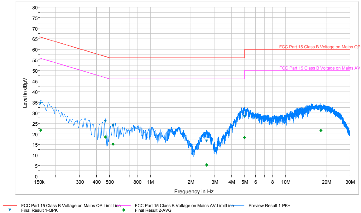
Plot 6-37. Line Conducted Plot with 802.11b (L1)
