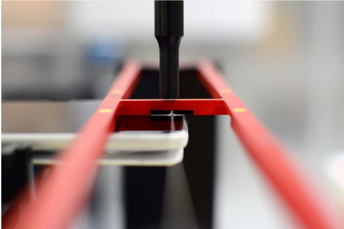
Figure 18-5 HAC Phantom Plane Alignment (Wireless Charging Cover – Open)
