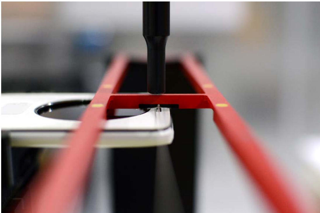
Figure 18-6 HAC Phantom Plane Alignment (Wireless Charging Cover – Closed)
