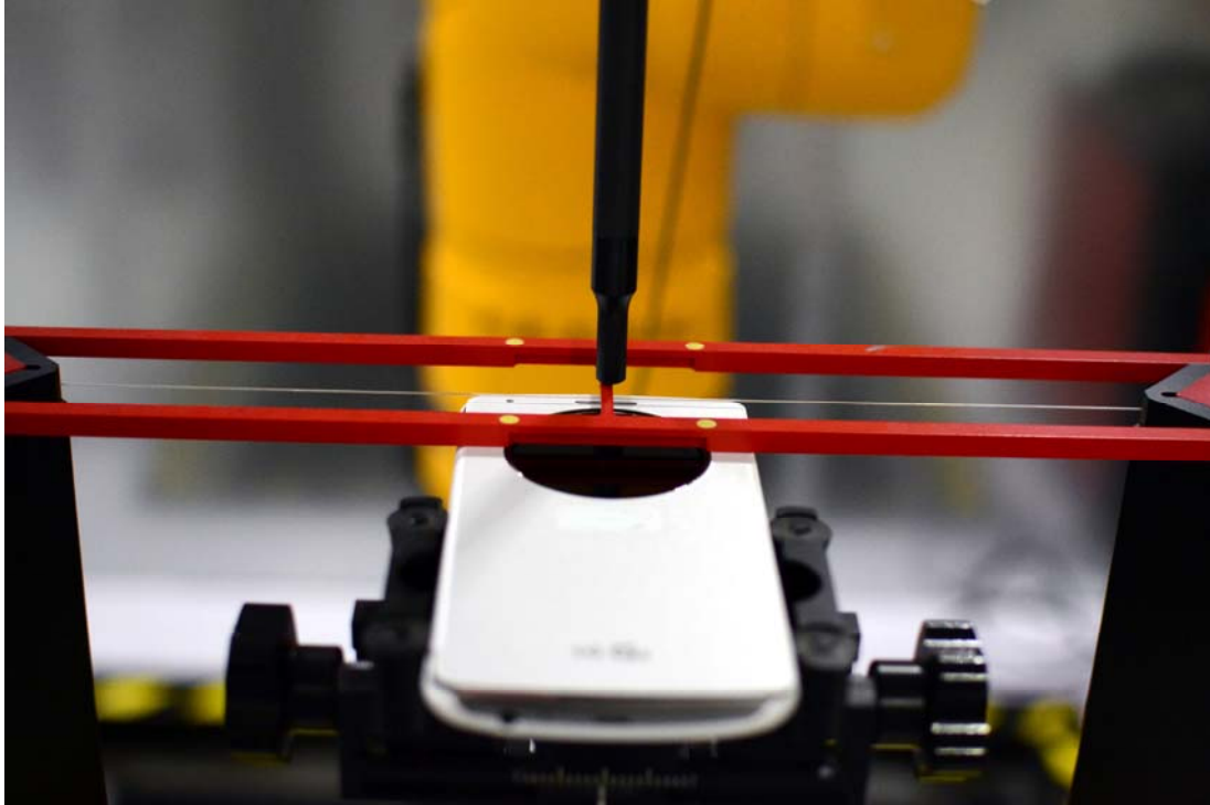
Figure 18-3 Ear Reference Point HAC Phantom Alignment (Wireless Charging Cover - Closed)
