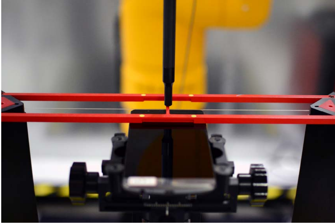
Figure 18-1 Ear Reference Point HAC Phantom Alignment (Standard Battery Cover)
