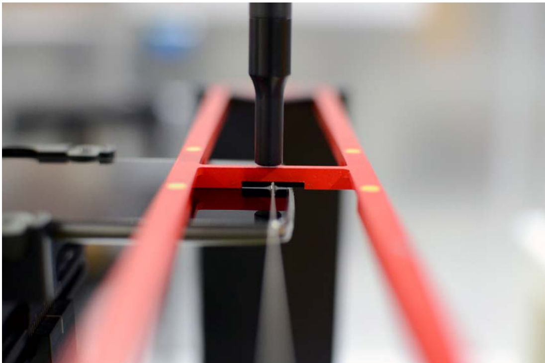
Figure 18-4 HAC Phantom Plane Alignment (Standard Battery Cover)
