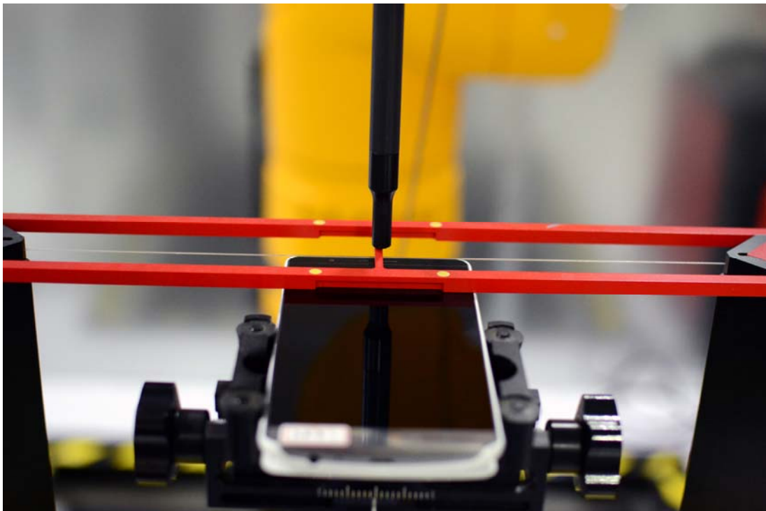
Figure 18-2 Ear Reference Point HAC Phantom Alignment (Wireless Charging Cover - Open)
