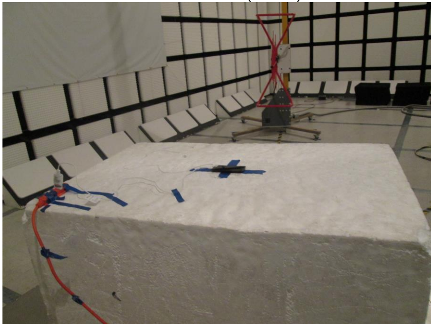
RADIATED EMISSIONS ABOVE 30 MHz (FRONT)
