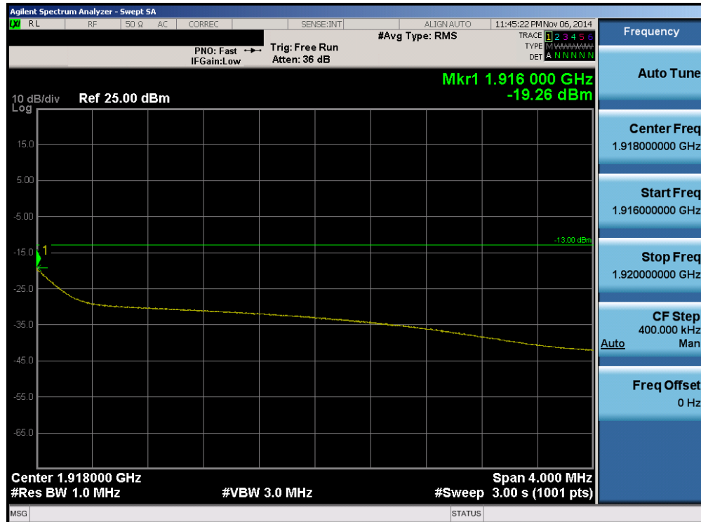
Plot 6-128. Upper Extended Band Edge Plot (Band 25 - 5.0MHz QPSK - RB Size 25)
