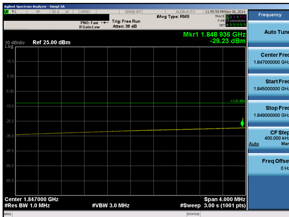
Plot 6-134. Lower Extended Band Edge Plot (Band 25 – 15.0MHz QPSK – RB Size 75)
