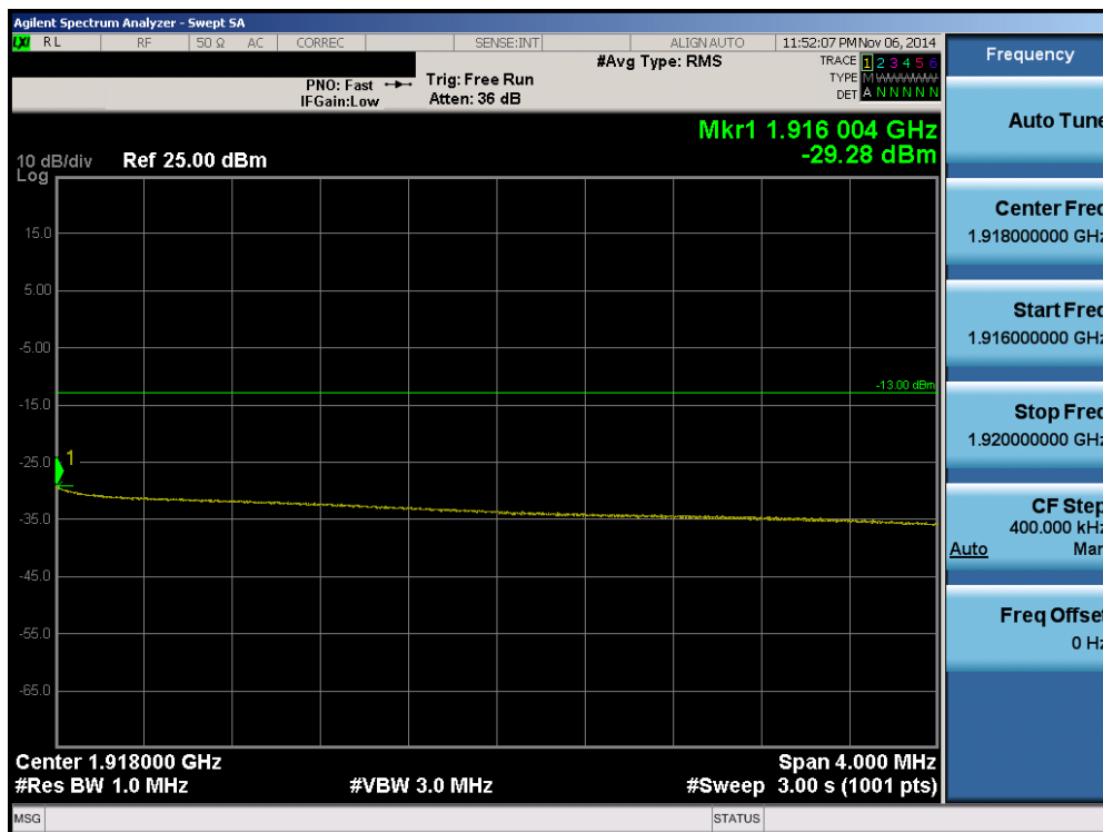
Plot 6-132. Upper Extended Band Edge Plot (Band 25 – 10.0MHz QPSK – RB Size 50)
