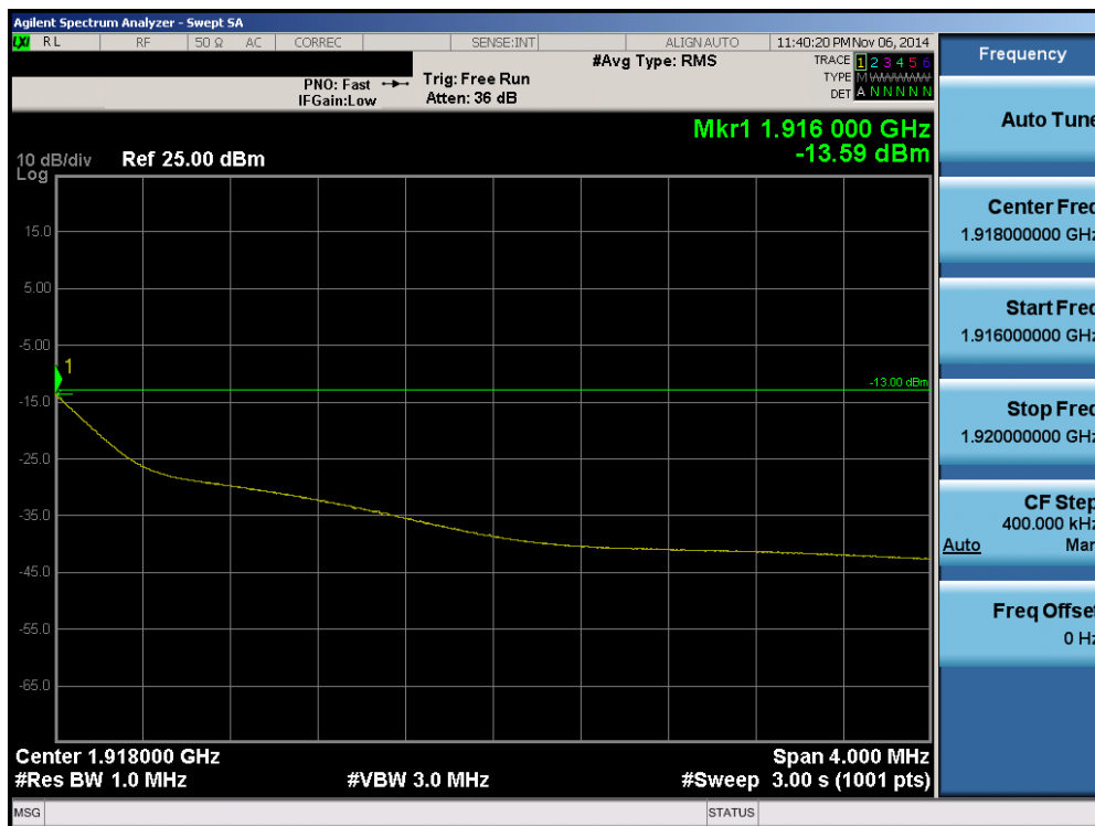
Plot 6-124. Upper Extended Band Edge Plot (Band 25 – 3.0MHz QPSK – RB Size 15)
