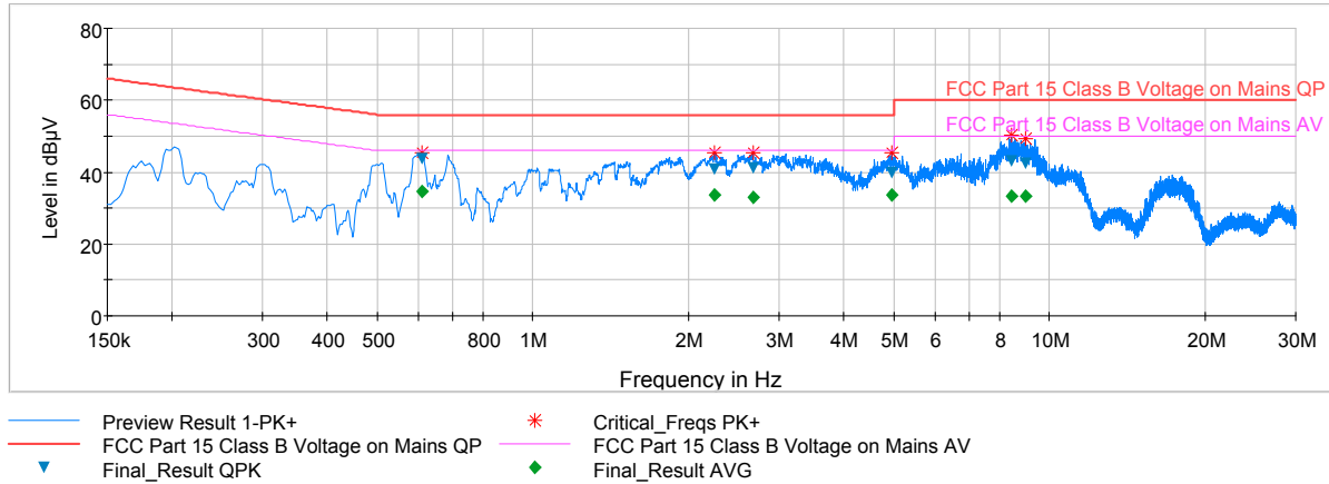
Plot 6-45. Line-Conducted Test Plot (N)
