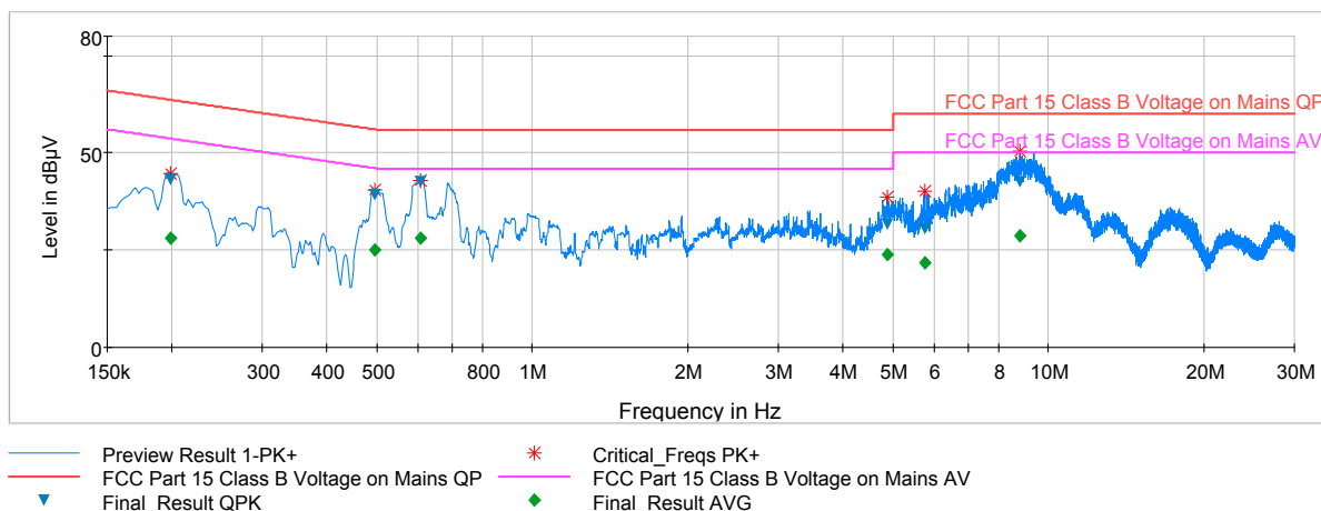
Plot 6-44. Line-Conducted Test Plot (L1)
