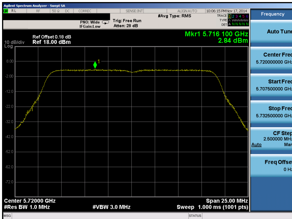
Plot 6-66. Peak Power Spectral Density Plot (20MHz BW 802.11n (UNII Band 2C) – Ch. 144)
