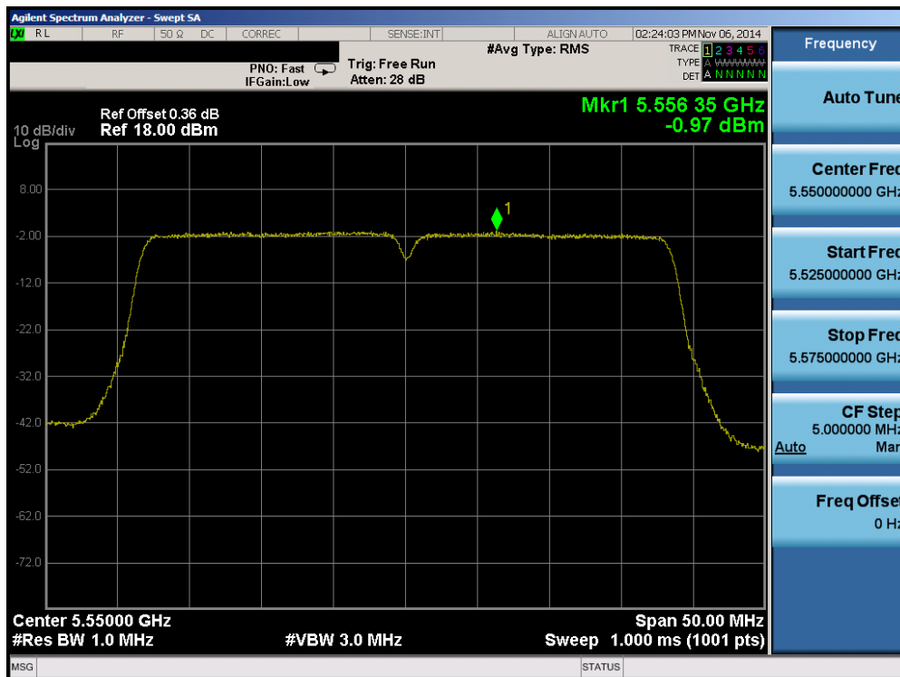
Plot 6-68. Peak Power Spectral Density Plot (40MHz BW 802.11n (UNII Band 2C) – Ch. 110)
