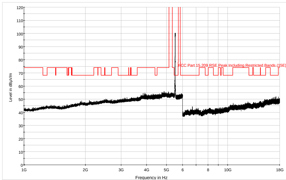
Plot 6-90. Radiated Spurious Plot above 1GHz (802.11a – Band 2C, Ch. 100 Ant. Pol. H)
