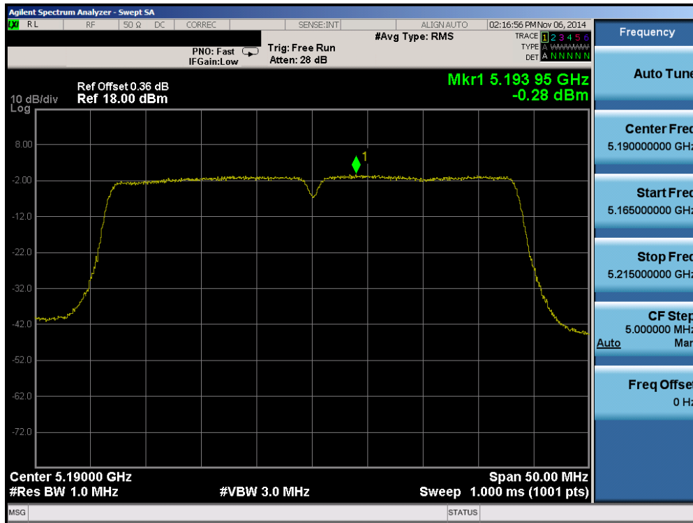
Plot 6-49. Peak Power Spectral Density Plot (40MHz BW 802.11n (UNII Band 1) – Ch. 38)
