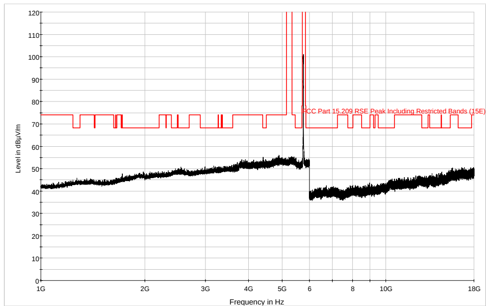
Plot 6-96. Radiated Spurious Plot above 1GHz (802.11a – Band 3, Ch. 149 Ant. Pol. V)
