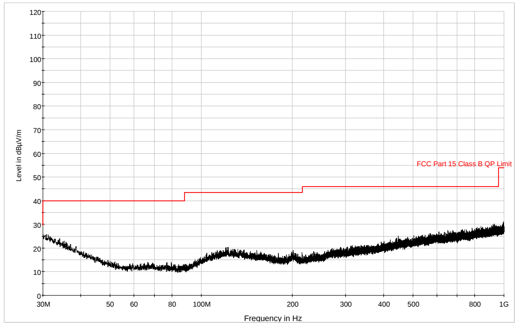
Plot 6-85. Radiated Spurious Plot below 1GHz (802.11a – Band 2A, Ch. 52 Ant. Pol. H)
