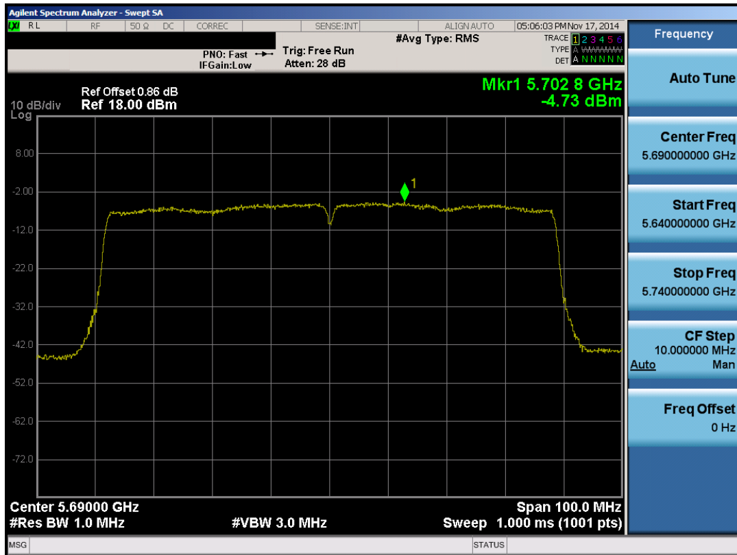
Plot 6-71. Peak Power Spectral Density Plot (80MHz BW 802.11ac (UNII Band 2C) – Ch. 138)
