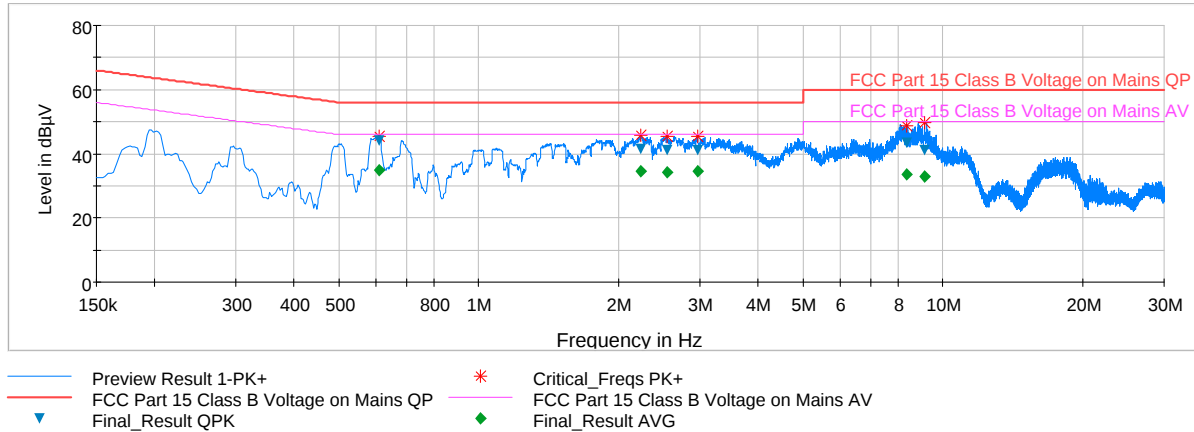
Plot 6-123. Line Conducted Plot with 802.11a UNII Band 2C (N)
