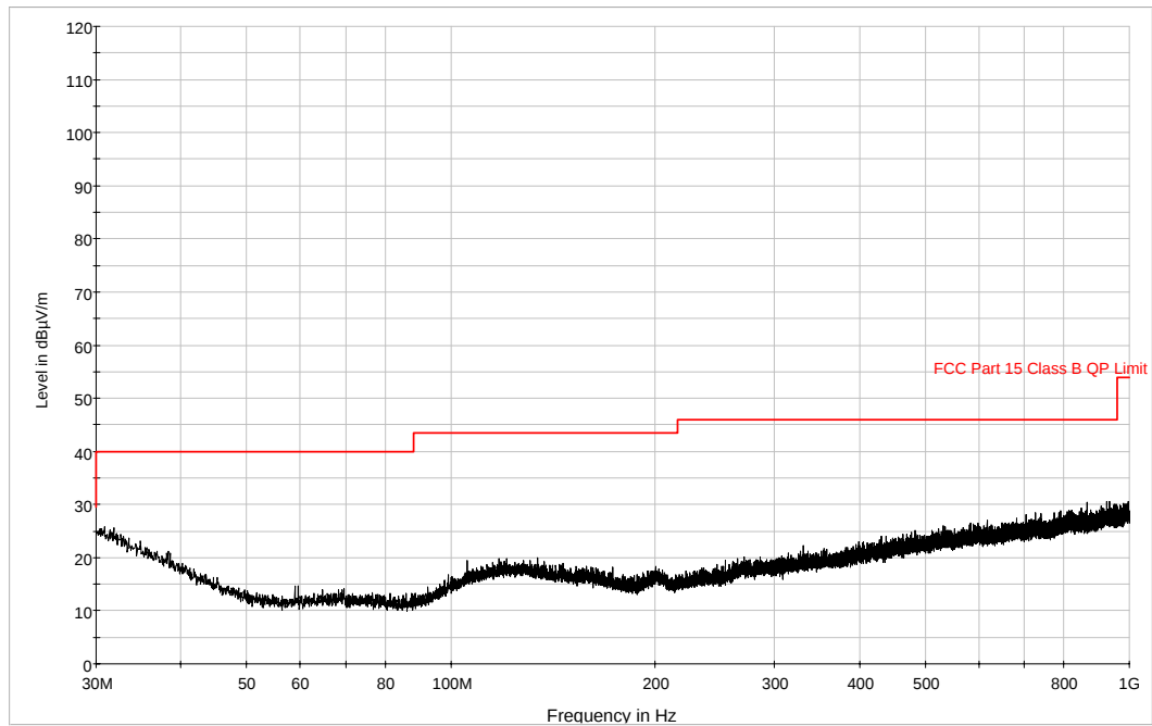
Plot 6-87. Radiated Spurious Plot below 1GHz (802.11a – Band 2A, Ch. 52 Ant. Pol. V)
