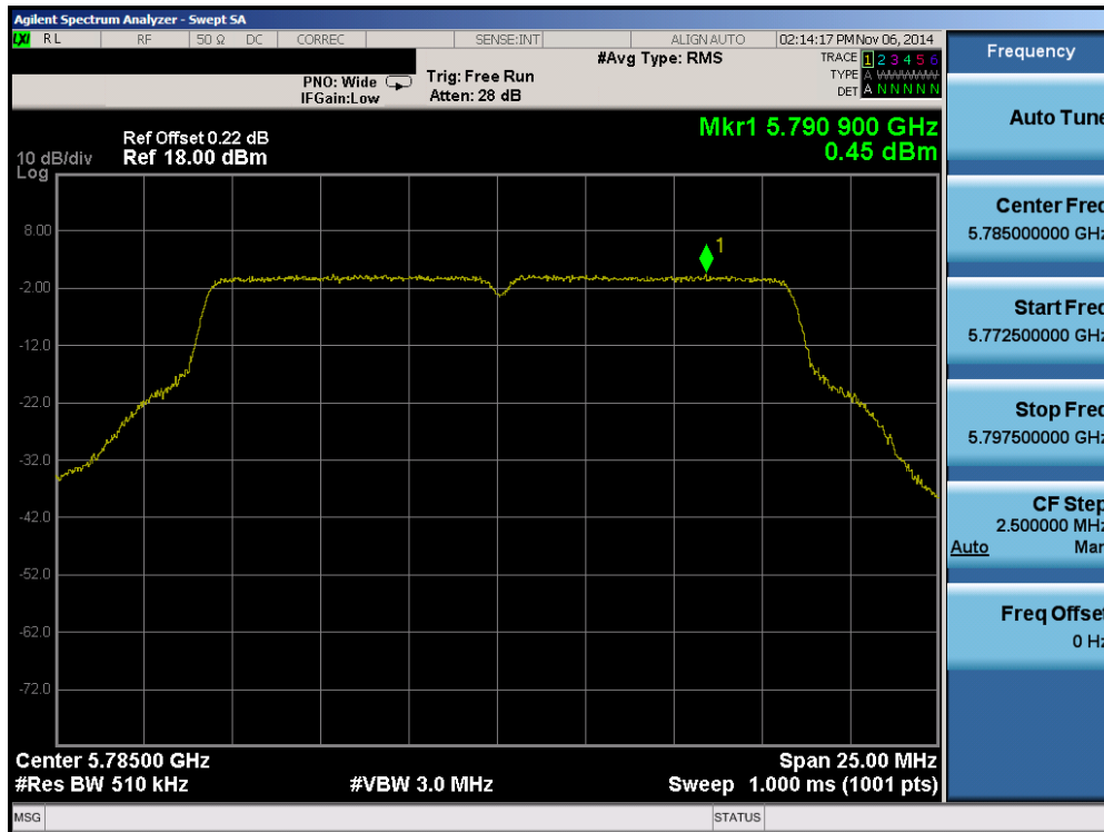
Plot 6-73. Peak Power Spectral Density Plot (802.11a (UNII Band 3) – Ch. 157)
