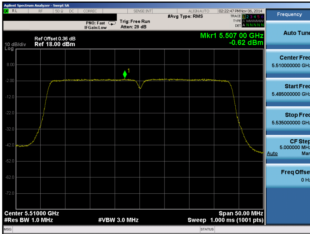
Plot 6-67. Peak Power Spectral Density Plot (40MHz BW 802.11n (UNII Band 2C) – Ch. 102)
