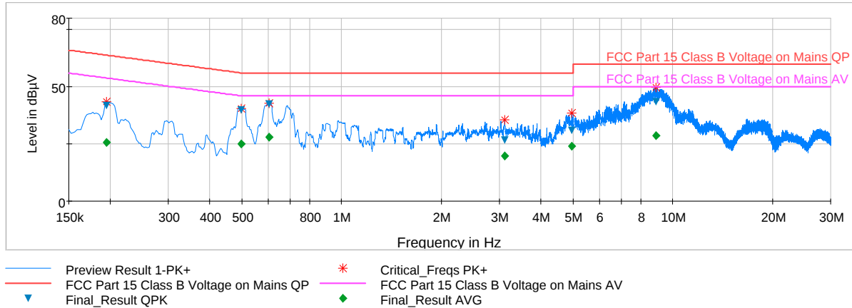
Plot 6-122. Line Conducted Plot with 802.11a UNII Band 2C (L1)
