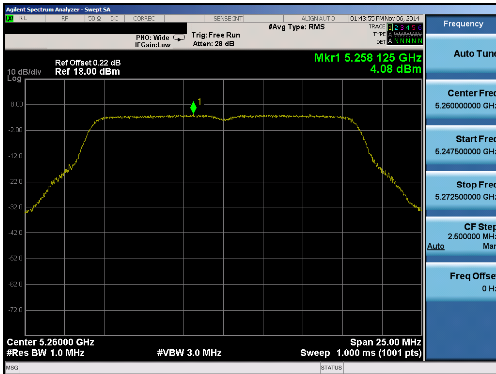
Plot 6-52. Peak Power Spectral Density Plot (802.11a (UNII Band 2A) – Ch. 52)
