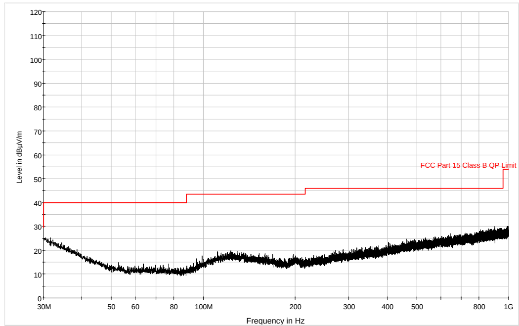
Plot 6-93. Radiated Spurious Plot below 1GHz (802.11a – Band 3, Ch. 149 Ant. Pol. H)
