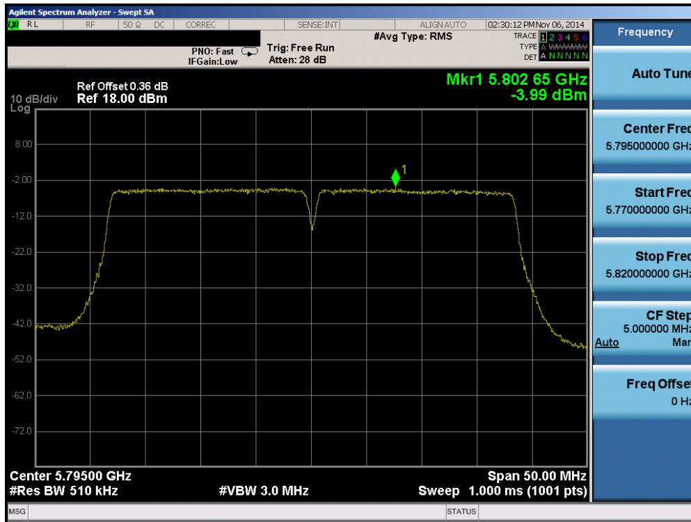
Plot 6-79. Peak Power Spectral Density Plot (40MHz BW 802.11n (UNII Band 3) – Ch. 159)
