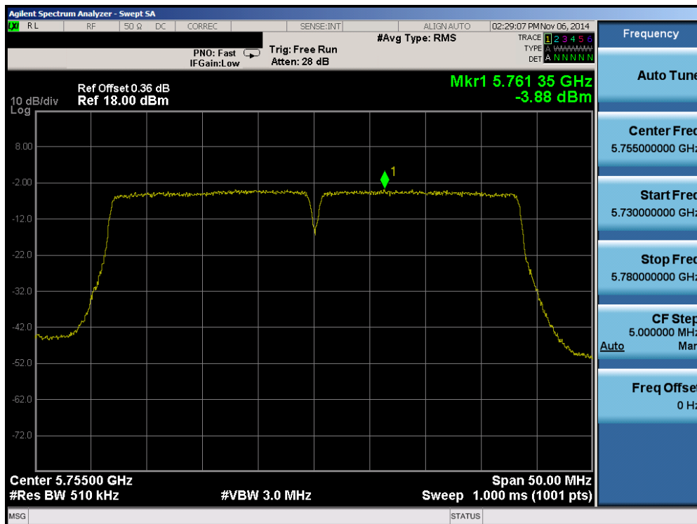
Plot 6-78. Peak Power Spectral Density Plot (40MHz BW 802.11n (UNII Band 3) – Ch. 151)
