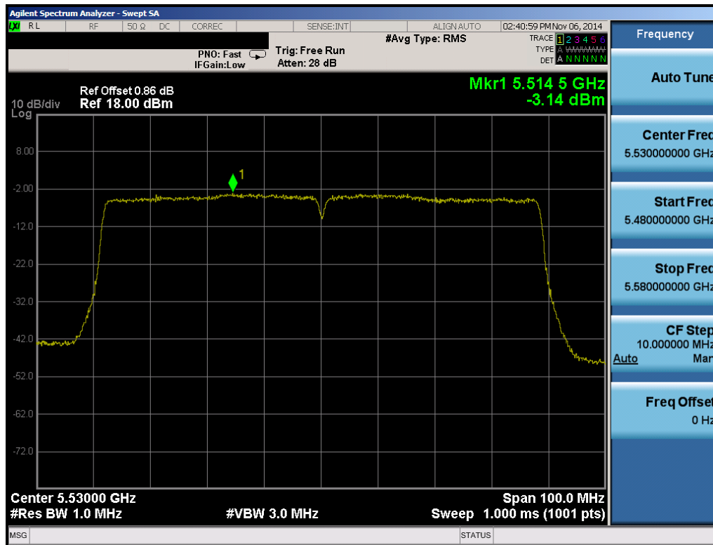
Plot 6-70. Peak Power Spectral Density Plot (80MHz BW 802.11ac (UNII Band 2C) – Ch. 106)
