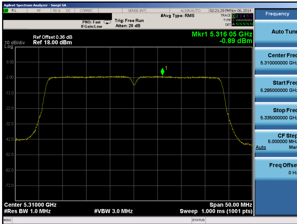
Plot 6-59. Peak Power Spectral Density Plot (40MHz BW 802.11n (UNII Band 2A) – Ch. 62)
