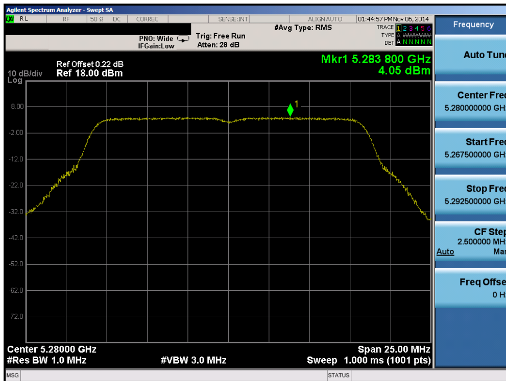
Plot 6-53. Peak Power Spectral Density Plot (802.11a (UNII Band 2A) – Ch. 56)
