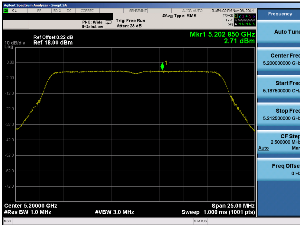
Plot 6-47. Peak Power Spectral Density Plot (20MHz BW 802.11n (UNII Band 1) – Ch. 40)
