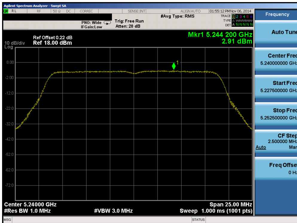
Plot 6-48. Peak Power Spectral Density Plot (20MHz BW 802.11n (UNII Band 1) – Ch. 48)
