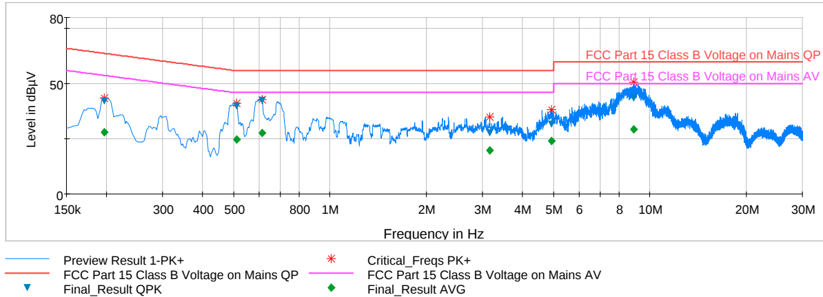
Plot 6-118. Line Conducted Plot with 802.11a UNII Band 1 (L1)
