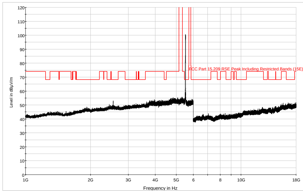
Plot 6-92. Radiated Spurious Plot above 1GHz (802.11a – Band 2C, Ch. 100 Ant. Pol. V)
