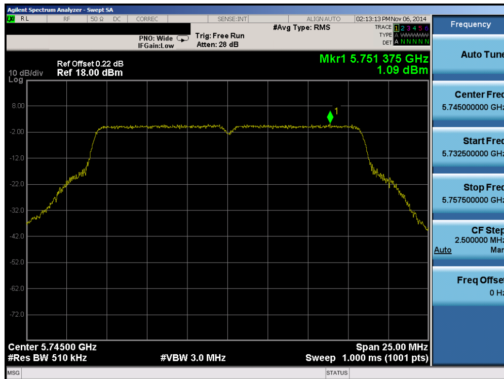
Plot 6-72. Peak Power Spectral Density Plot (802.11a (UNII Band 3) – Ch. 149)
