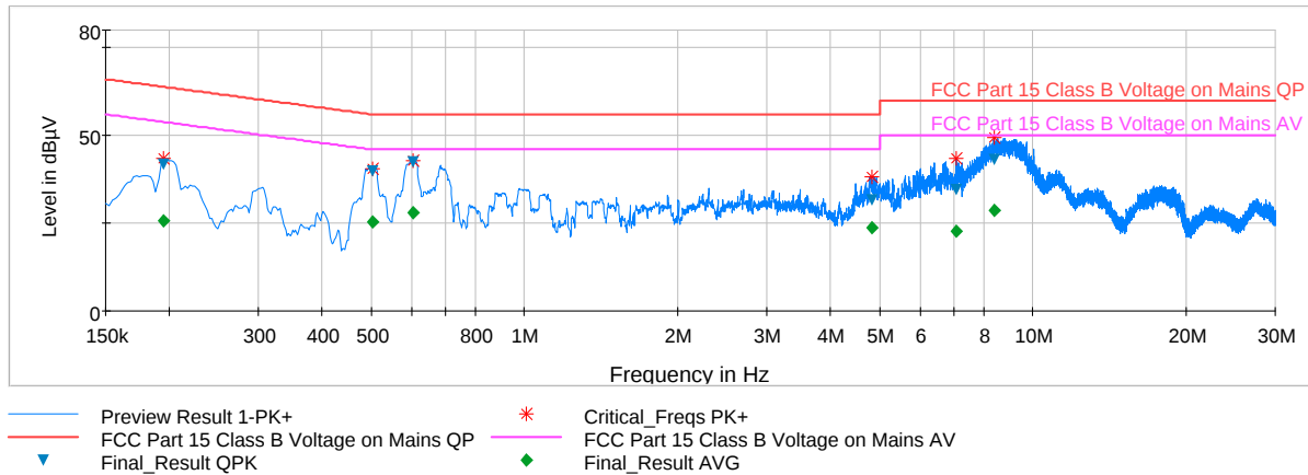
Plot 6-124. Line Conducted Plot with 802.11a UNII Band 3 (L1)
