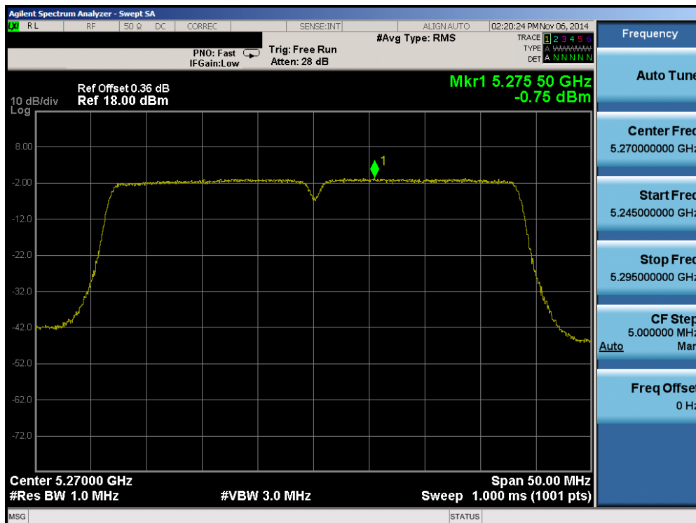
Plot 6-58. Peak Power Spectral Density Plot (40MHz BW 802.11n (UNII Band 2A) – Ch. 54)
