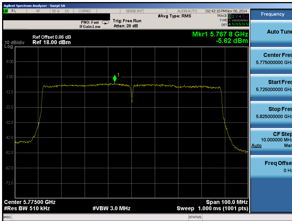
Plot 6-80. Peak Power Spectral Density Plot (80MHz BW 802.11ac (UNII Band 3) – Ch. 155)
