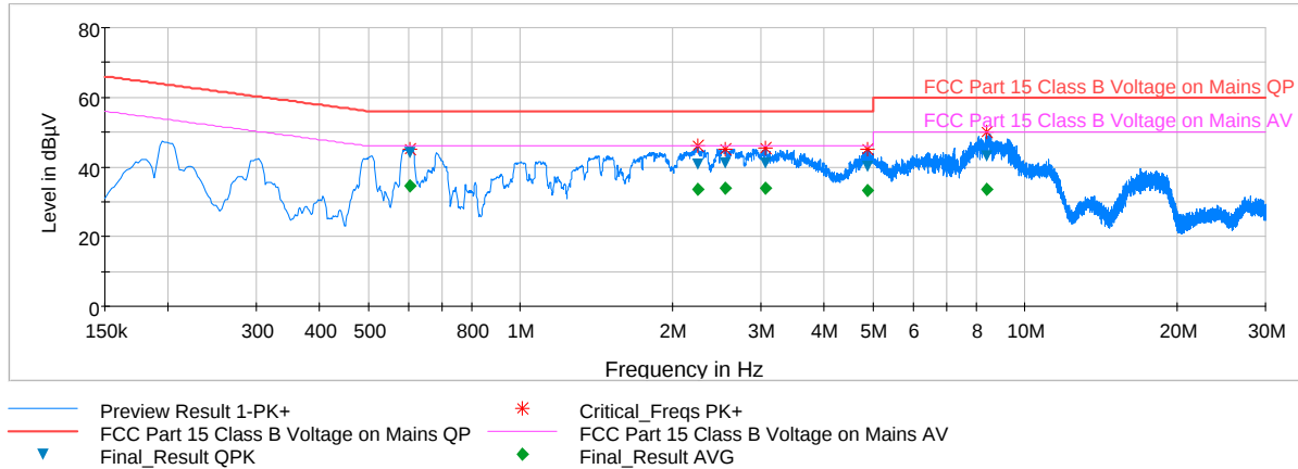
Plot 6-125. Line Conducted Plot with 802.11a UNII Band 3 (N)
