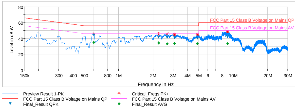
Plot 6-119. Line Conducted Plot with 802.11a UNII Band 1 (N)
