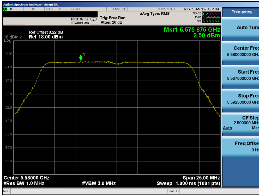
Plot 6-65. Peak Power Spectral Density Plot (20MHz BW 802.11n (UNII Band 2C) – Ch. 116)
