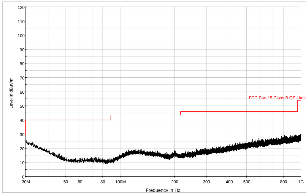
Plot 6-91. Radiated Spurious Plot below 1GHz (802.11a – Band 2C, Ch. 100 Ant. Pol. V)
