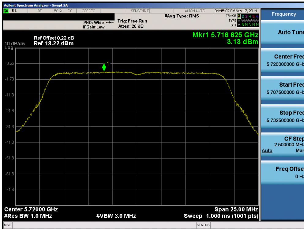
Plot 6-63. Peak Power Spectral Density Plot (802.11a (UNII Band 2C) – Ch. 144)
