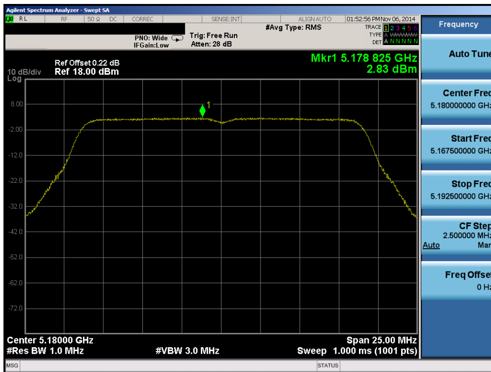
Plot 6-46. Peak Power Spectral Density Plot (20MHz BW 802.11n (UNII Band 1) – Ch. 36)
