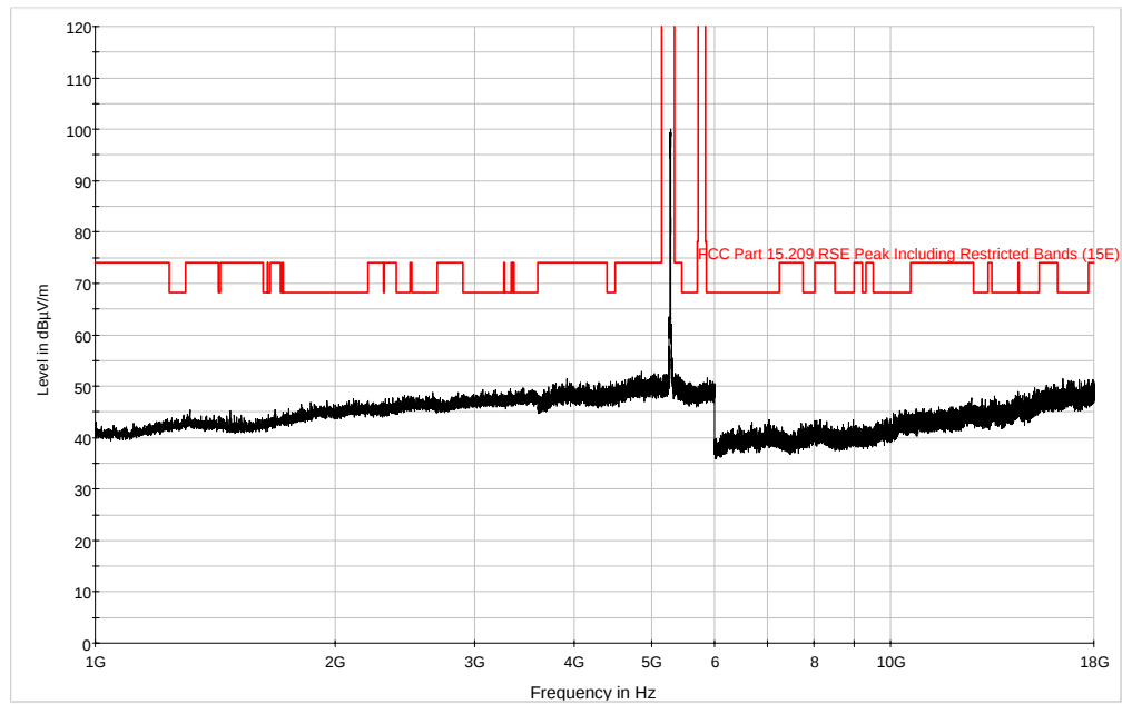
Plot 6-88. Radiated Spurious Plot above 1GHz (802.11a – Band 2A, Ch. 52 Ant. Pol. V)
