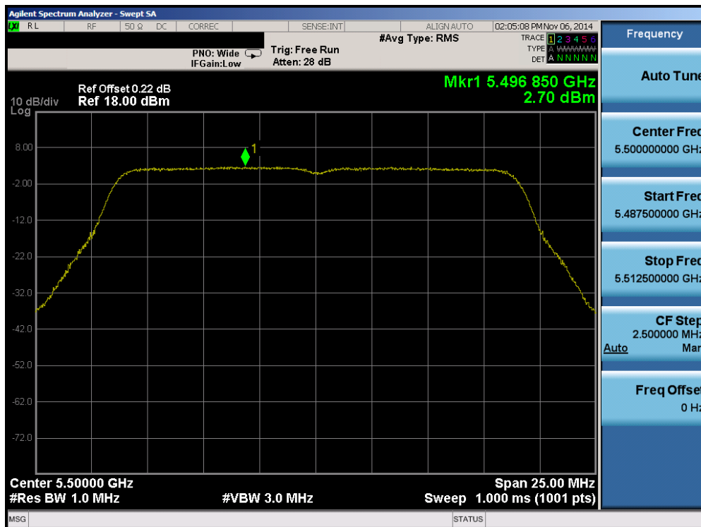
Plot 6-64. Peak Power Spectral Density Plot (20MHz BW 802.11n (UNII Band 2C) – Ch. 100)
