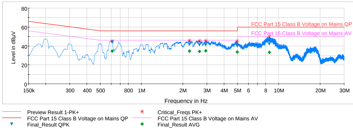
Plot 6-121. Line Conducted Plot with 802.11a UNII Band 2A (N)
