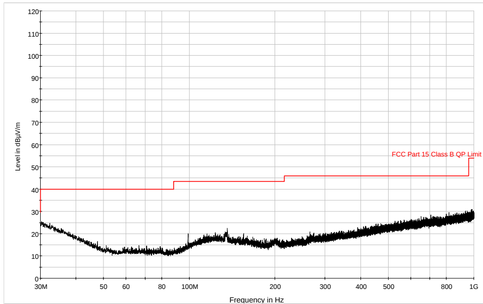
Plot 6-89. Radiated Spurious Plot below 1GHz (802.11a – Band 2C, Ch. 100 Ant. Pol. H)
