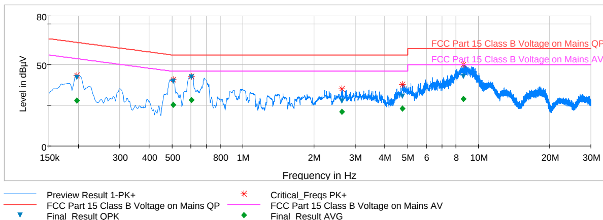
Plot 6-120. Line Conducted Plot with 802.11a UNII Band 2A (L1)
