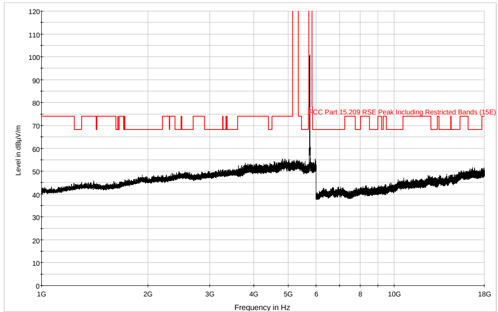
Plot 6-94. Radiated Spurious Plot above 1GHz (802.11a – Band 3, Ch. 149 Ant. Pol. H)
