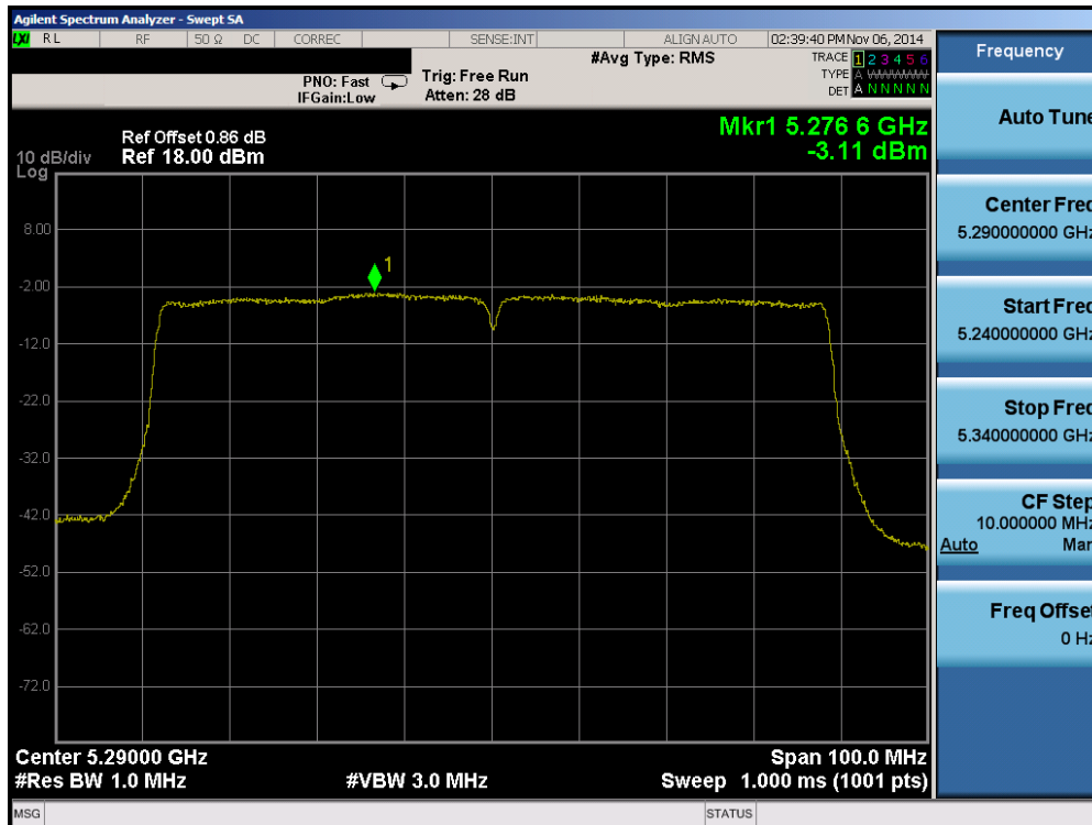
Plot 6-60. Peak Power Spectral Density Plot (80MHz BW 802.11ac (UNII Band 2A) – Ch. 58)
