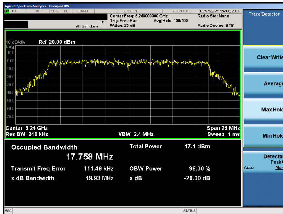
Plot 6-31. 20dB Bandwidth Plot (20MHz BW 802.11n (UNII Band 1) – Ch. 48)
