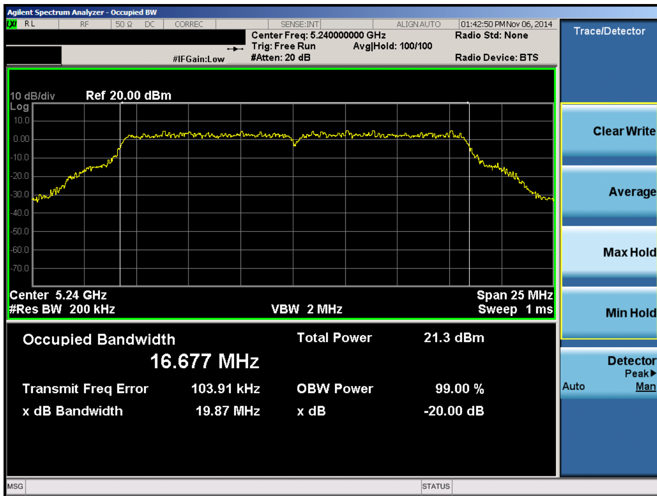
Plot 6-30. 20dB Bandwidth Plot (20MHz BW 802.11a (UNII Band 1) – Ch. 48)
