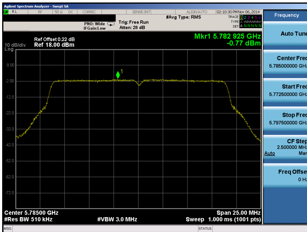
Plot 6-76. Peak Power Spectral Density Plot (20MHz BW 802.11n (UNII Band 3) – Ch. 157)
