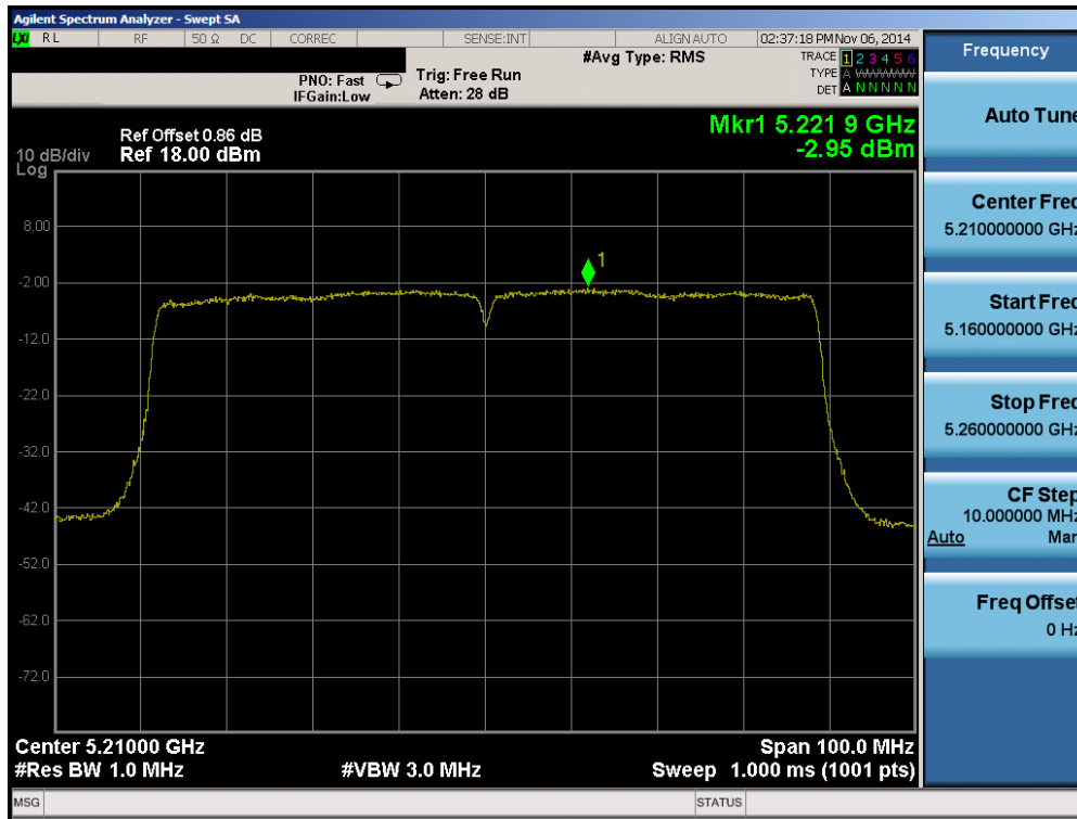
Plot 6-51. Peak Power Spectral Density Plot (80MHz BW 802.11ac (UNII Band 1) – Ch. 42)
