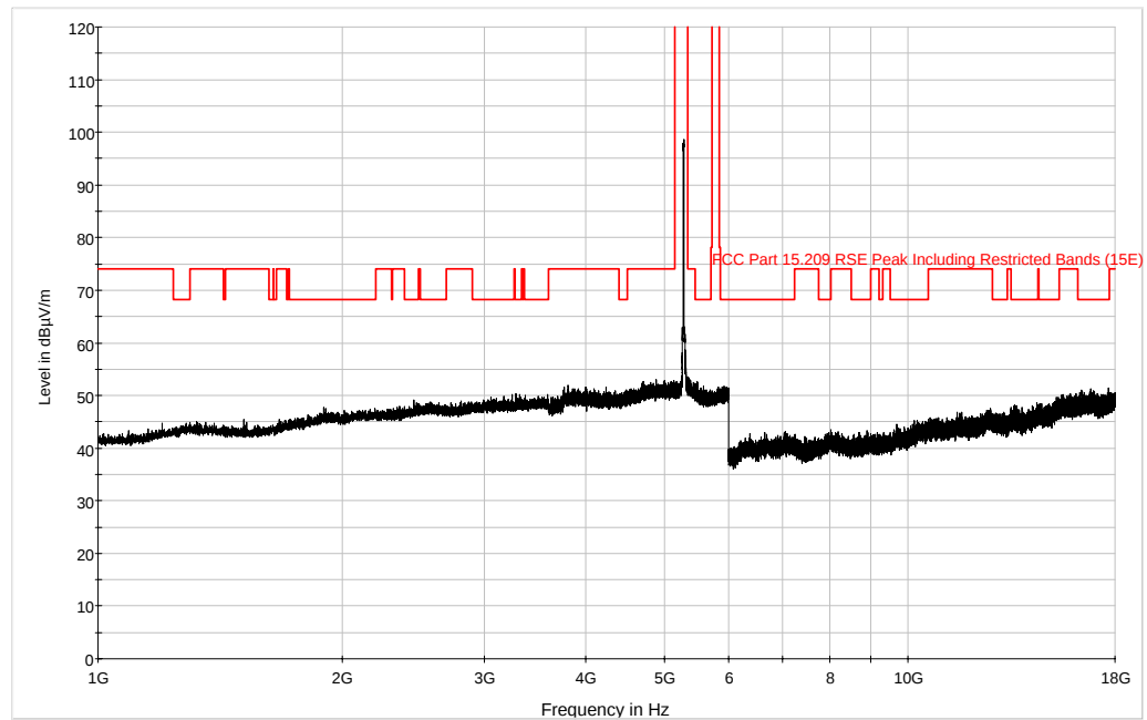
Plot 6-86. Radiated Spurious Plot above 1GHz (802.11a – Band 2A, Ch. 52 Ant. Pol. H)
