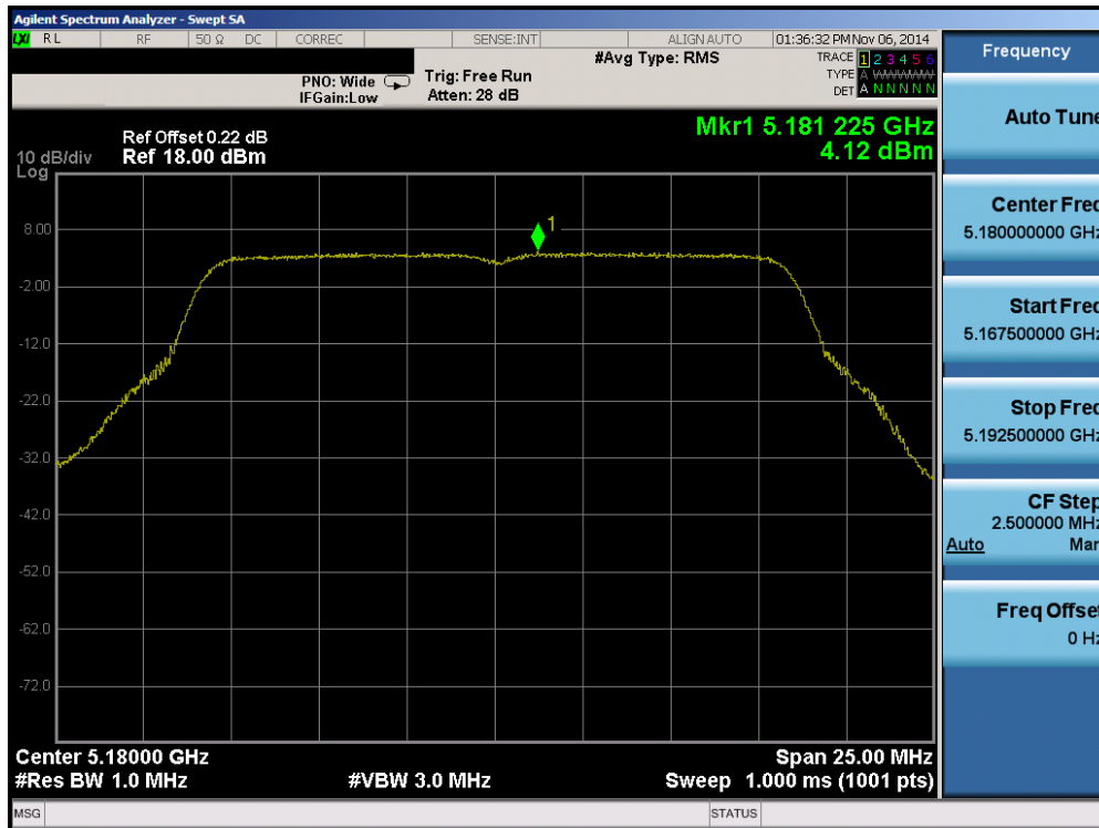
Plot 6-43. Peak Power Spectral Density Plot (802.11a (UNII Band 1) – Ch. 36)
