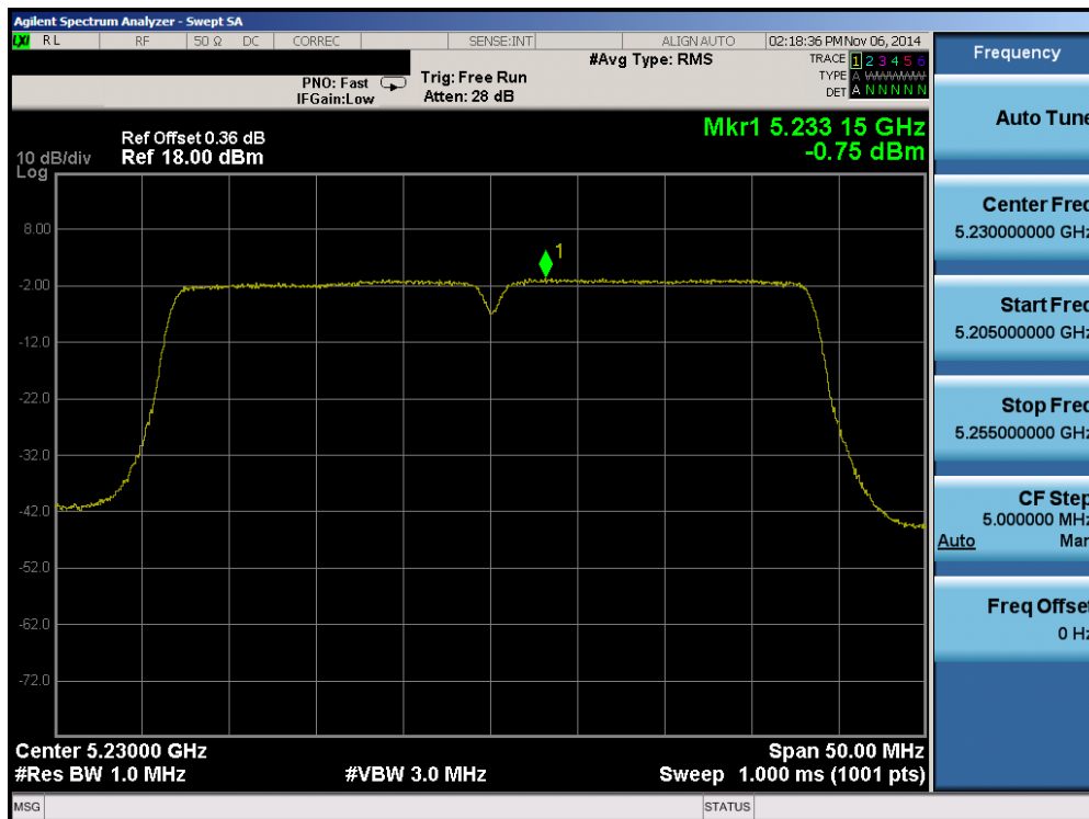
Plot 6-50. Peak Power Spectral Density Plot (40MHz BW 802.11n (UNII Band 1) – Ch. 46)
