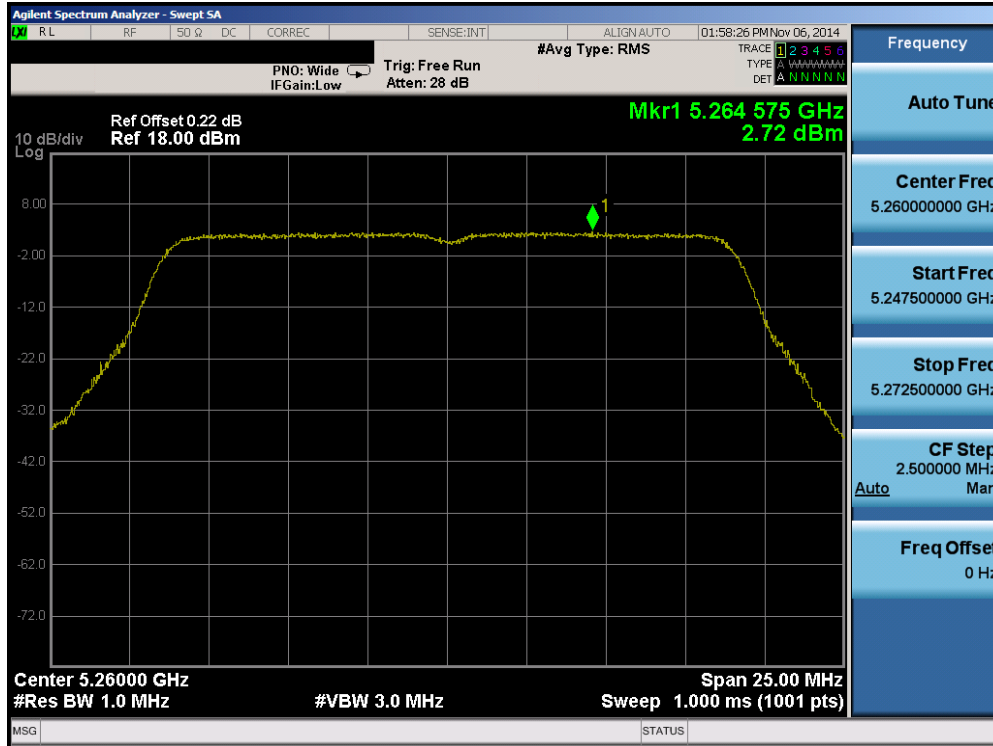
Plot 6-55. Peak Power Spectral Density Plot (20MHz BW 802.11n (UNII Band 2A) – Ch. 52)
