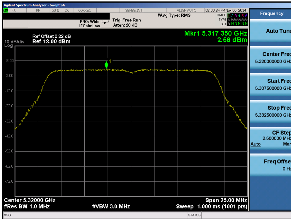
Plot 6-57. Peak Power Spectral Density Plot (20MHz BW 802.11n (UNII Band 2A) – Ch. 64)
