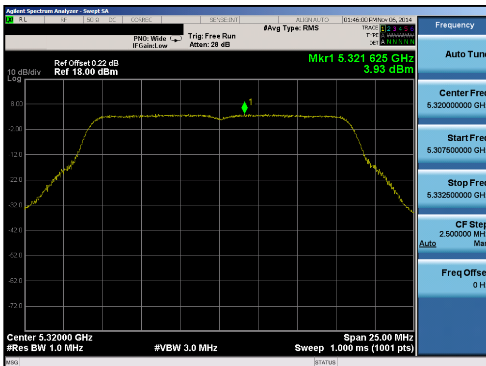
Plot 6-54. Peak Power Spectral Density Plot (802.11a (UNII Band 2A) – Ch. 64)
