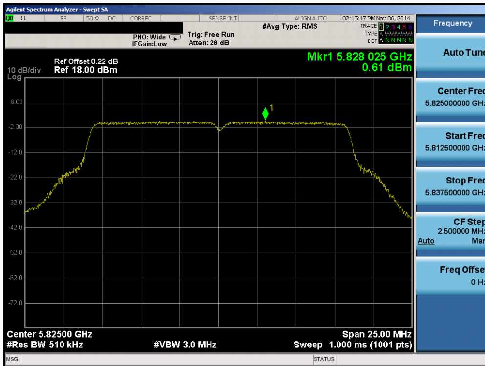
Plot 6-74. Peak Power Spectral Density Plot (802.11a (UNII Band 3) – Ch. 165)
