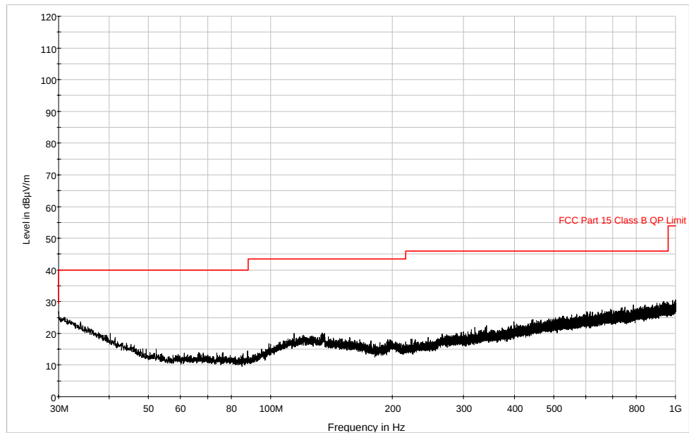
Plot 6-81. Radiated Spurious Plot below 1GHz (802.11a – Band 1, Ch. 36 Ant. Pol. H)
