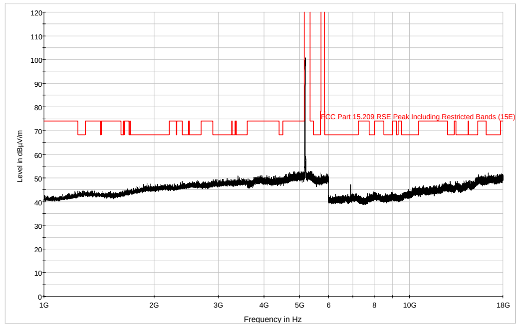
Plot 6-84. Radiated Spurious Plot above 1GHz (802.11a – Band 1, Ch. 36 Ant. Pol. V)
