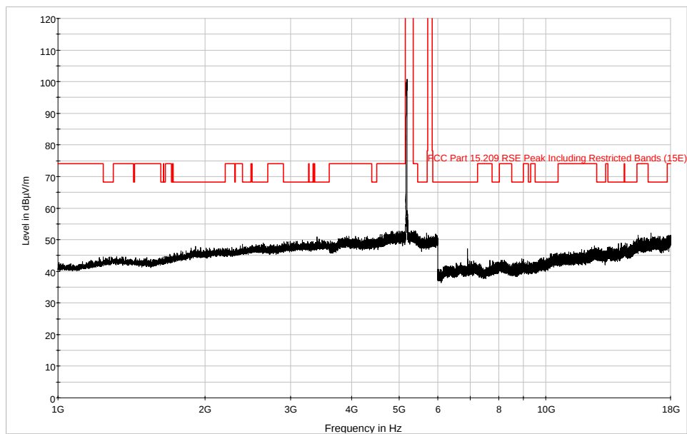
Plot 6-82. Radiated Spurious Plot above 1GHz (802.11a – Band 1, Ch. 36 Ant. Pol. H)
