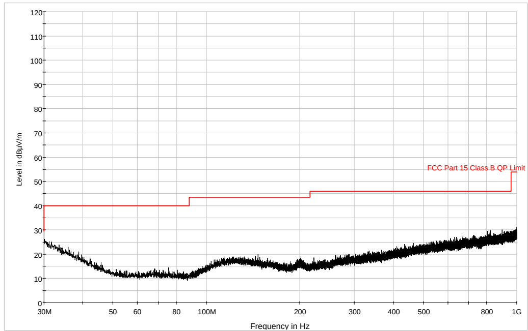
Plot 6-83. Radiated Spurious Plot below 1GHz (802.11a – Band 1, Ch. 36 Ant. Pol. V)
