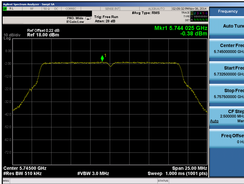
Plot 6-75. Peak Power Spectral Density Plot (20MHz BW 802.11n (UNII Band 3) – Ch. 149)
