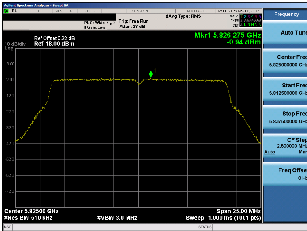
Plot 6-77. Peak Power Spectral Density Plot (20MHz BW 802.11n (UNII Band 3) – Ch. 165)
