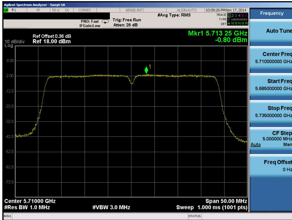
Plot 6-69. Peak Power Spectral Density Plot (40MHz BW 802.11n (UNII Band 2C) – Ch. 142)
