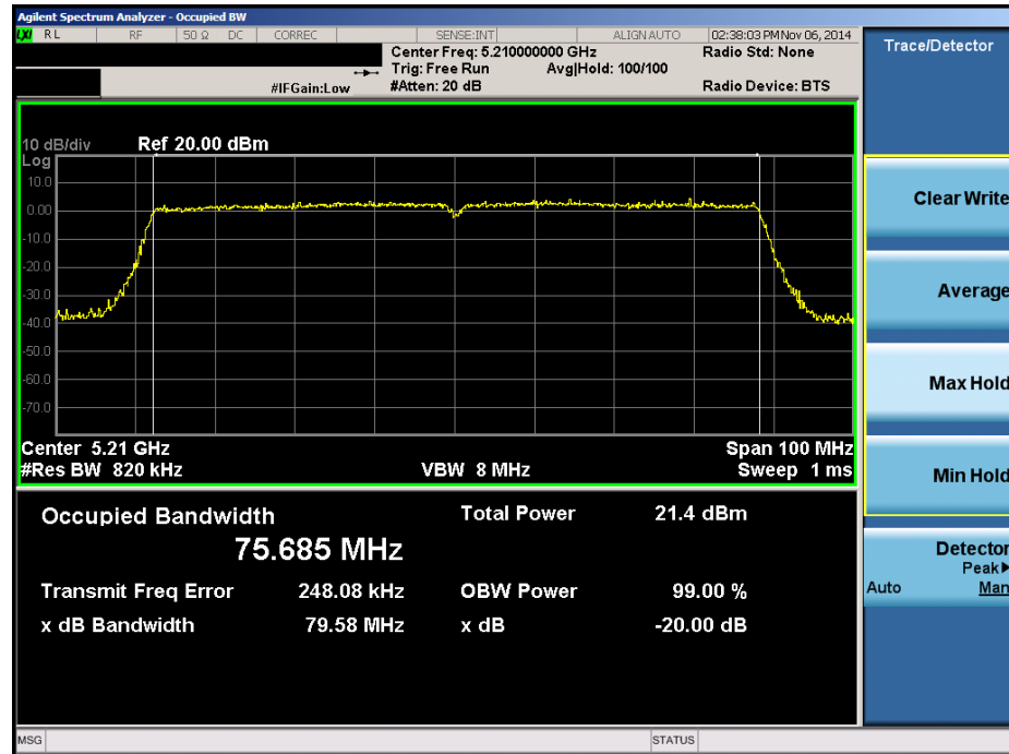
Plot 6-33. 20dB Bandwidth Plot (80MHz BW 802.11ac (UNII Band 1) – Ch. 42)
