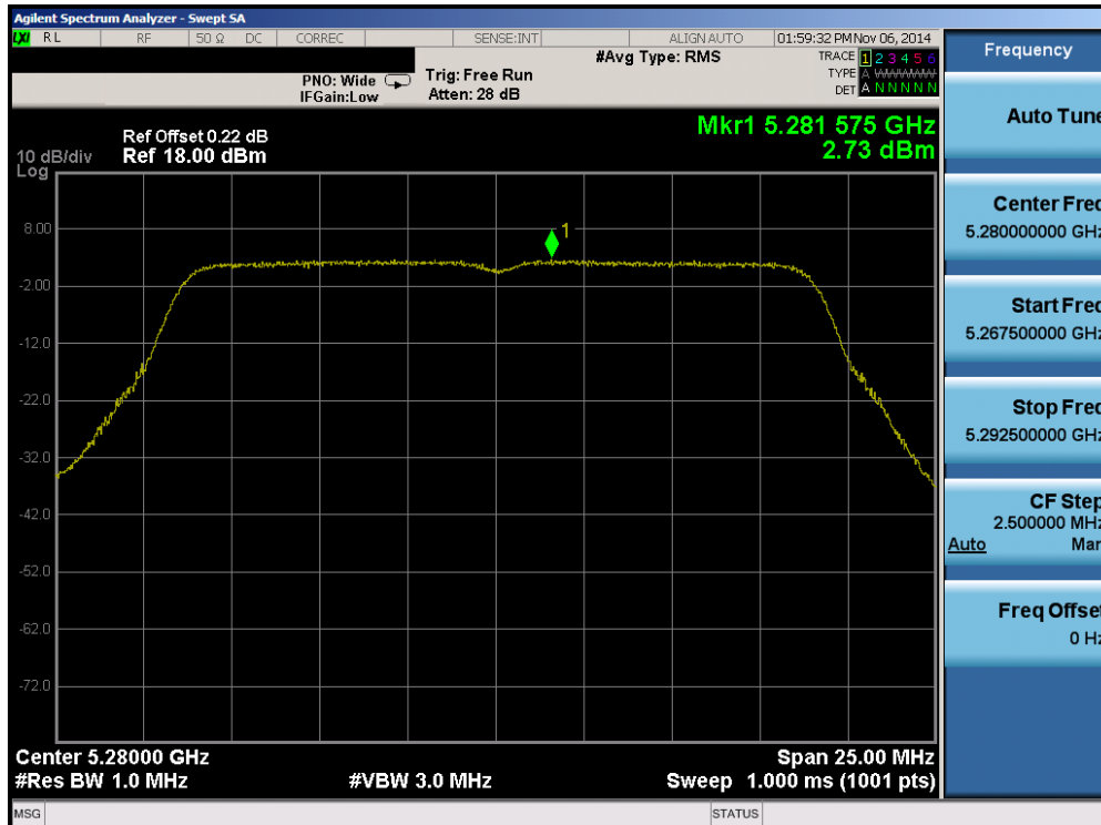
Plot 6-56. Peak Power Spectral Density Plot (20MHz BW 802.11n (UNII Band 2A) – Ch. 56)
