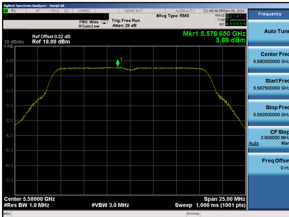
Plot 6-62. Peak Power Spectral Density Plot (802.11a (UNII Band 2C) – Ch. 116)
