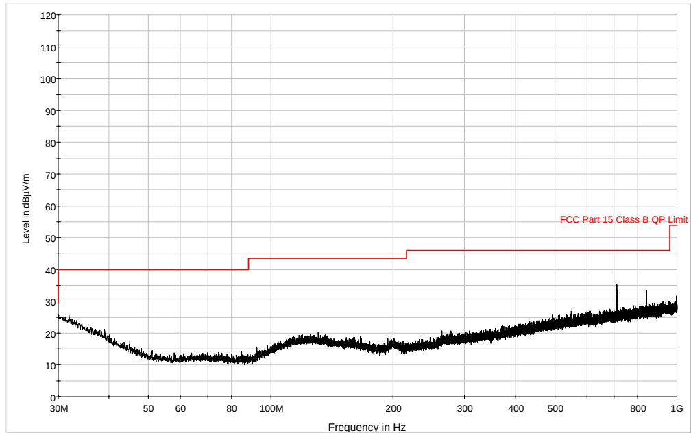
Plot 6-95. Radiated Spurious Plot below 1GHz (802.11a – Band 3, Ch. 149 Ant. Pol. V)
