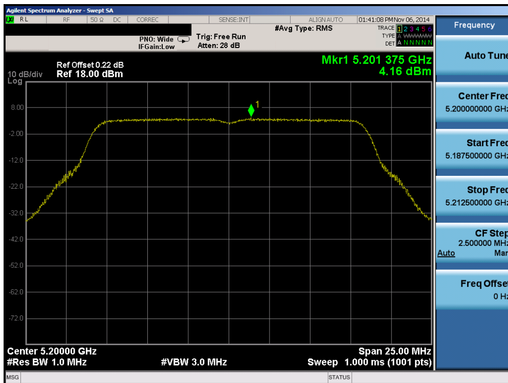
Plot 6-44. Peak Power Spectral Density Plot (802.11a (UNII Band 1) – Ch. 40)
