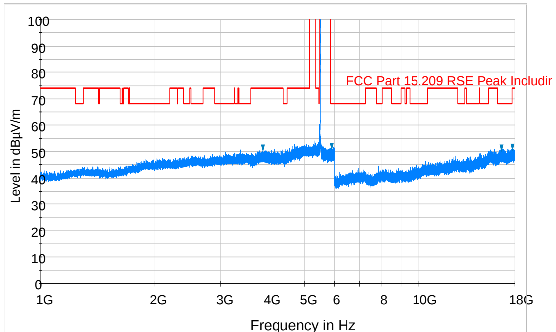
Plot 6-6. Radiated Spurious Plot above 1GHz (802.11a – U2C, Ant. Pol. V)
