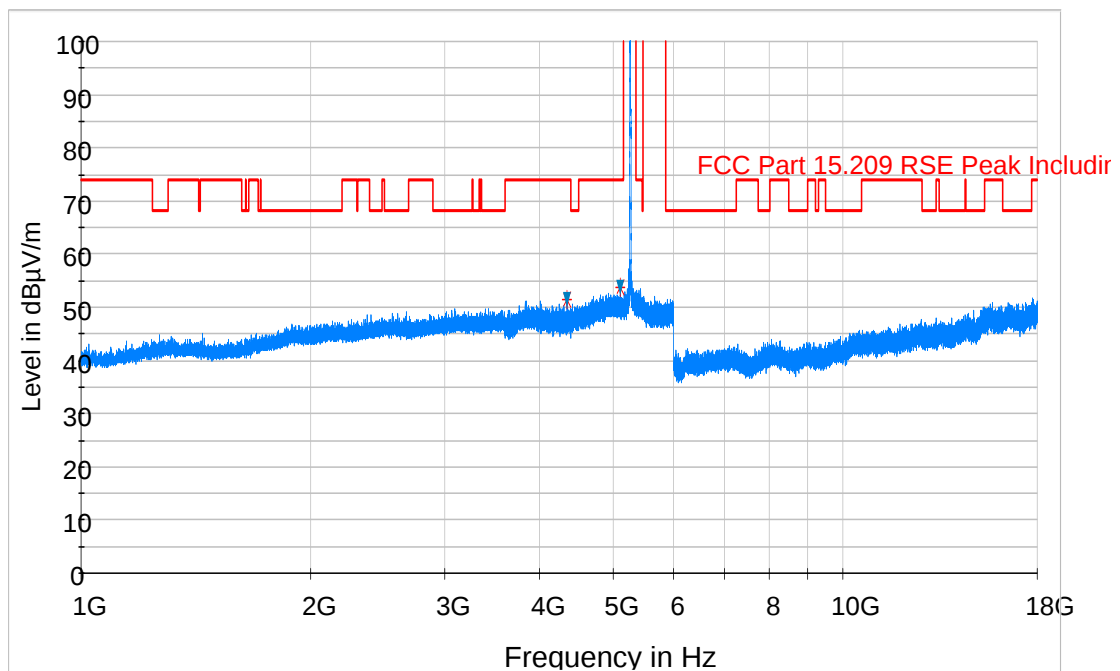
Plot 6-4. Radiated Spurious Plot above 1GHz (802.11a – U2A, Ant. Pol. V)
