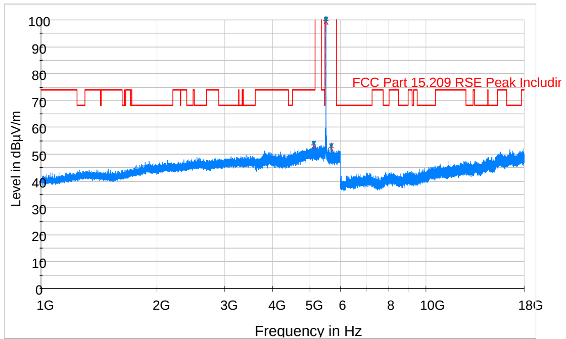
Plot 6-5. Radiated Spurious Plot above 1GHz (802.11a – U2C, Ant. Pol. H)
