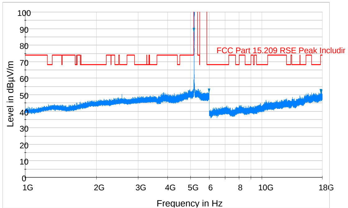
Plot 6-1. Radiated Spurious Plot above 1GHz (802.11a – U1, Ant. Pol. H)
