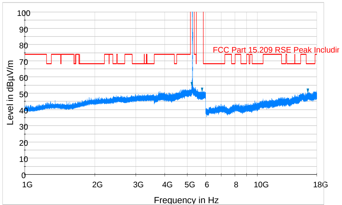
Plot 6-3. Radiated Spurious Plot above 1GHz (802.11a – U2A, Ant. Pol. H)
