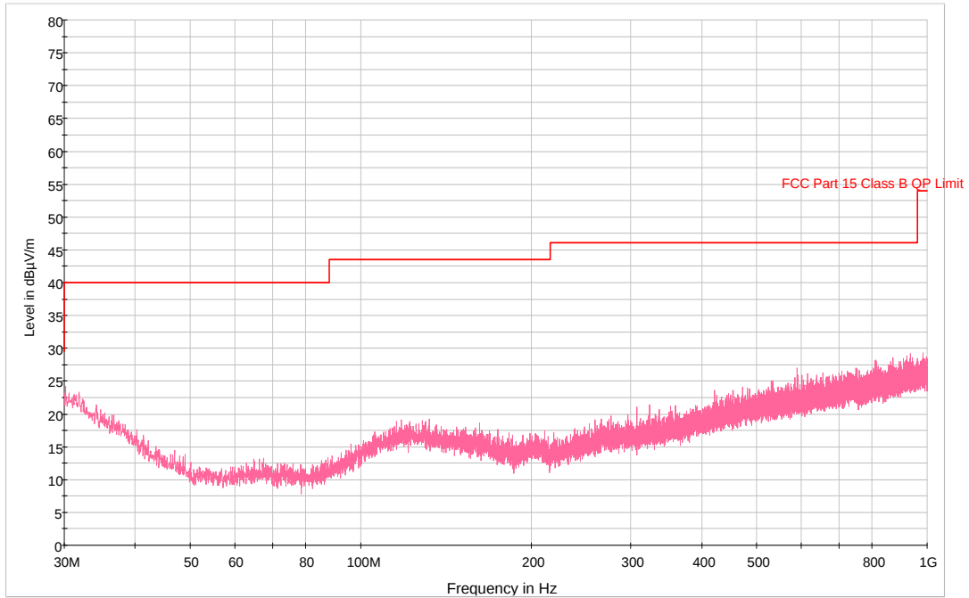
Plot 6-30. Radiated Spurious Plot below 1GHz (802.11a – U3, Ant. Pol. H)
