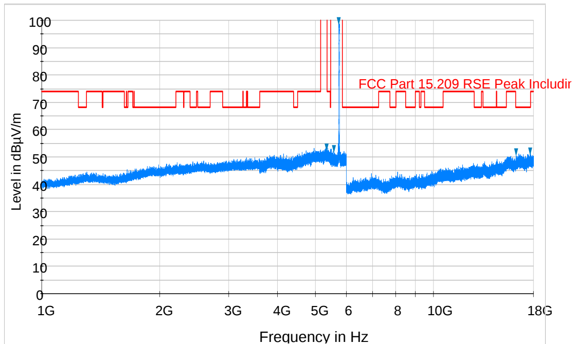
Plot 6-8. Radiated Spurious Plot above 1GHz (802.11a – U3, Ant. Pol. V)
