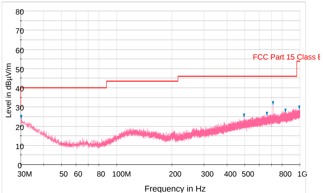
Plot 6-31. Radiated Spurious Plot below 1GHz (802.11a – U3, Ant. Pol. V)
