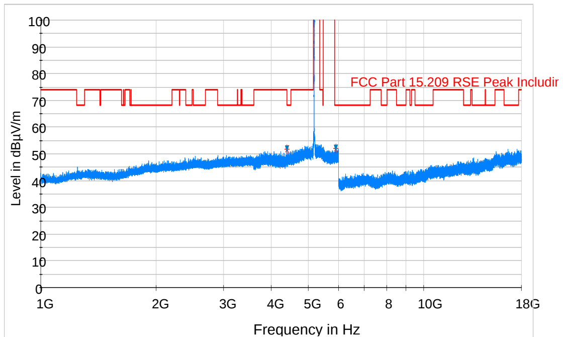
Plot 6-2. Radiated Spurious Plot above 1GHz (802.11a – U1, Ant. Pol. V)
