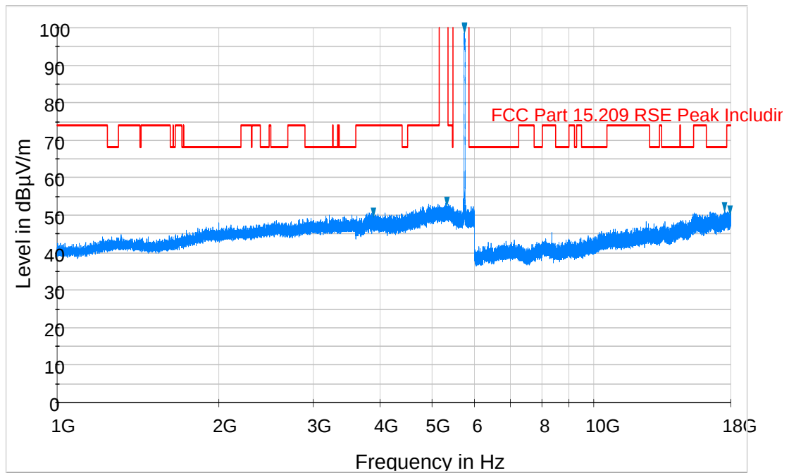
Plot 6-7. Radiated Spurious Plot above 1GHz (802.11a – U3, Ant. Pol. H)
