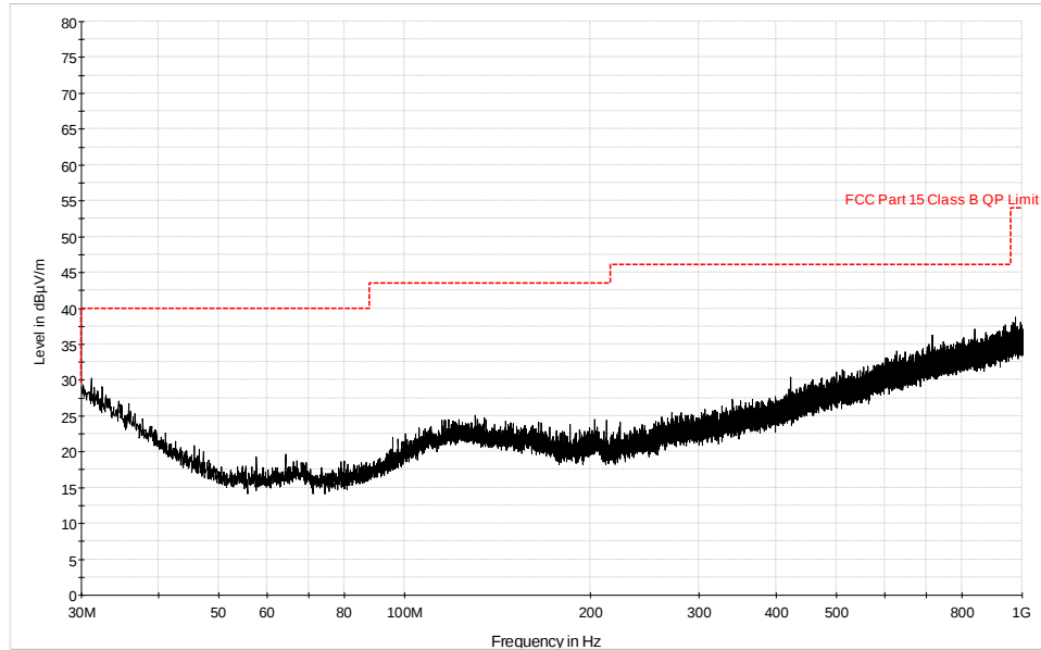
Plot 6-37. Radiated Spurious Plot below 1GHz (802.11b – Ch. 6 Ant. Pol. H)
