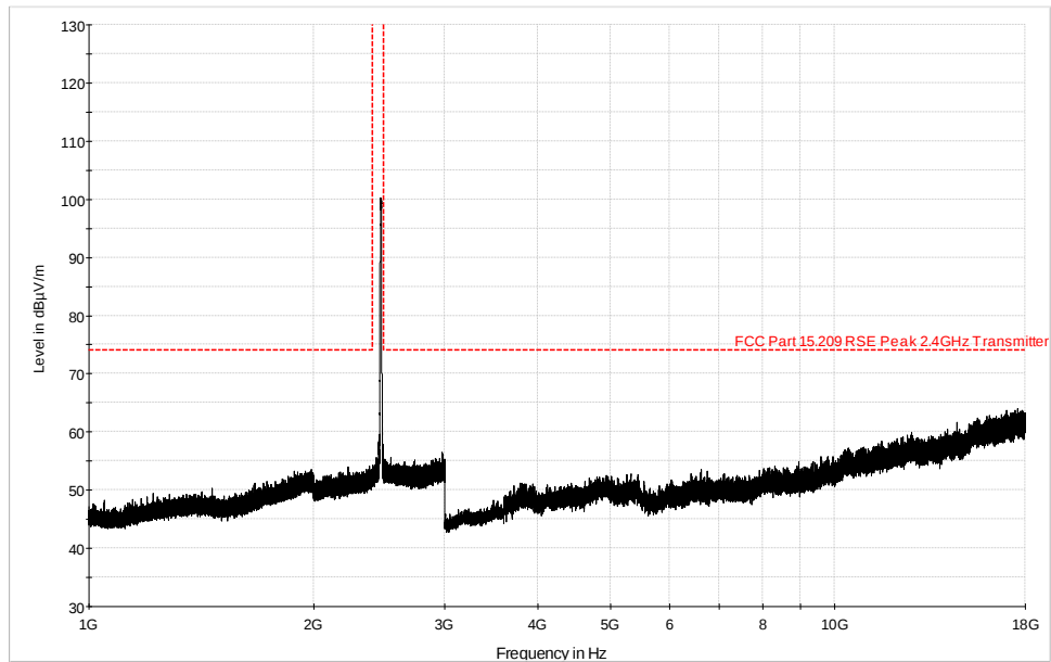
Plot 6-35. Radiated Spurious Plot above 1GHz (802.11b – Ch. 11 Ant. Pol. H)
