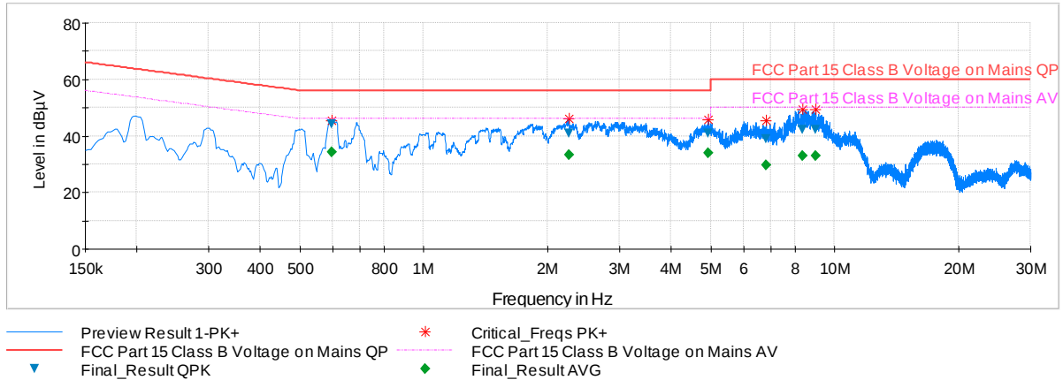
Plot 6-44. Line Conducted Plot with 802.11b (N)
