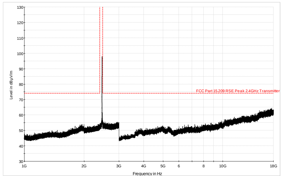
Plot 6-36. Radiated Spurious Plot above 1GHz (802.11b – Ch. 11 Ant. Pol. V)
