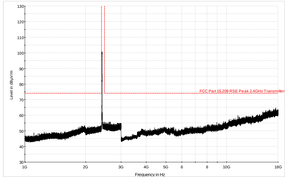
Plot 6-31. Radiated Spurious Plot above 1GHz (802.11b – Ch. 1 Ant. Pol. H)
