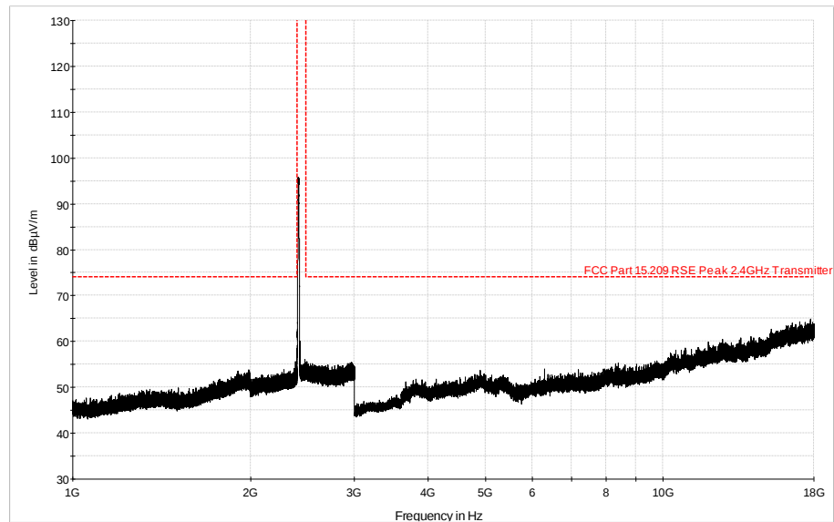
Plot 6-32. Radiated Spurious Plot above 1GHz (802.11b – Ch. 1 Ant. Pol. V)
