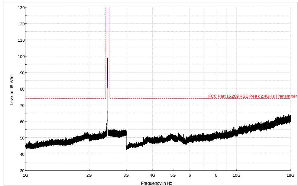
Plot 6-33. Radiated Spurious Plot above 1GHz (802.11b – Ch. 6 Ant. Pol. H)
