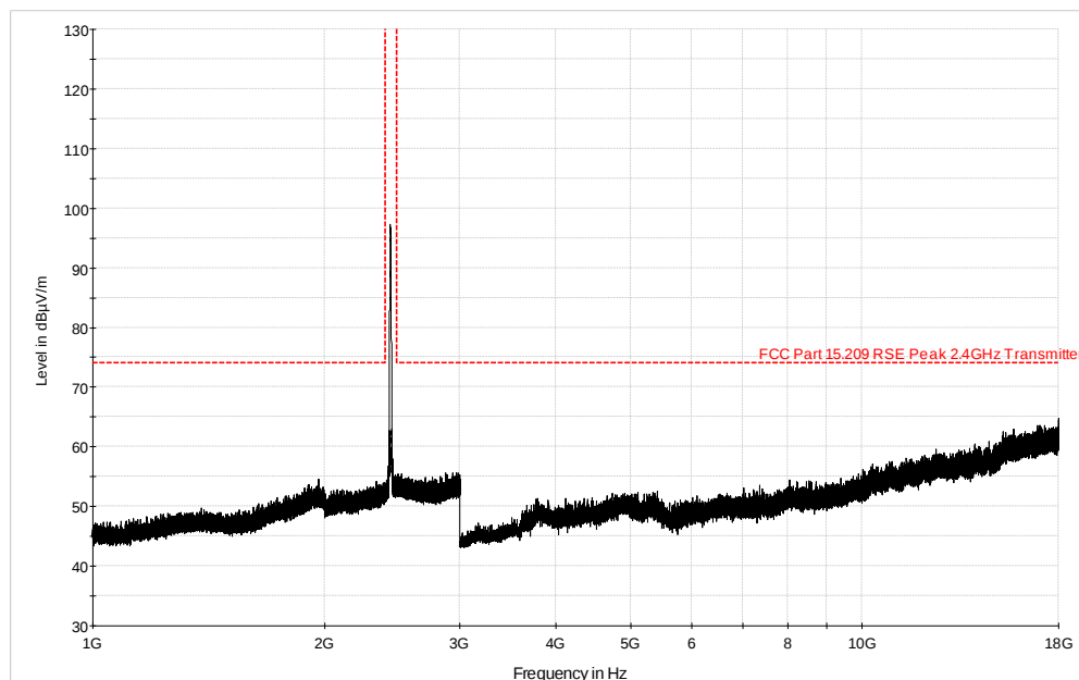
Plot 6-34. Radiated Spurious Plot above 1GHz (802.11b – Ch. 6 Ant. Pol. V)
