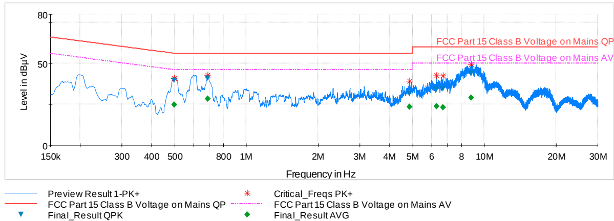
Plot 6-43. Line Conducted Plot with 802.11b (L1)
