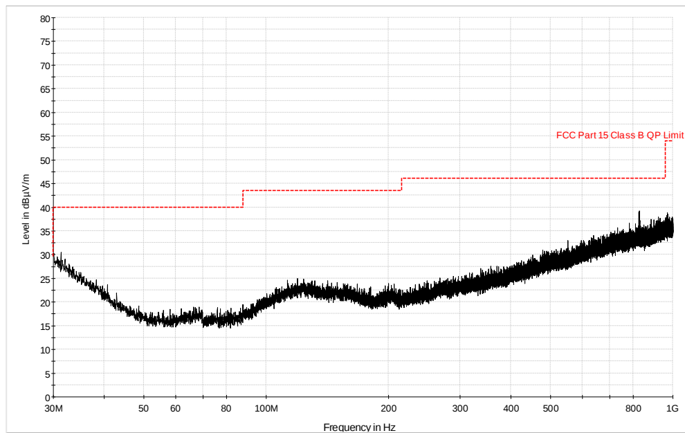
Plot 6-38. Radiated Spurious Plot below 1GHz (802.11b – Ch. 6 Ant. Pol. V)
