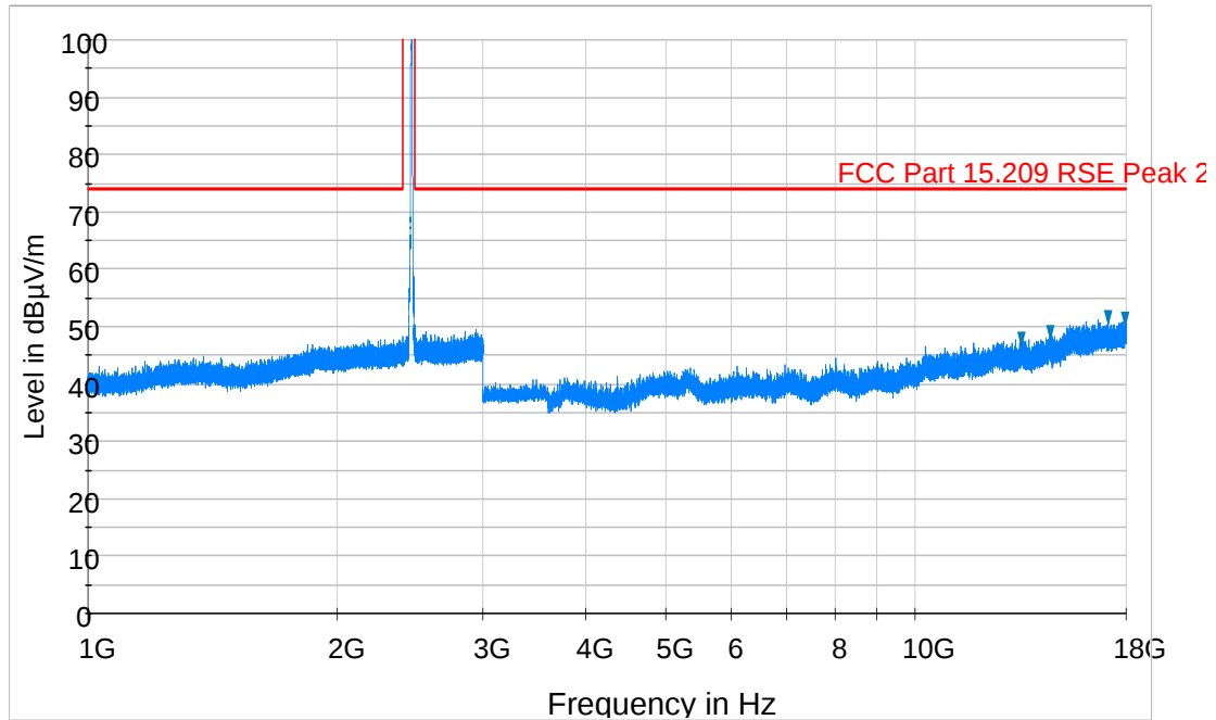
Plot 6-6. Radiated Spurious Plot above 1GHz (802.11b – Ch. 11, Ant. Pol. V)
