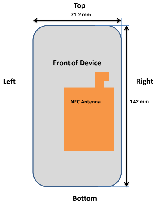
Figure F-9 NFC Antenna Locations
