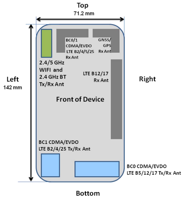
Figure F-8 DUT Antenna Locations
