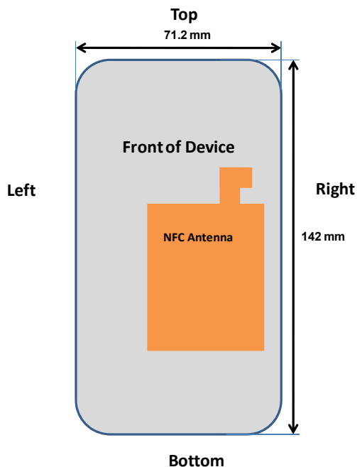
Bottom Figure F-2 NFC Antenna Locations
