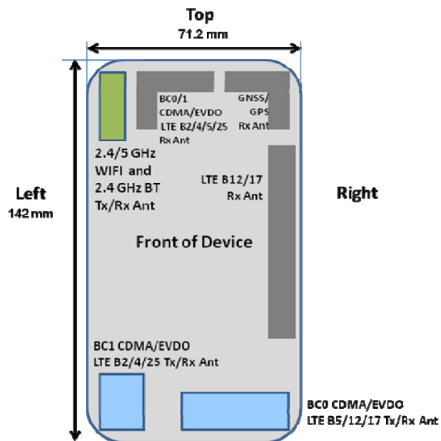
Bottom Figure F-1 DUT Antenna Locations
